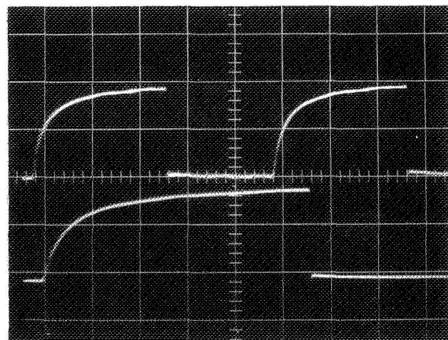
(a) SWEEP TIME (TOP) = 10 ms/cm, (BOTTOM) = 20 ms/cm ERROR VOLTAGE \approx 5 mV/cm
