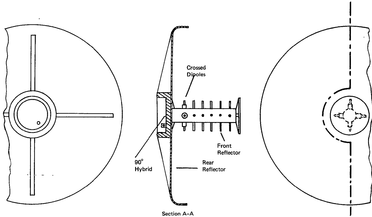
Figure II-6-5. Backfire Antenna
