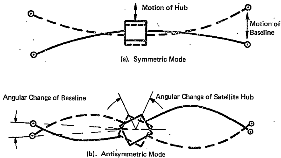
Figure II-7-3. Satellite Dynamics
