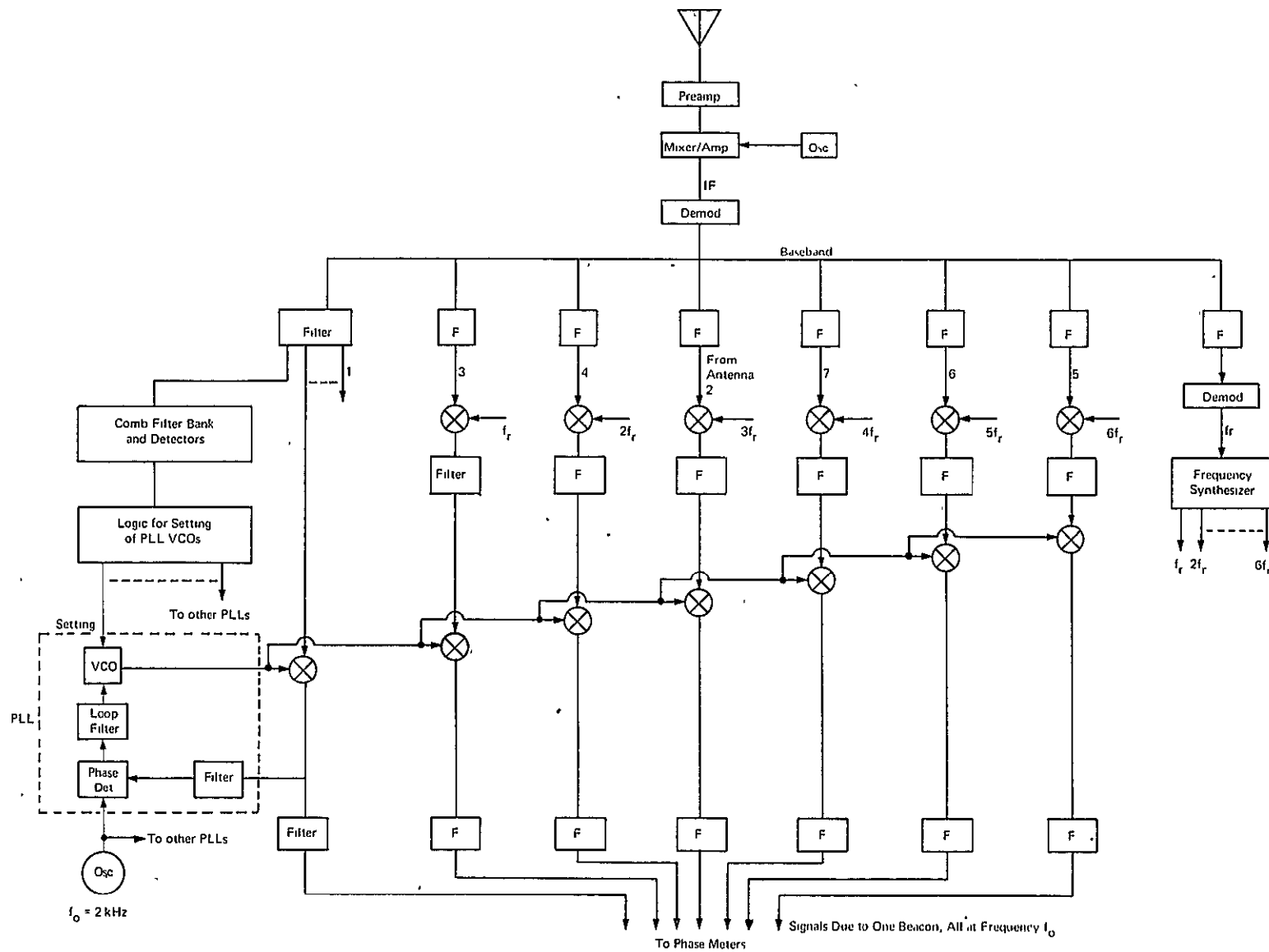
Figure II-8-8. Ground Station Receiver Configuration
