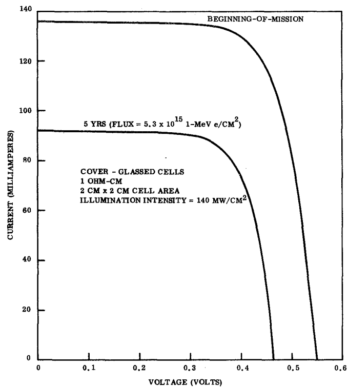
Figure 52. HVSA Solar Cell Current-Voltage Curves at +43^{\circ}\text{C} ( 316^{\circ}\text{K} )
