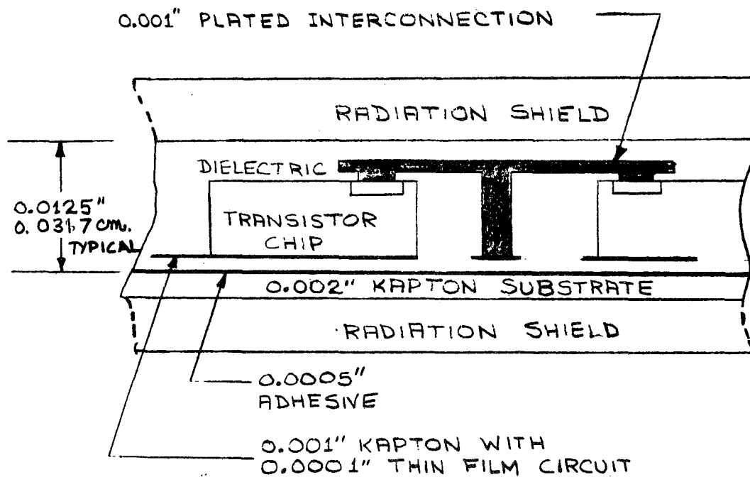
Figure 88. Thick Film Hybrid and Tape Interconnections
