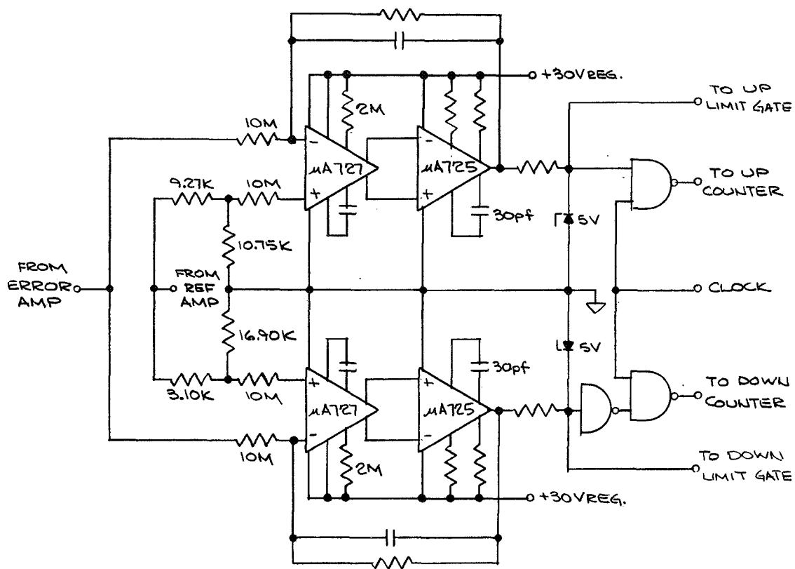
Figure 28. High and Low Detector Elements
