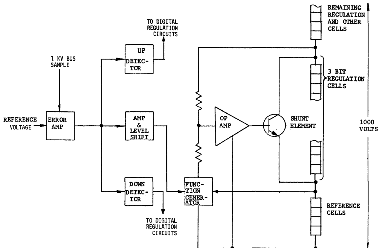
Figure 42. Three Bit Linear Regulator Block Diagram
