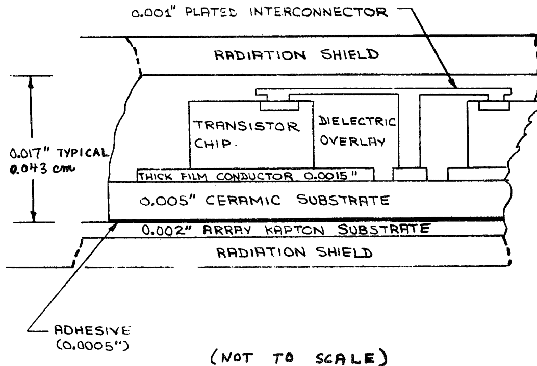
Figure 87. Thick Film Hybrid and Plated Interconnections
