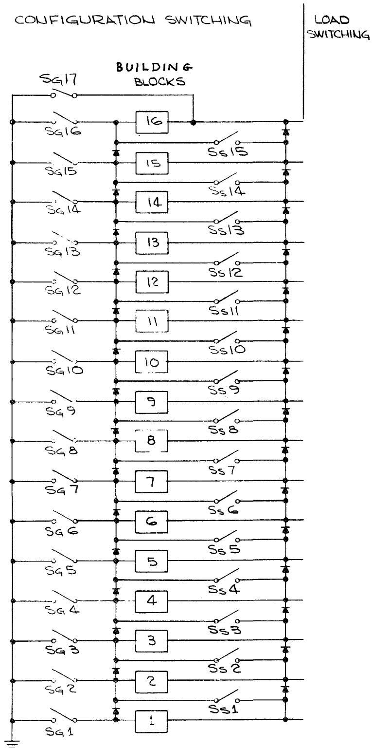
Figure 6. Switching Concept With No Output Isolation Provision
