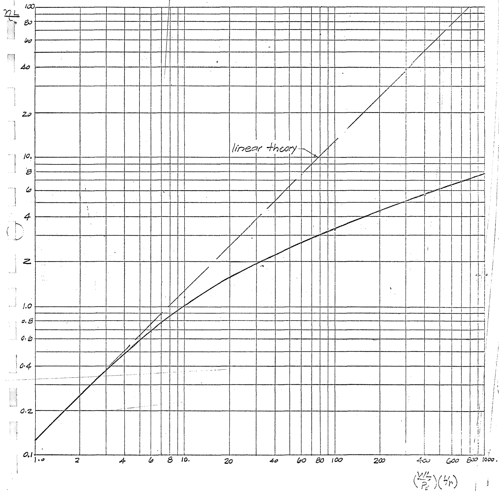
Fig. 3 Mid-Span Deflection
