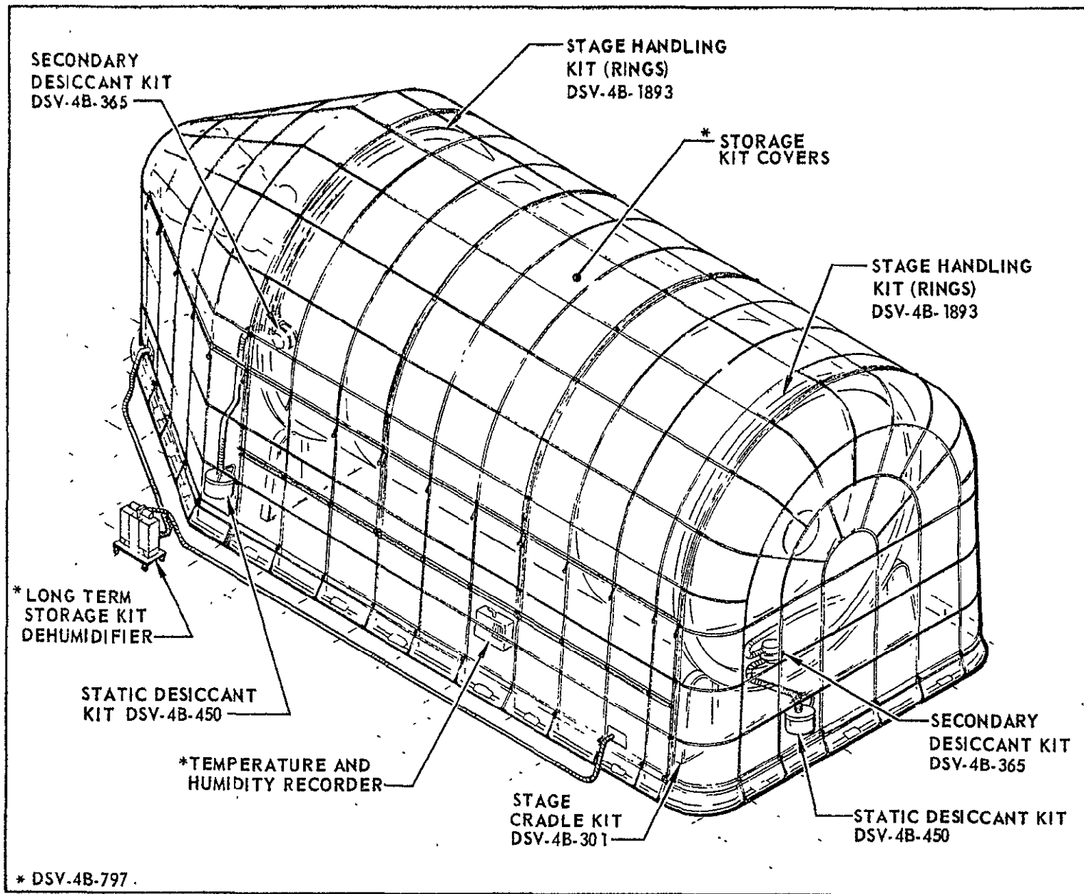
Figure 4. GSE and NDSE Requirements - Horizontal Storage STC - Typical
