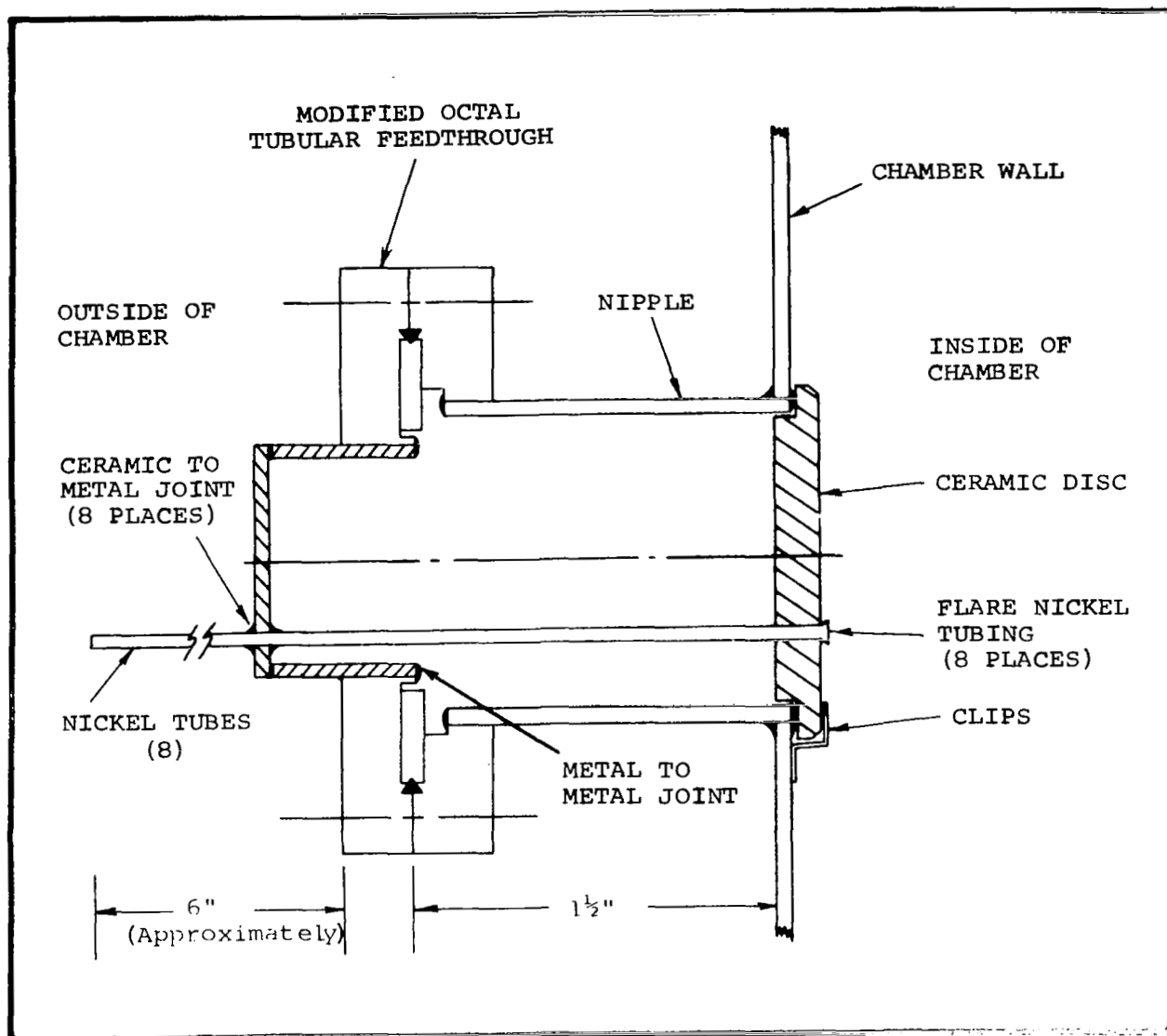
FIGURE II-3. Details of Special Thermocouple Feedthrough Flange on the Vacuum Furnace Chamber
