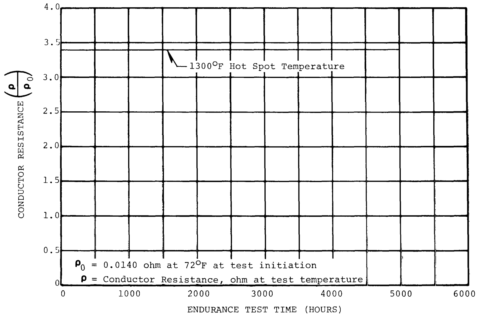
FIGURE II-27. Stator Conductor Average Resistance Versus Endurance Test Time Referenced to a 1300^\circ\text{F} Conductor Hot-Spot Temperature
