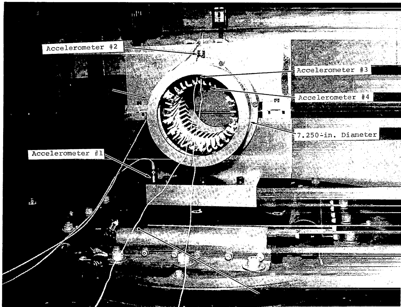
FIGURE II-21. Stator Assembly and Test Fixture Installed on Shaker for Vibration Test - 1100° F Model
