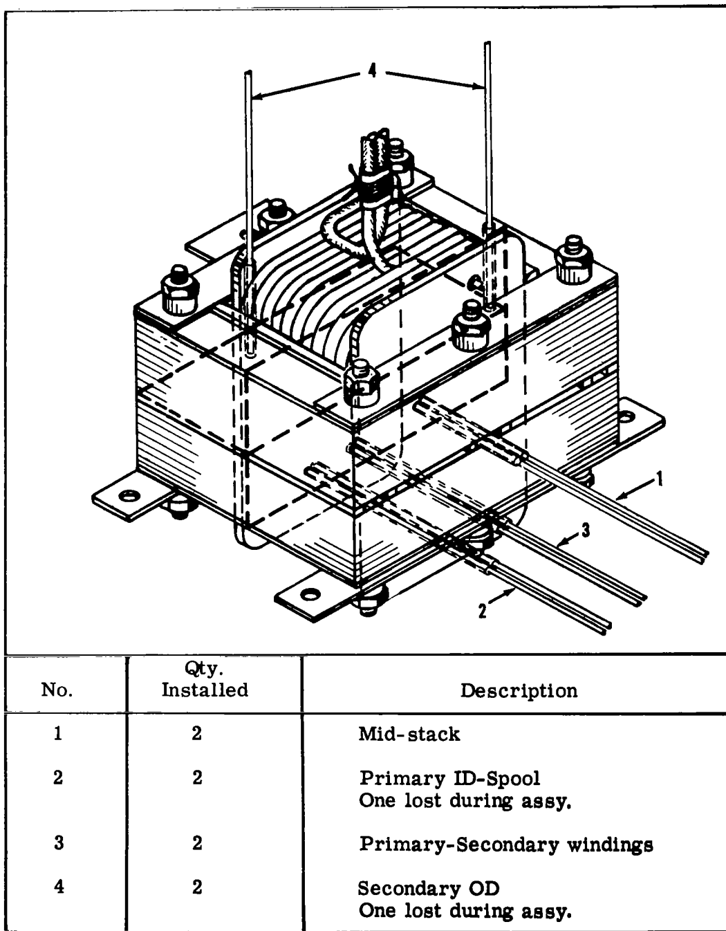
FIGURE II-36. Transformer Assembly Showing Thermocouple Locations and Junction Positions
