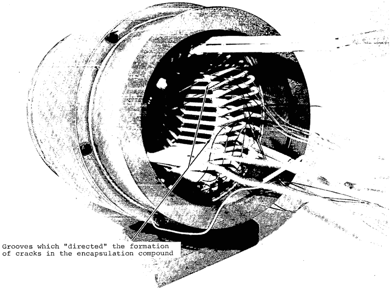
FIGURE II-20. Post-Test View of Stator Showing Stack, Windings, Slot Wedges and Encapsulating Compound - 1100° F Model
