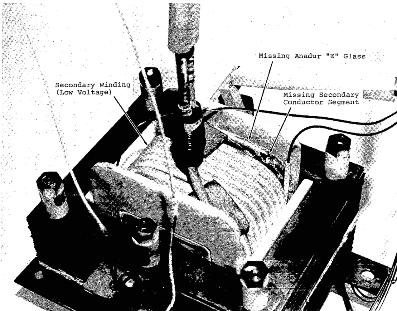
FIGURE II-43. Close-Up of Transformer Secondary Winding
