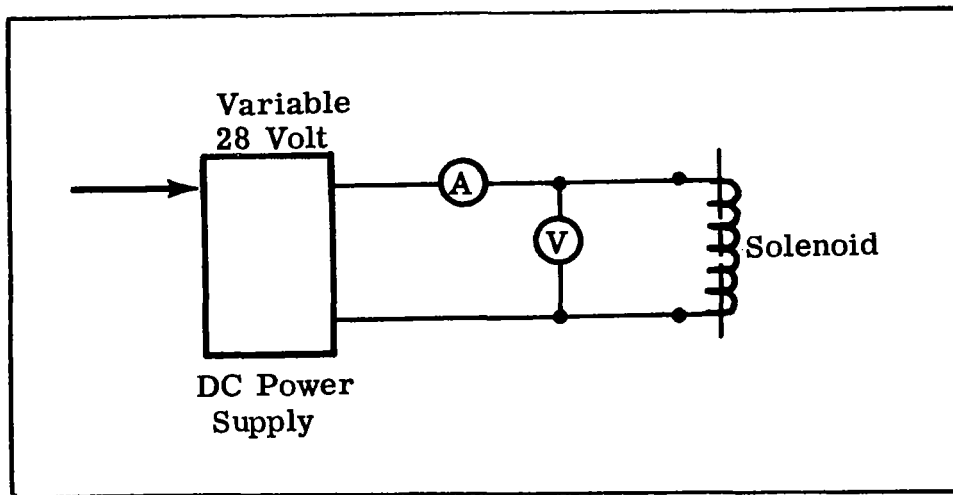
FIGURE II-56. Solenoid Circuitry
