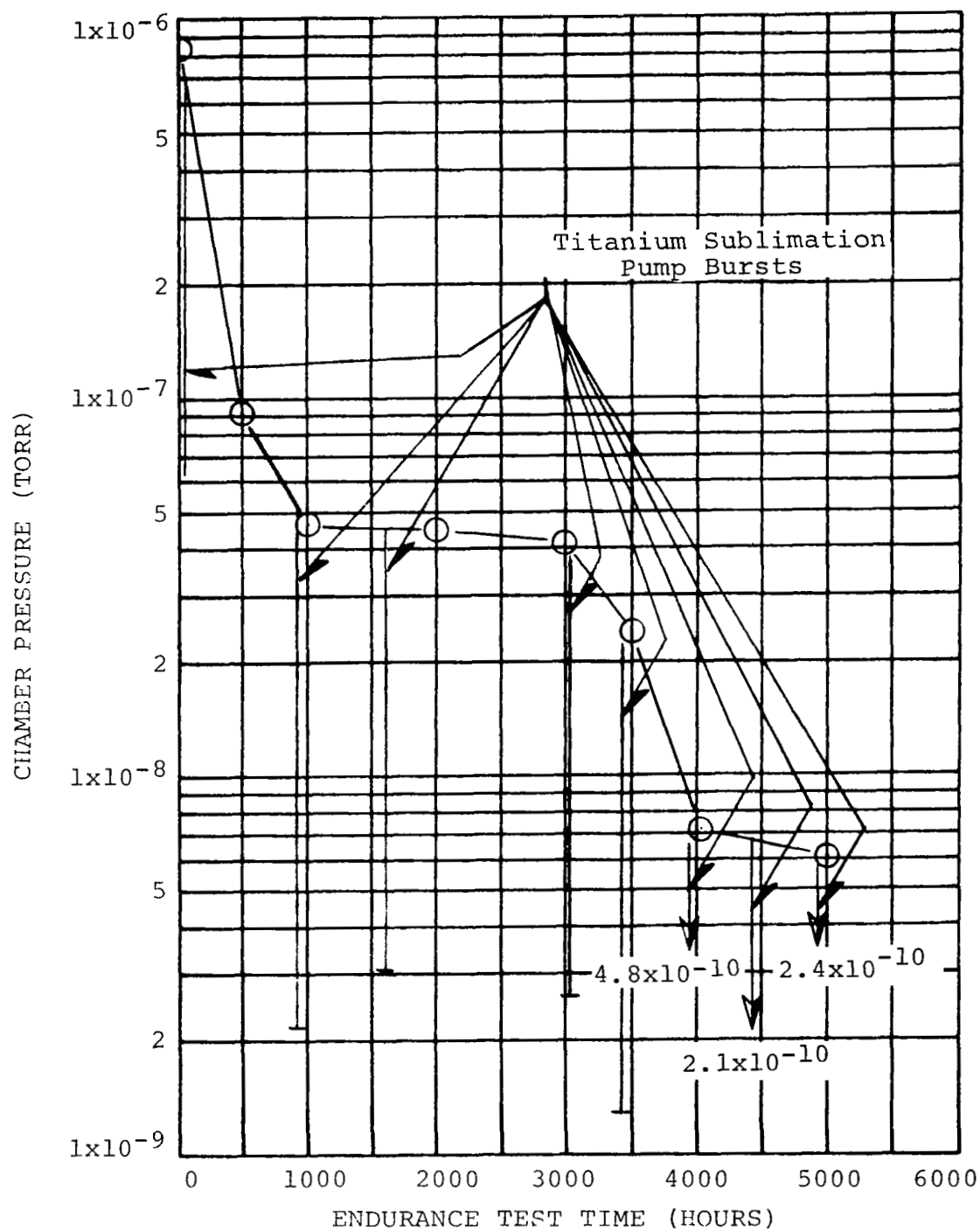
FIGURE II-37. Transformer-Solenoid Chamber Pressure Versus Endurance Test Time - 1100° F Models
