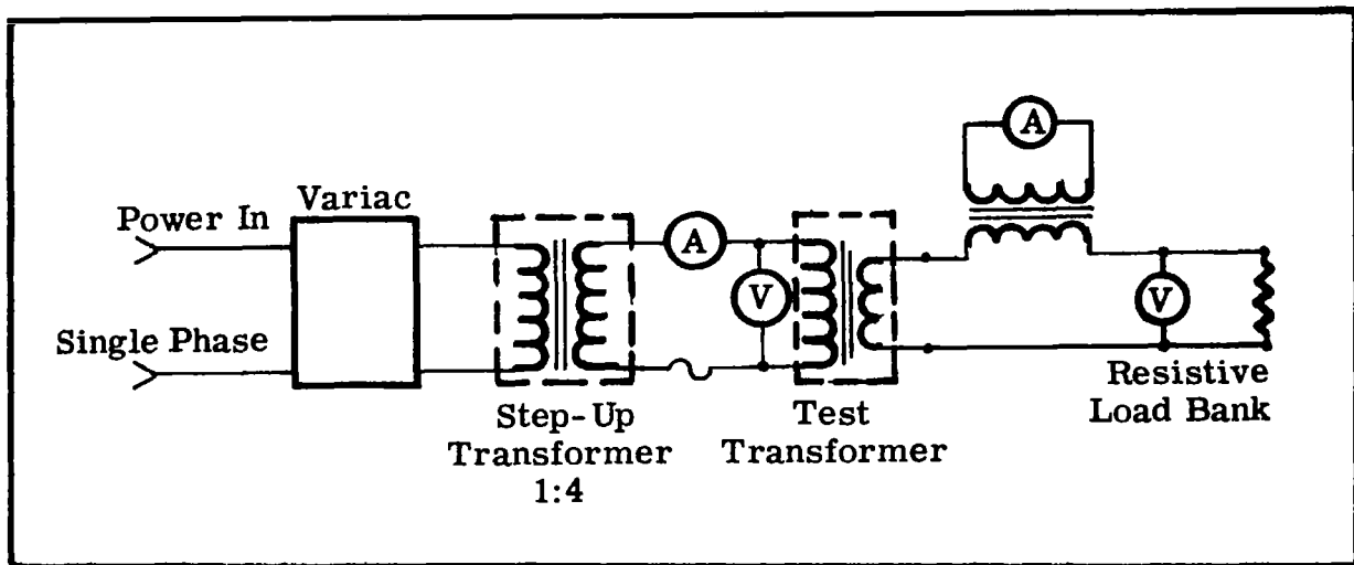
FIGURE II-35. Electrical Test Schematic for the 1 kVA Rated Transformer
