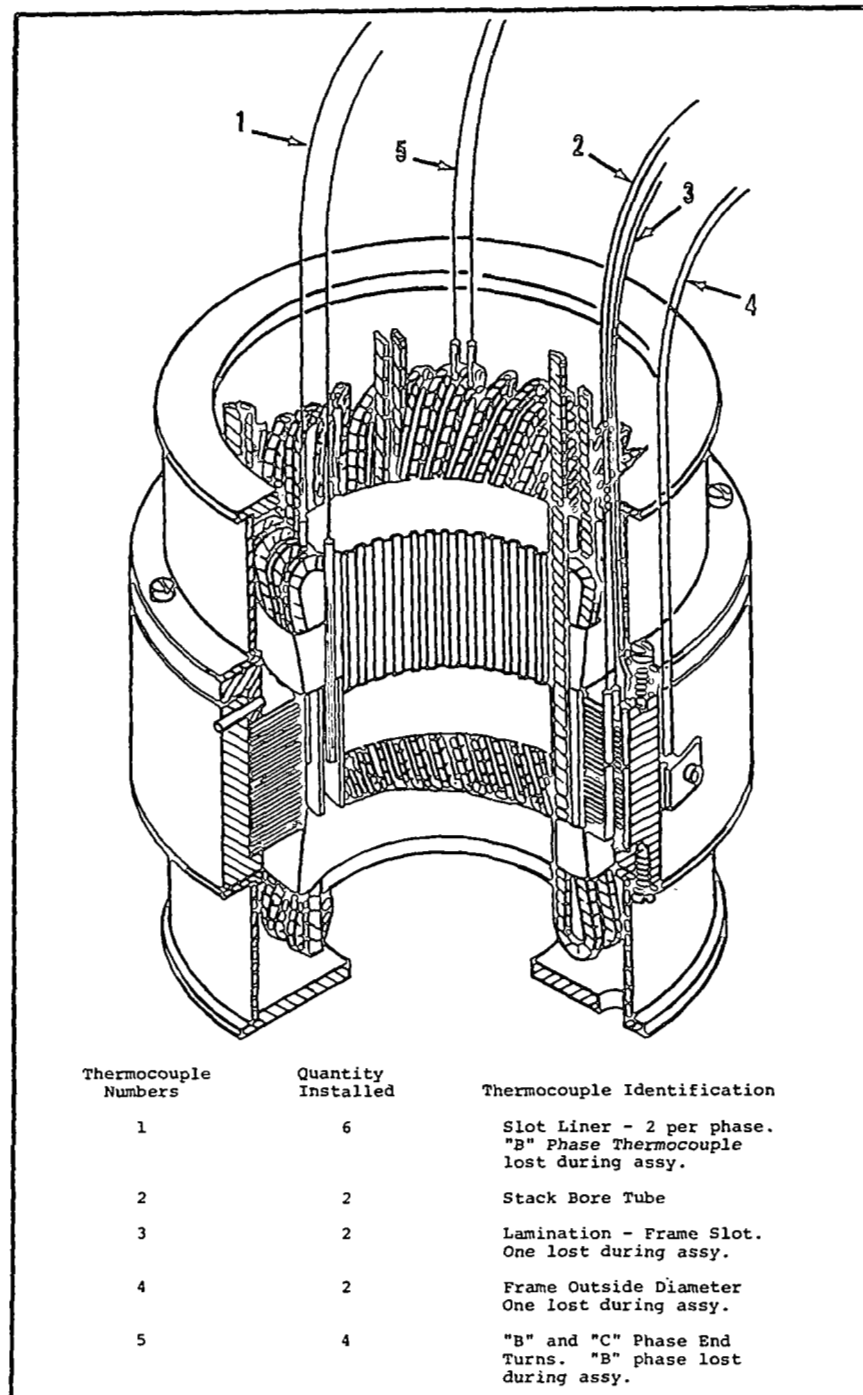
FIGURE II-13. Cutaway Drawing Showing Locations of Stator Thermocouples
