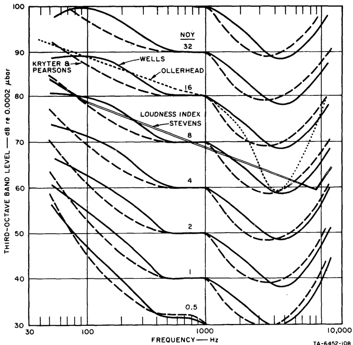
FIGURE 1 EQUAL NOISINESS CONTOURS AS FOUND BY KRYTER AND PEARSONS (14), OLLERHEAD (21) AND WELLS (30), AND EQUAL LOUDNESS INDEX CONTOUR (Stevens, 2, 29)
