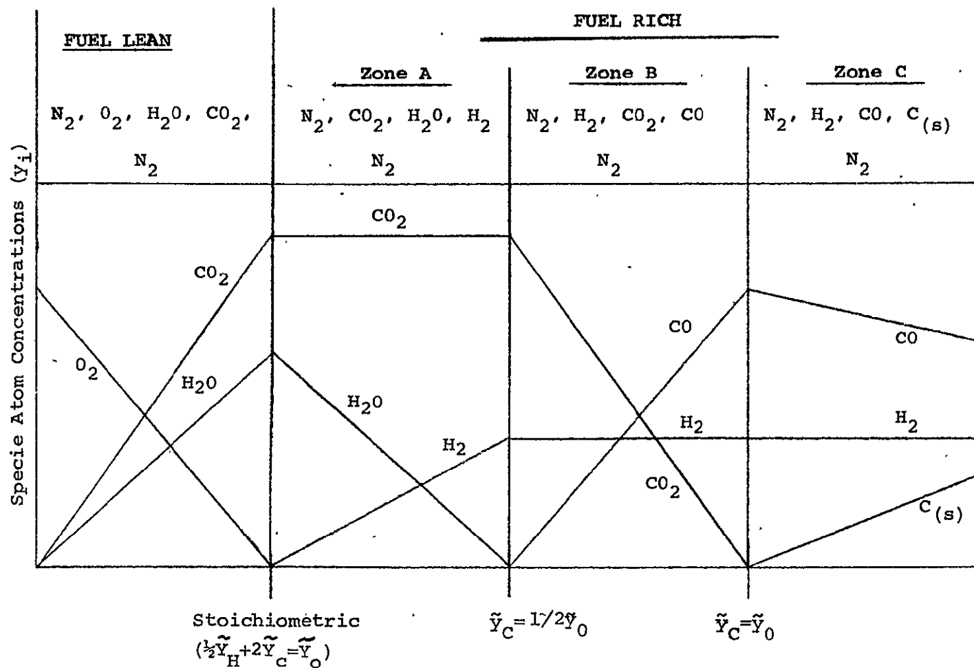
FIGURE 5. - EARLY QUASI-COMPLETE COMBUSTION OF HYDROCARBON-AIR CHEMISTRY MODEL (MODEL A)
