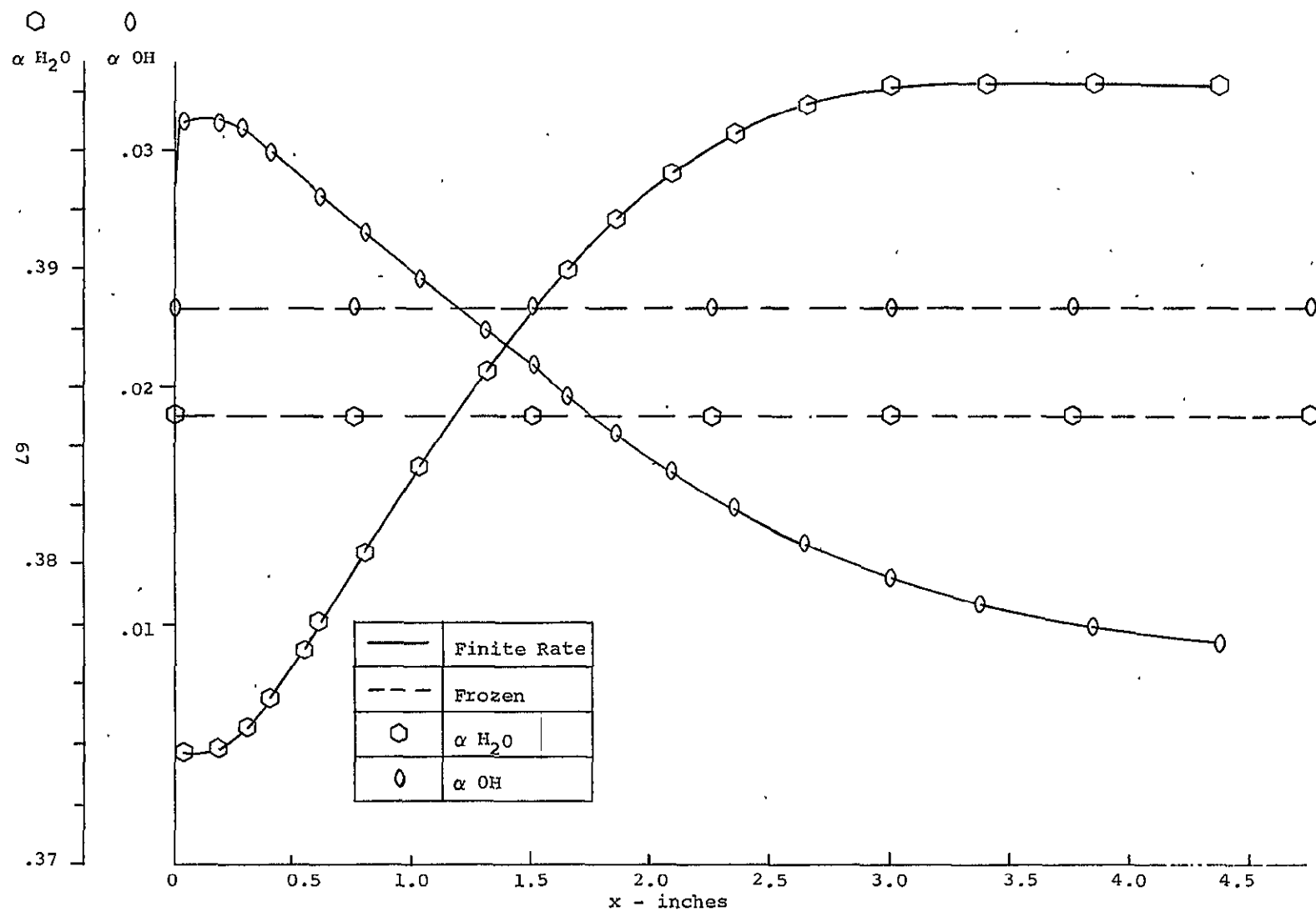
FIGURE 20b - CENTERLINE
