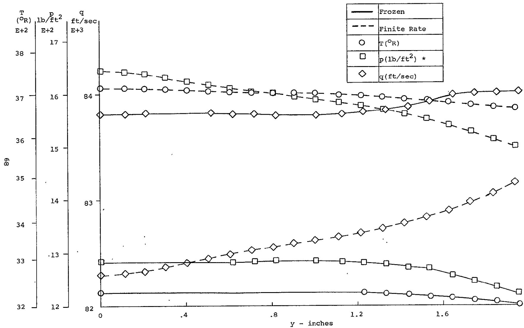
FIGURE 21 - END STATION
