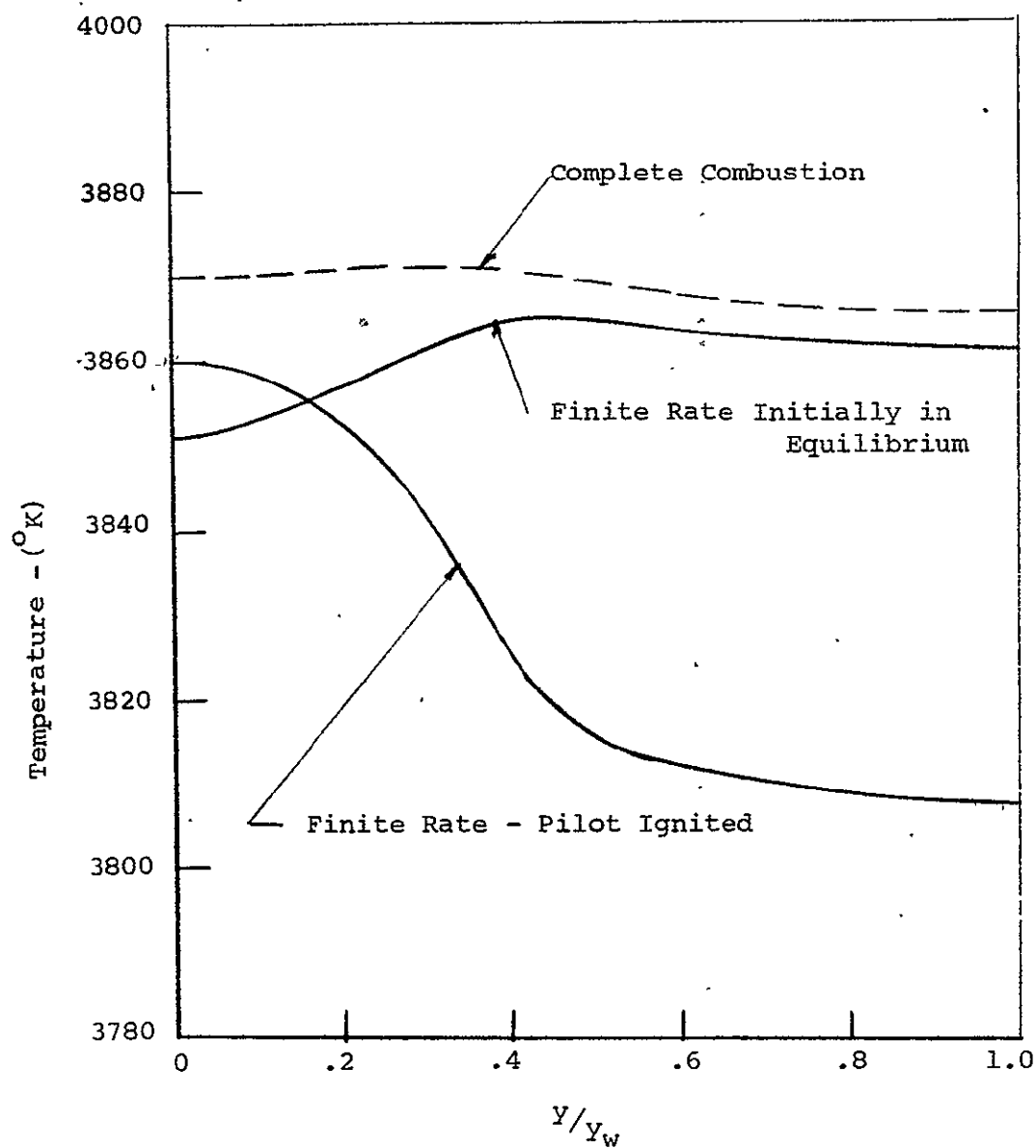
FIGURE -17- TEMPERATURE PROFILE COMPARISON
