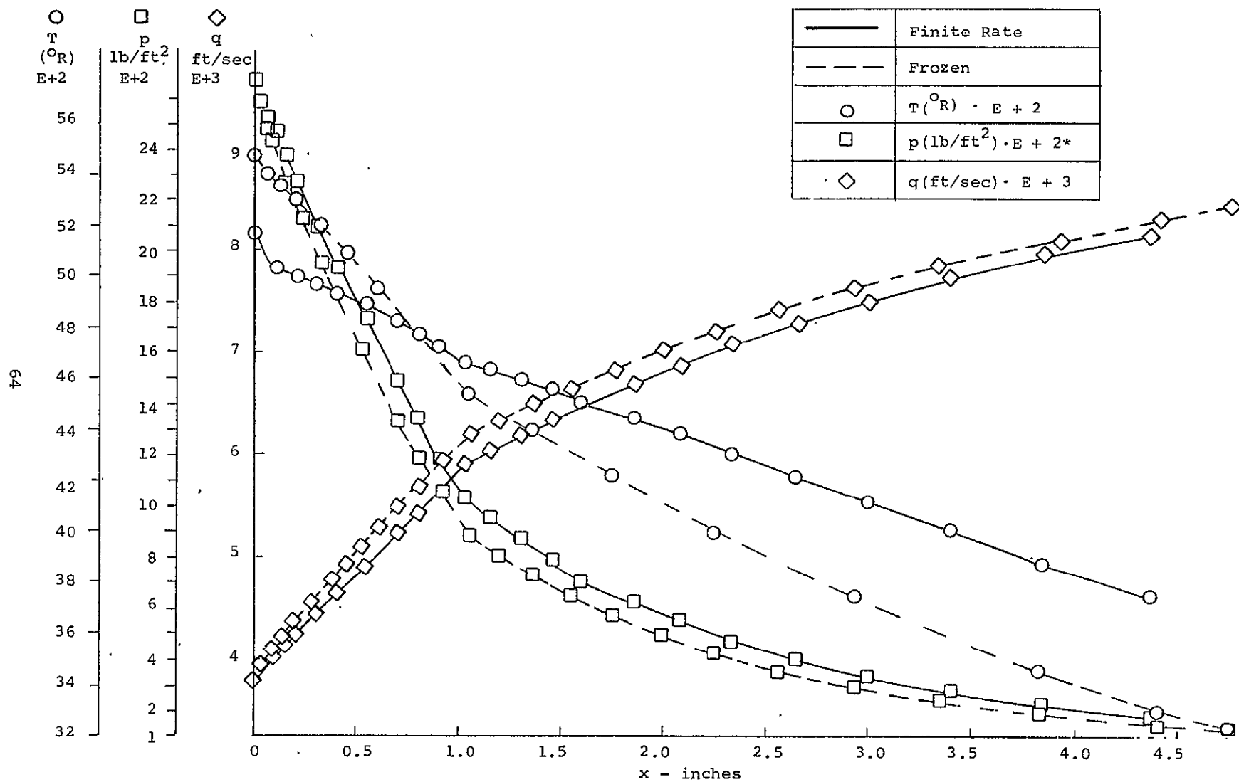
FIGURE 19a - WALL
