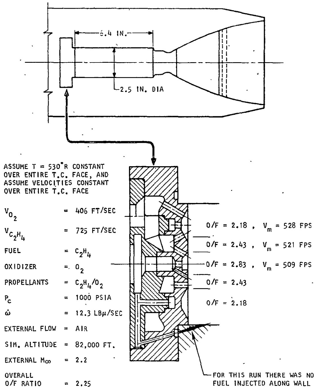
FIGURE 14 SCALE DRAWING OF CORNELL LAB. ETHYLENE-OXYGEN ROCKET ENGINE
