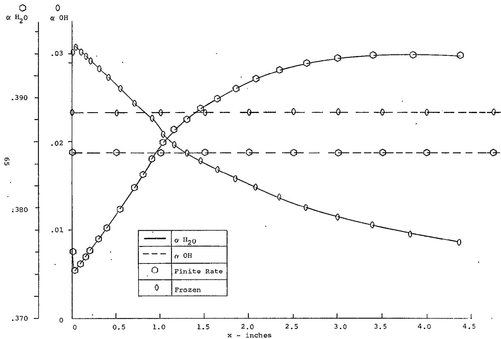
FIGURE 19b - WALL
