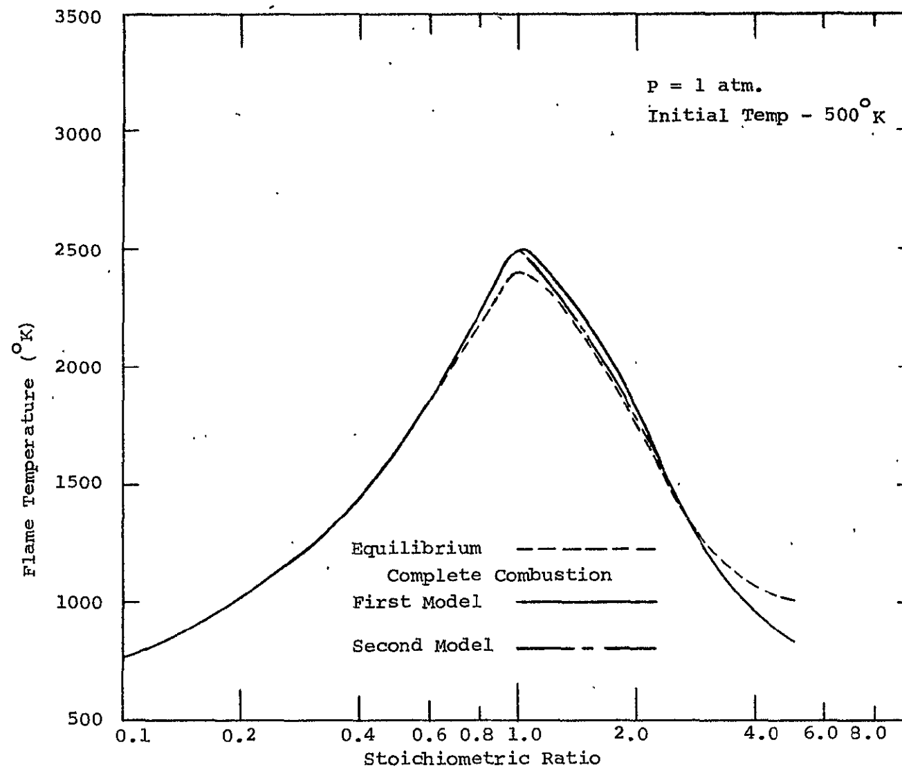
FIGURE 3 - COMPARISON OF QUASI-COMPLETE COMBUSTION MODELS WITH EQUILIBRIUM CHEMISTRY FOR A PROPANE-AIR SYSTEM
