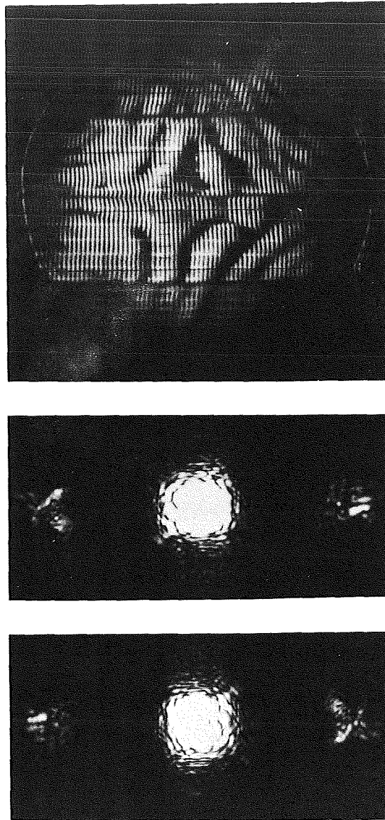
Figure 4.3 Top: Nontime-averaged temporal reference hologram made under the same conditions as those in Figure 4.2 except that a cutout of the letter "X" was placed between the sound source and the camera tube. Middle: Reconstructed true image of the "X" is in focus at the left of the zero-order beam seen in the center of the picture. The out-of-focus conjugate image of the "X" is to the right of the zero-order beam. Bottom: Conjugate image on the right is in focus; the true image on the left is out of focus.
