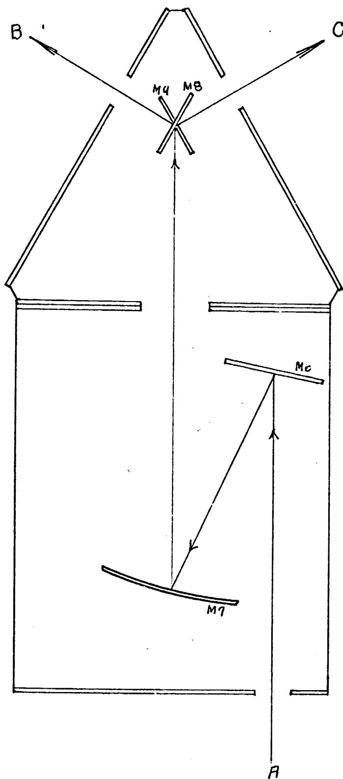
Figure 1. Reimaging Optics and Beam Splitter
