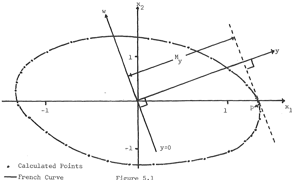
Figure 5.1 Reachable Set of (5.9)
