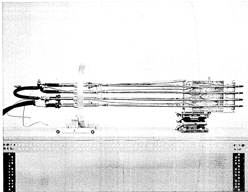
Figure VI-10. Rear view of entire multipurpose sample holder assembly.
