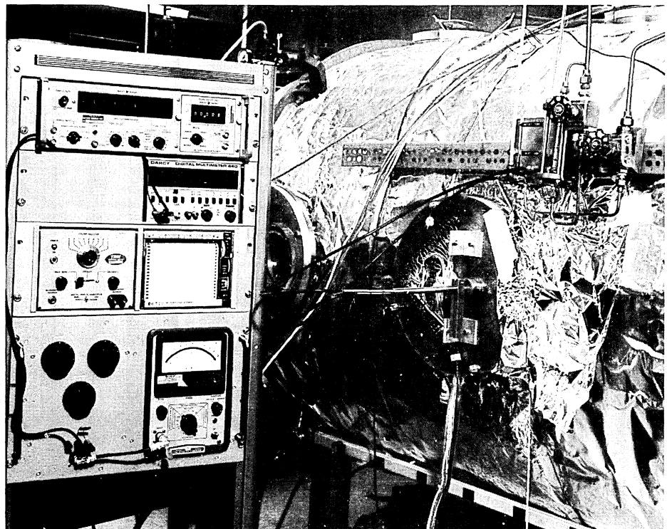
Figure IV-11. Exterior view of port plate, electronics, and water cooling system.
