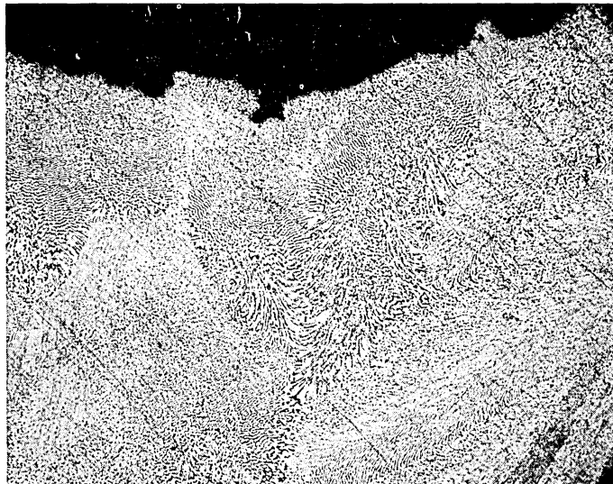
Figure III-7. Cross section of solder sample after exposure to cesium. 100X.
