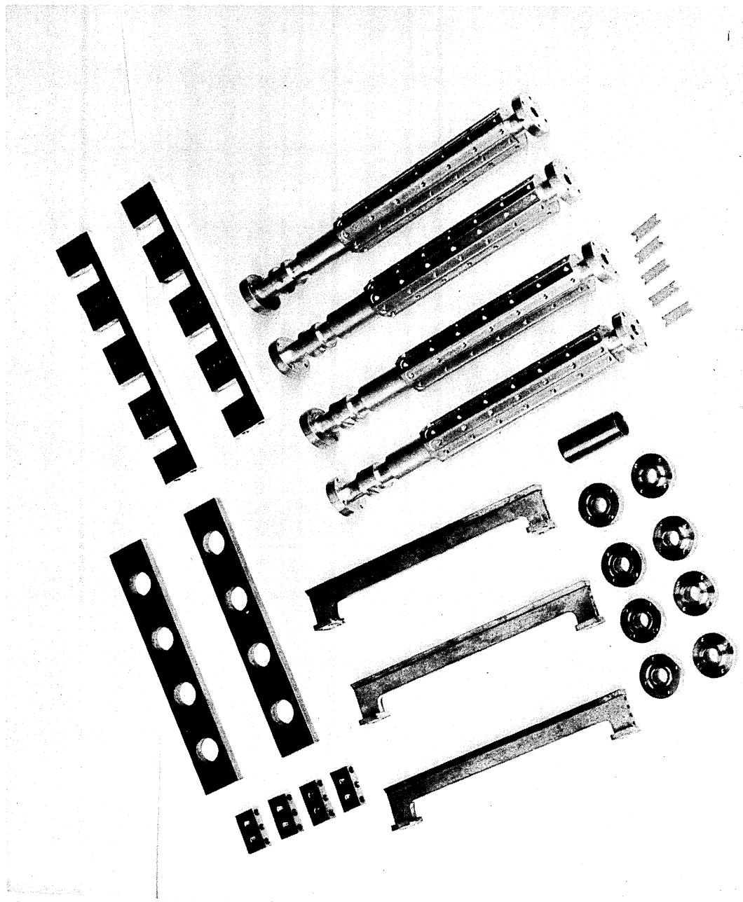
Figure VI-5. Principal parts of the multipurpose sample holder.
