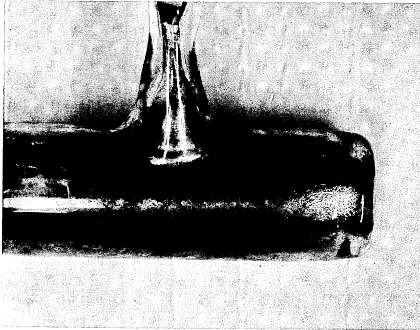
Figure III-3. Photo of upper end of test vessel showing metallic deposit.
