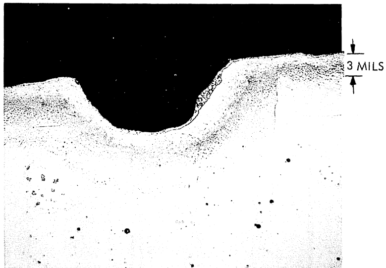
Figure III-4b. Cross section of silver casting after 4 week exposure to mercury. 100X.
