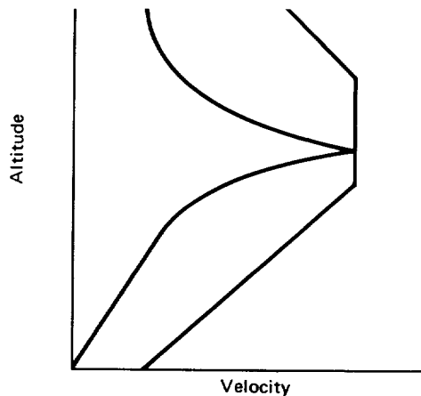
Step 6: (Optional) Extend profile upward by constructing wind-back-off curve.
