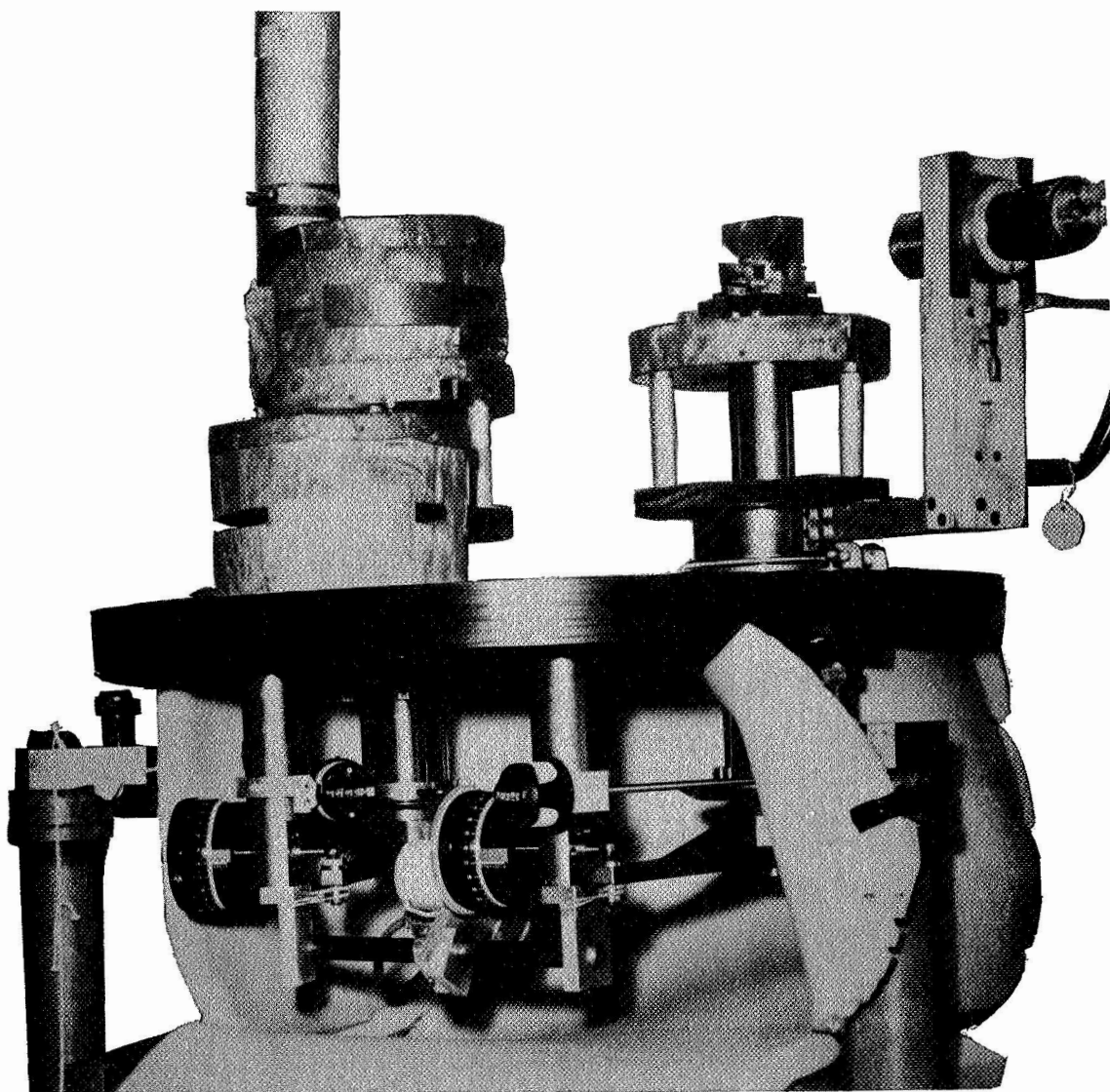
Double Crystal X-Ray Spectrometer
