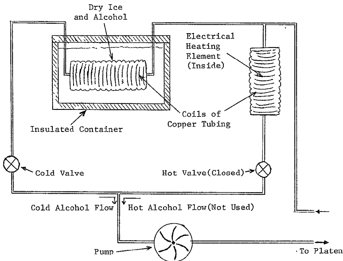
Fig. 2. -- Schematic of the physical layout of the temperature controlling system.
