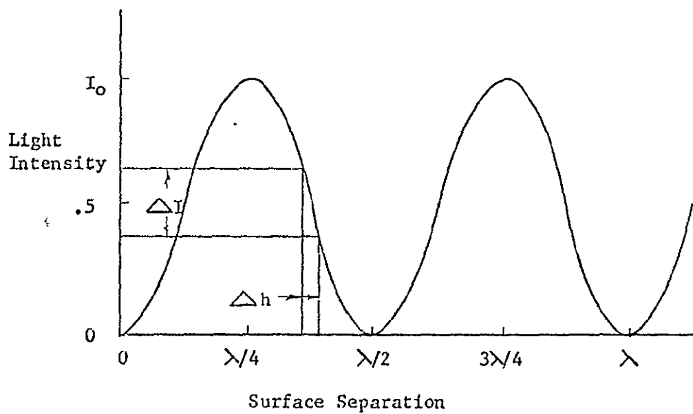
LIGHT INTENSITY VERSUS SURFACE SEPARATION IN AN OPTICAL WEDGE
