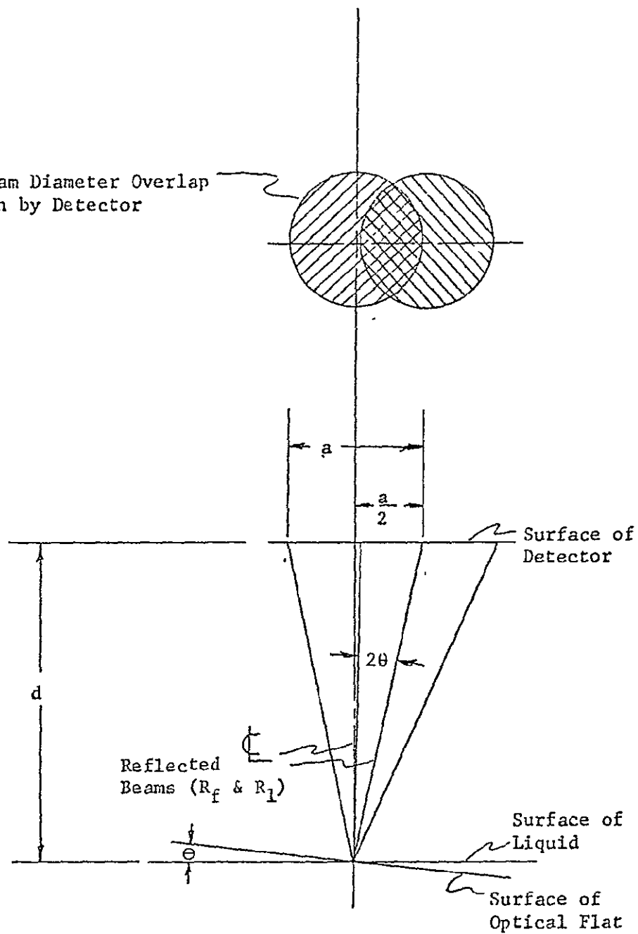
ILLUSTRATION OF OVERLAP OF REFLECTED BEAMS FROM SURFACES OF LIQUID AND OPTICAL FLAT
