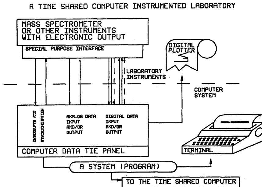
Figure 1. Typical laboratory instrumentation center contains computer data tie panel, keyboard terminal and graphic plotter.
