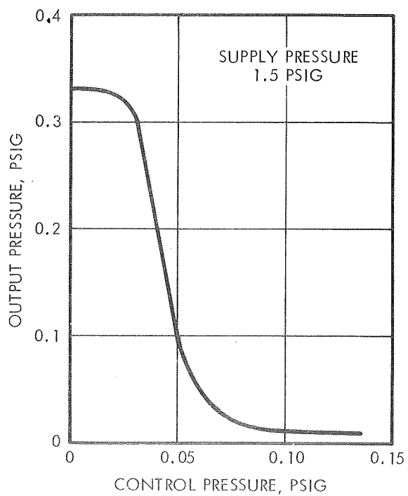
Figure 8-35. Flow Interaction NOR Input-Output Characteristics
