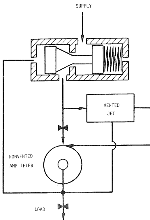
Figure 8-106. Hybrid Regulator Scheme
