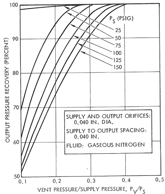
Figure 8-134. Model VJ-1 Vented Jet Pressure Recovery (0.016" Diameter Load)
