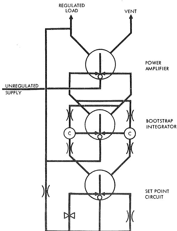
Figure 8-107. Proportional Pressure Control System
