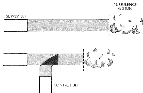
Figure 8-7. Controlled Turbulence Effect
