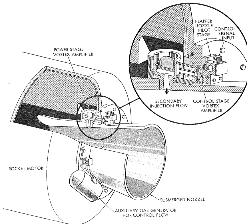
Figure 8-80. Concept of Vortex Amplifier Controlled SITVC System
