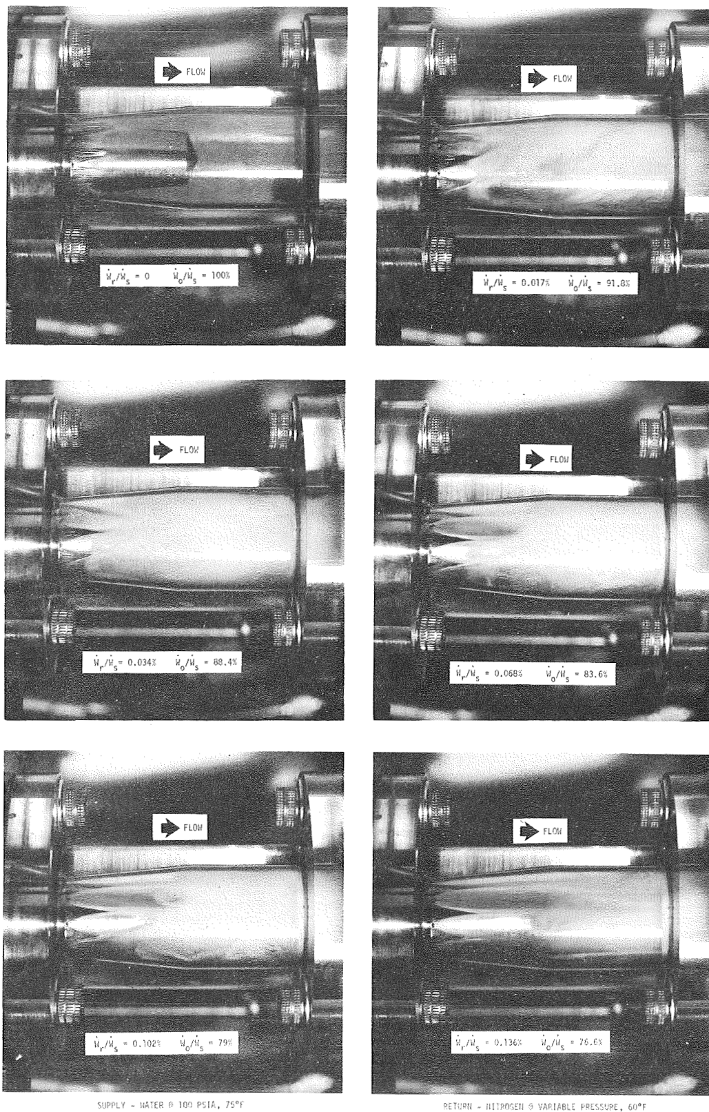
Figure 8-187. Nitrogen-Water Interaction in Venturi Sump (Pintle 12-1/2 in, P_o/P_s = 0.2 )
