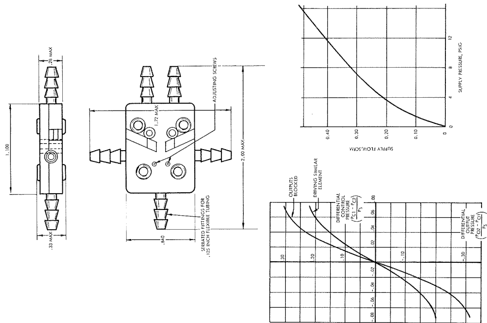
Figure 8-22. Trimable Proportional Amplifier (Courtesy of General Electric)
