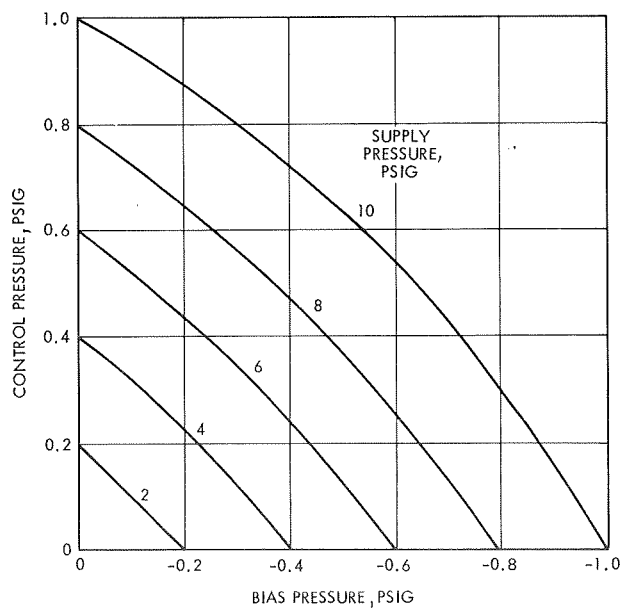
Figure 8-66. Pressure Sensor Control or Switching Pressure
