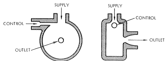
Figure 8-25. Basic Nonvented Vortex Amplifier Configuration
