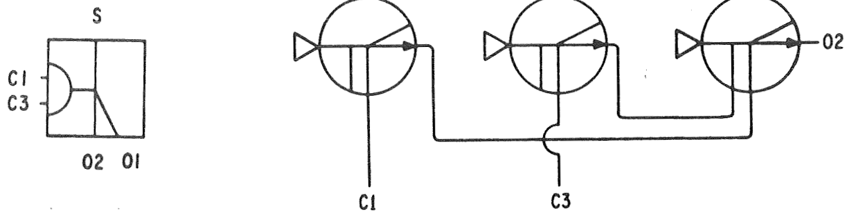
Functional Symbol
