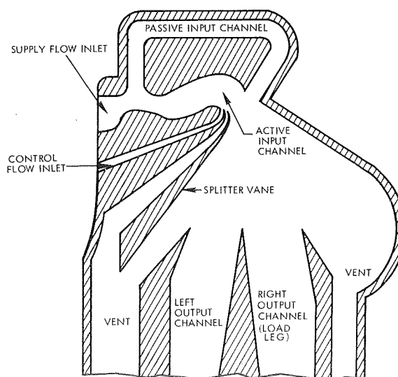
Figure 8-43. Double Leg Elbow Amplifier
