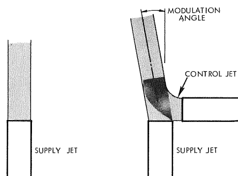
Figure 8-5. Beam Deflection Effect
