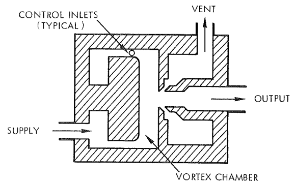
Figure 8-30. Vortex Pressure Amplifier Configuration
