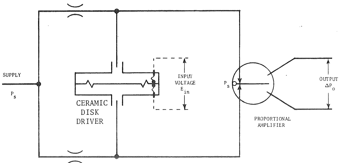
Figure 8-152. Acoustic Driver Configuration With Ceramic Disk
