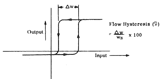
Figure 8-B3. Digital Amplifier Hysteresis
