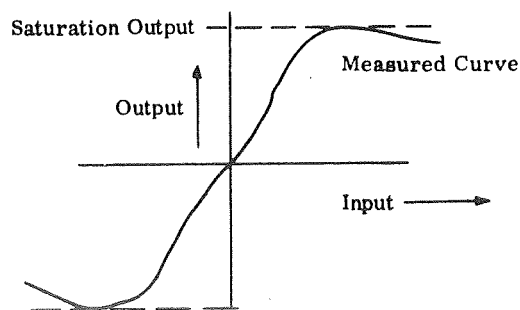
Figure 8-B6. Saturation
