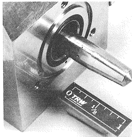
Figure 8-160. Venturi Sump Return Orifices in Pintle
