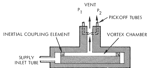
Figure 8-70. Vortex Rate Sensor
