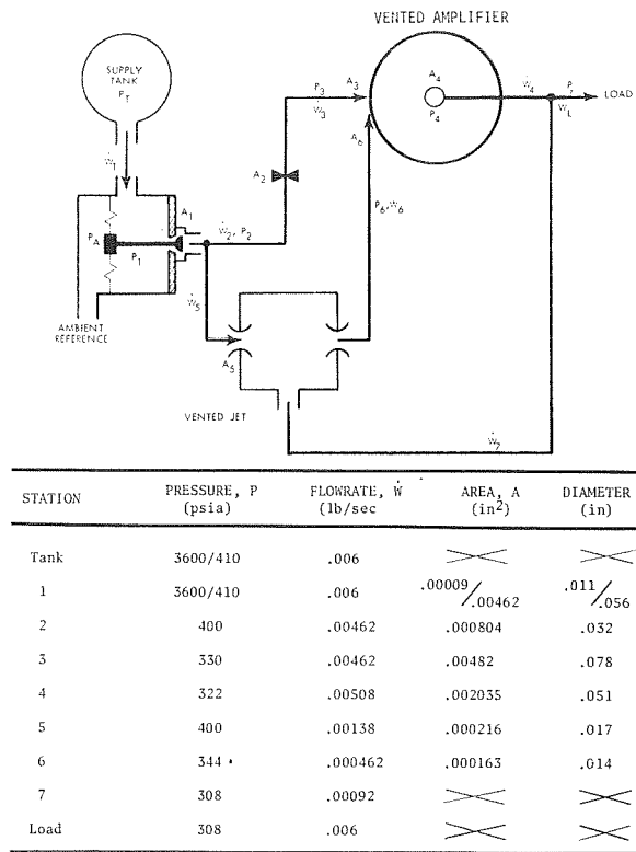
Figure 8-121. Hybrid Regulator-Set Point Parameters
