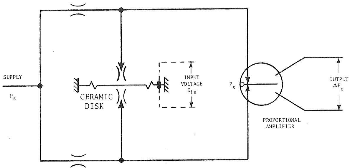
Figure 8-151. Balanced Flapper Nozzle Configuration with Ceramic Disk
