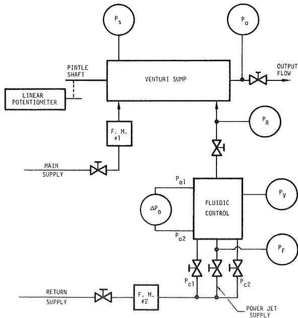
Figure 8-163. Fluidic Control Demonstration Test Setup
