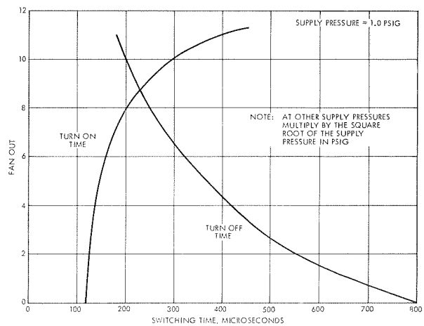
Figure 8-39. Impact Modulator NOR Switching Time
