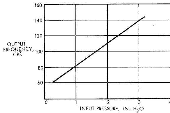
Figure 8-52. Pressure Controlled Oscillator Performance
