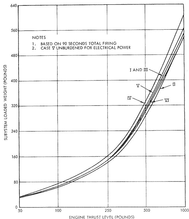
Figure 8-119. Propulsion Subsystem Loaded Weight Comparisons
