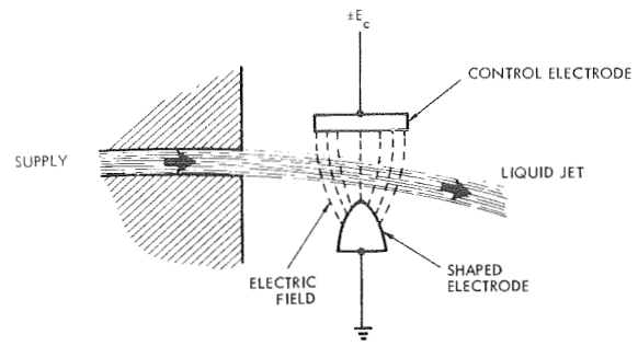
Figure 8-139. Free Jet Modulation by Nonuniform Field
