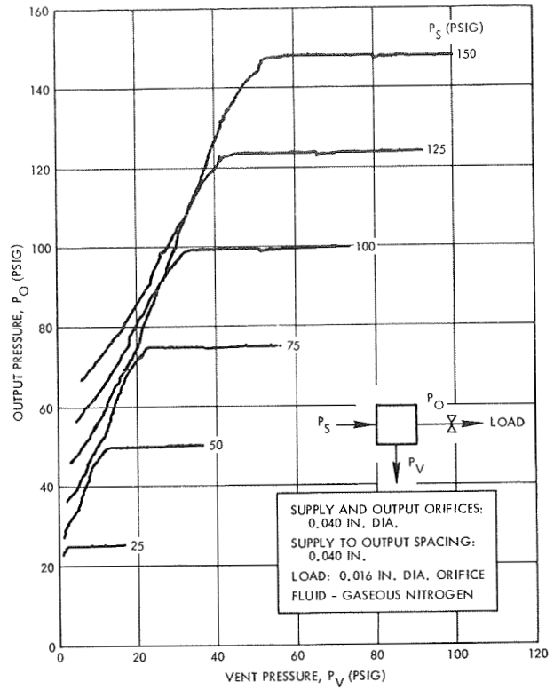
Figure 8-132. Model VJ-1 Vented Jet Performance (0.016" Diameter Load)
