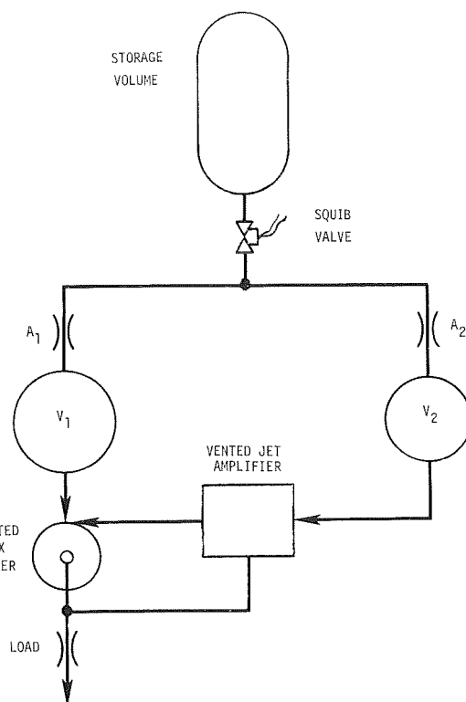
Figure 8-105. Lag Circuit Regulator
