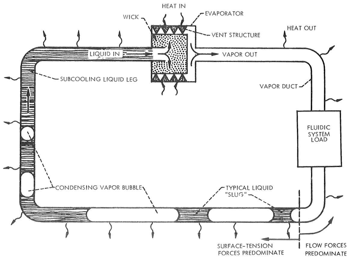
Figure 8-156. Capillary Pumped Heat Transfer Loop
