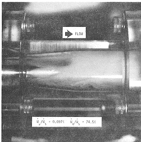
Figure 8-186. Nitrogen-Water Interaction in Venturi Sump (Pintle Full Out, P_o/P_s = 0.2 )
