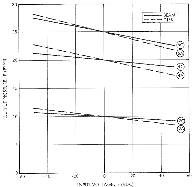
Figure 8-149. Comparison of Disc and Beam E-F Transducer Calibration
