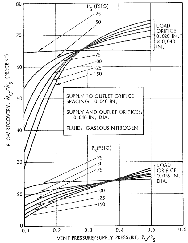
Figure 8-136. Model VJ-1 Vented Jet Output Flow Recovery
