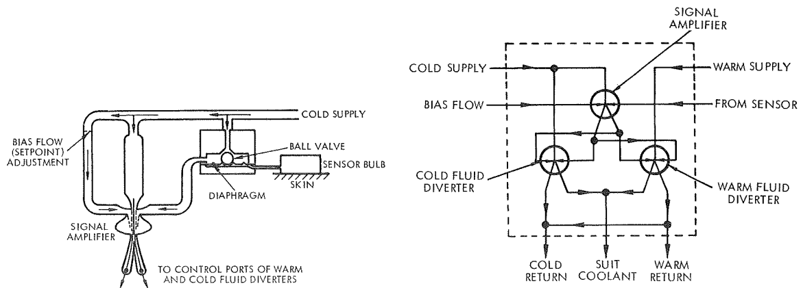
Figure 8-89. Sensor-Signal Amplifier Circuit
