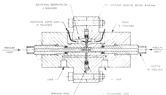
Figure 8-145. Piezoelectric E-F Transducer
