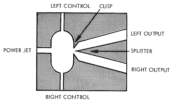
Figure 8-45. Edgetone Amplifier
