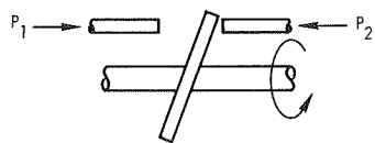
(b) ANGULAR DISPLACEMENT WITH WOBBLE PLATE
