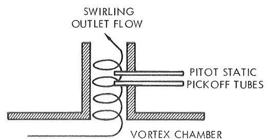
Figure 8-71. Rate Sensor Aerodynamic Pickoff Tubes
