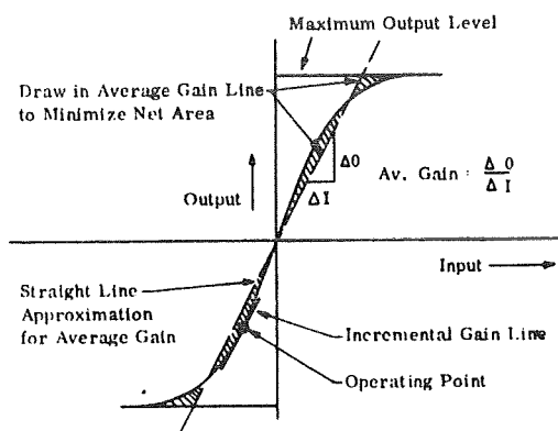
Figure 8-B1. Pressure Gain
