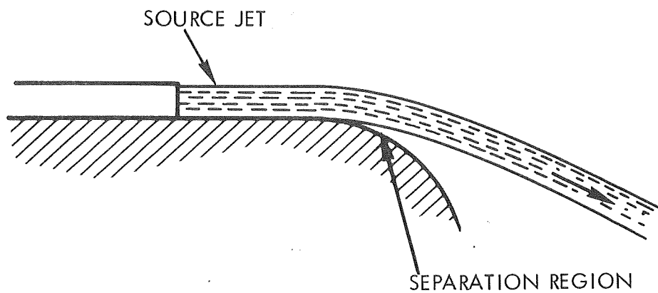
Figure 8-9. Separation Effect
