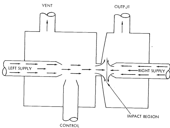
Figure 8-46. Transverse Impact Modulator
