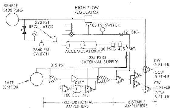
Figure 8-84. TIM Fluidic Control System
