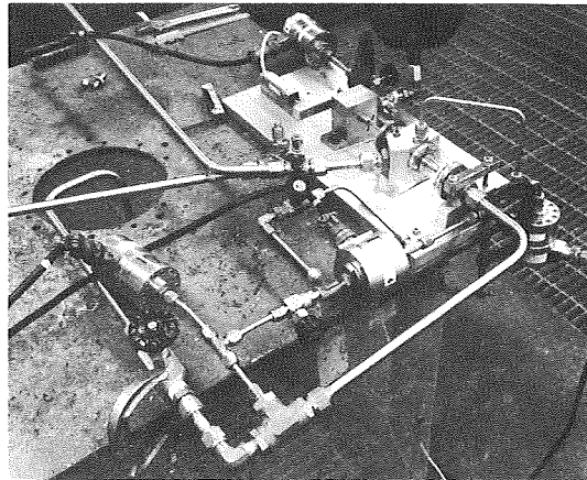
Figure 8-162. Venturi Sump Test Setup
