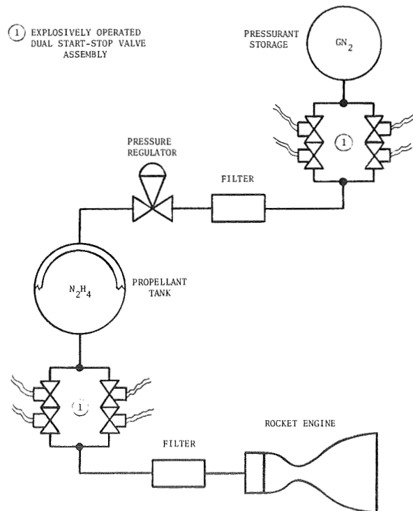
Figure 8-111. Baseline Monopropellant Hydrazine Propulsion System
