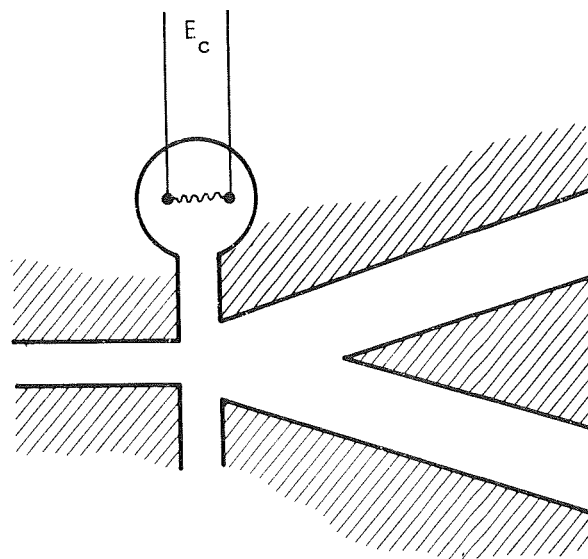
Figure 8-144. Bistable Device Switching by Spark Discharge
