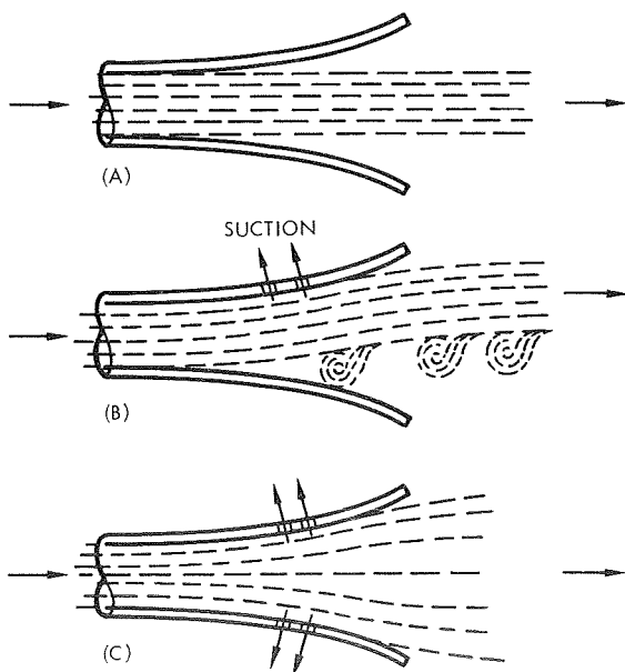
Figure 8-1. Prandtl Diffuser
