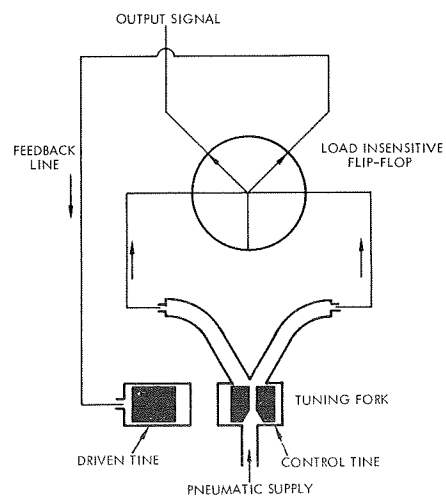
Figure 8-54. Fluidic Tuning Fork Oscillator
