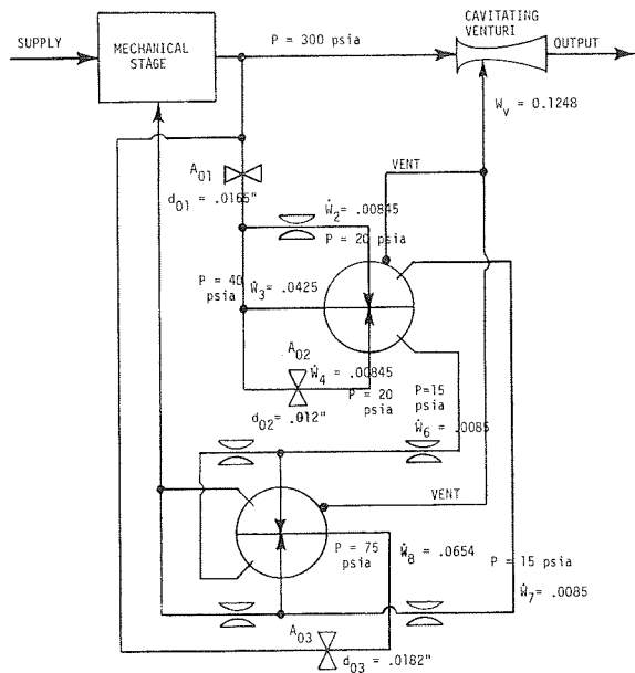
Figure 8-127. Simplified Hybrid Flow Regulator - Scheme II
