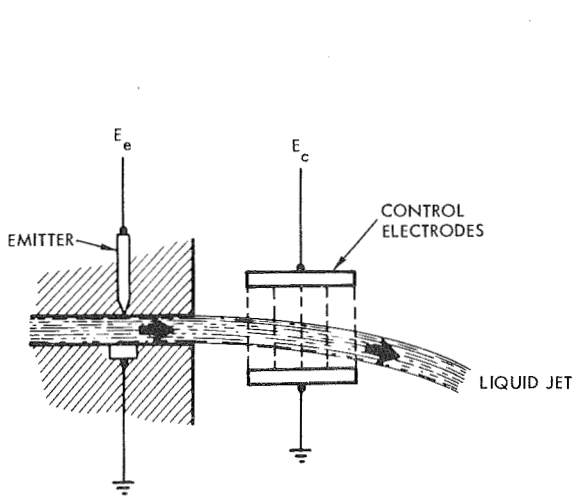
Figure 8-138. Free Jet Deflection by Coulomb Attraction
