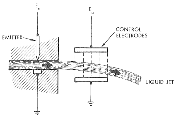
c. Charged Free Jet Deflection by Linear Field
