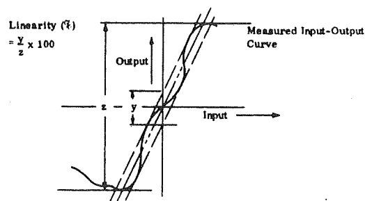
Figure 8-B4. Output Linearity
