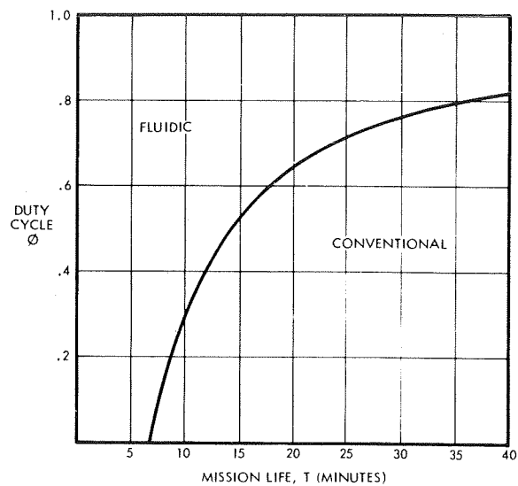
Figure 8-96. Optimum System Weight Regimes
