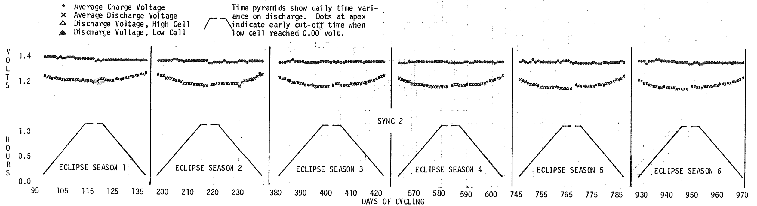
VOLTAGE CHARACTERISTICS OF SYNCHRONOUS PACKS VERSUS DAYS OF CYCLING FOR SUCCESSIVE ECLIPSE SEASONS
