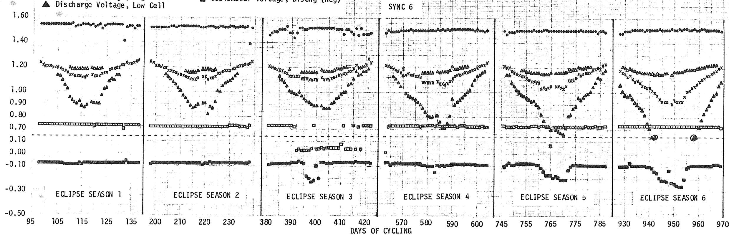
VOLTAGE CHARACTERISTICS OF SYNCHRONOUS PACKS VERSUS DAYS OF CYCLING FOR SUCCESSIVE ECLIPSE SEASONS
