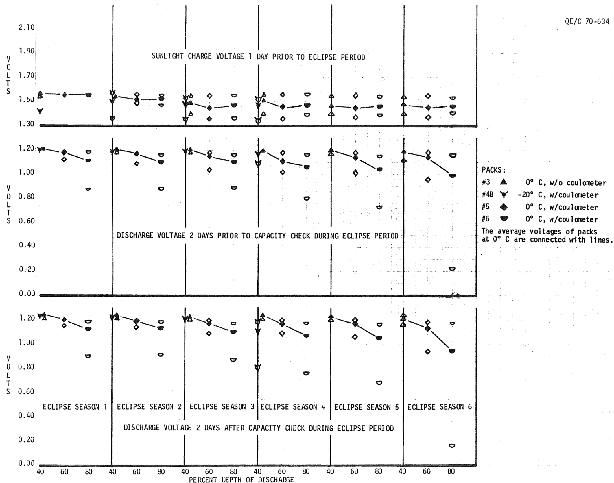
CROSS-SECTIONAL VOLTAGE CHARACTERISTICS VERSUS DEPTH OF DISCHARGE
