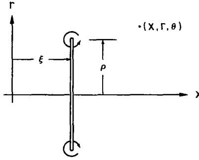
Figure 2. Interpretation Of The Green's Function
