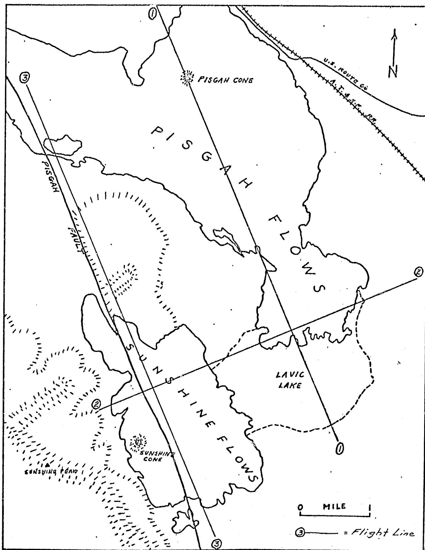
PISGAH CRATER &amp; VICINITY, CALIFORNIA - TEST SITE
