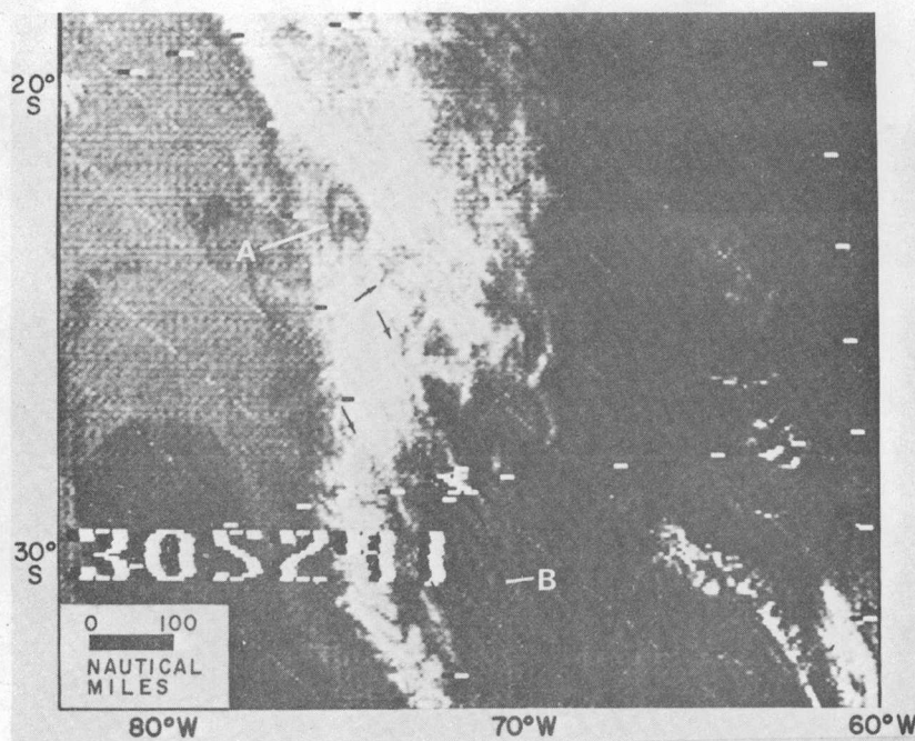
Figure 6 Nimbus I HRIR image of western South America (magnified); A - Atacama Desert, B - Sierra del Pie de Palo. Orbit 246, Data Block 184.
