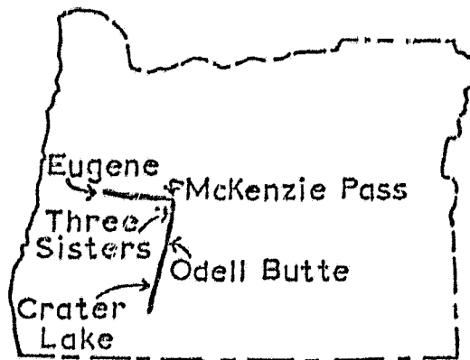
Figure 1. Index map showing path of infrared imagery and principal localities mentioned in text.
