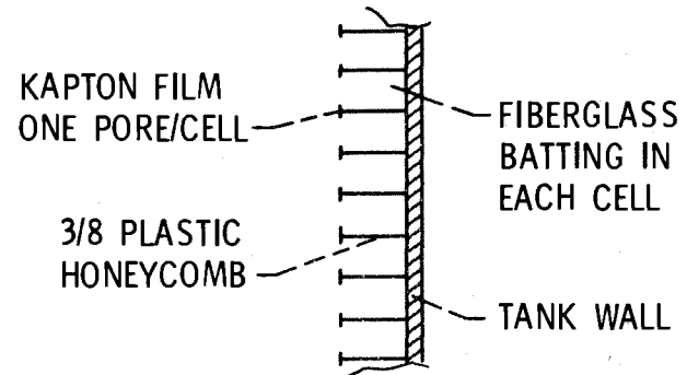
SST METHANE TANK (NAS3-12425)
