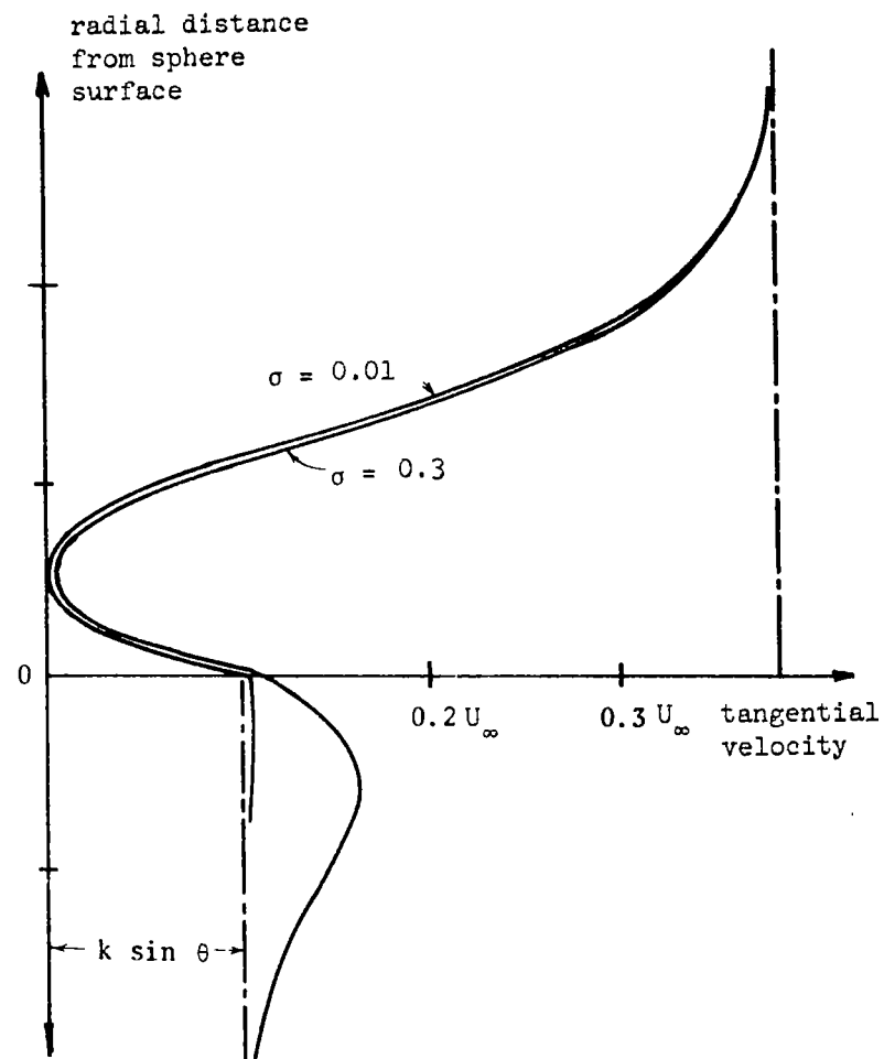
Figure 2. Separation profile at 165^\circ for \sigma = 0.01 and \sigma = 0.3 and k = 0.4 .
