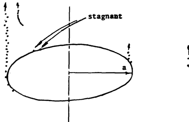
Figure 8(a). Path of pliolite particles relative to a 3.8 mm by 7.7 mm glycol drop in 5.5 cp silicone oil.
