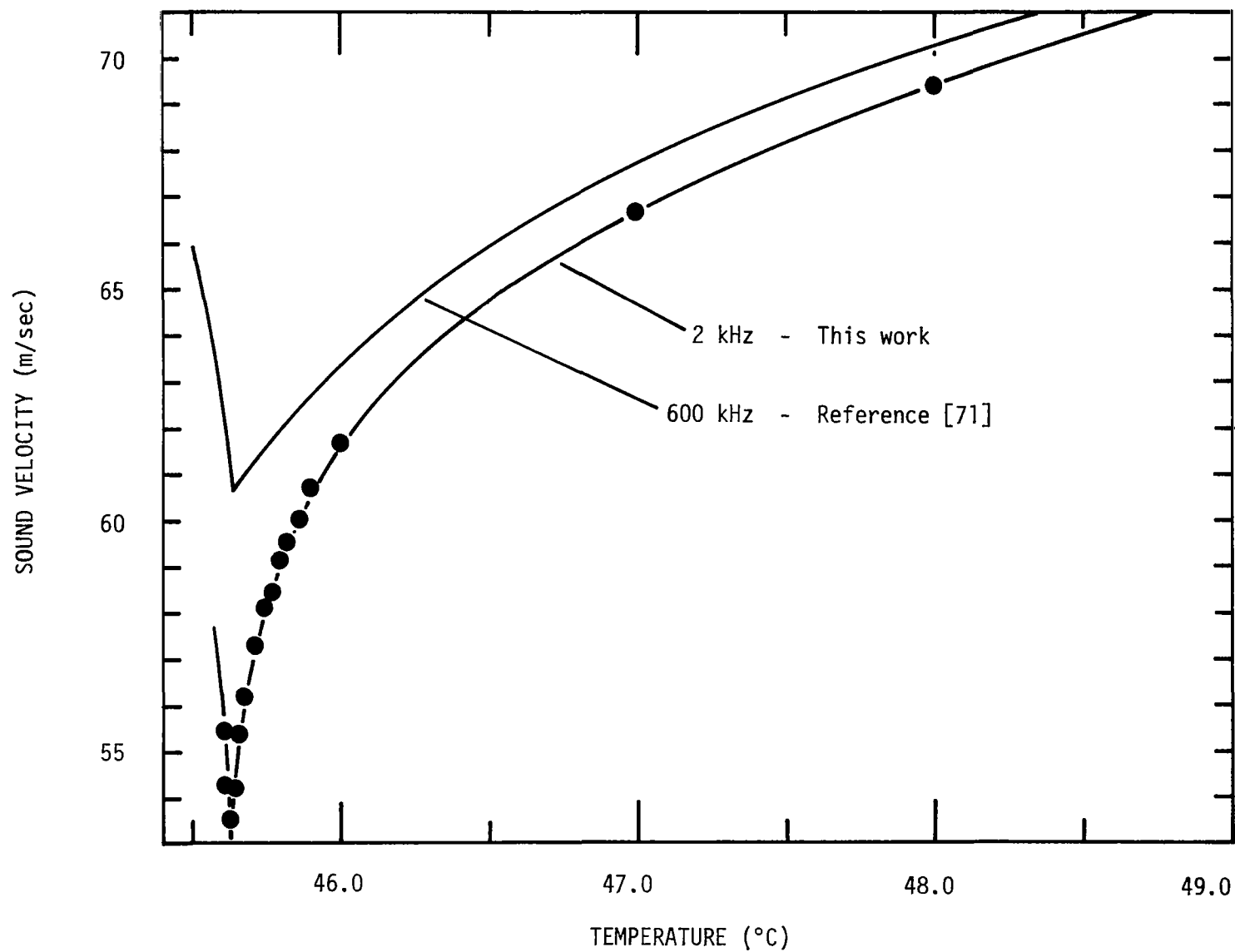
FIG. 17. SOUND VELOCITY AS A FUNCTION OF TEMPERATURE IN \text{SF}_6 AT CRITICAL DENSITY.
