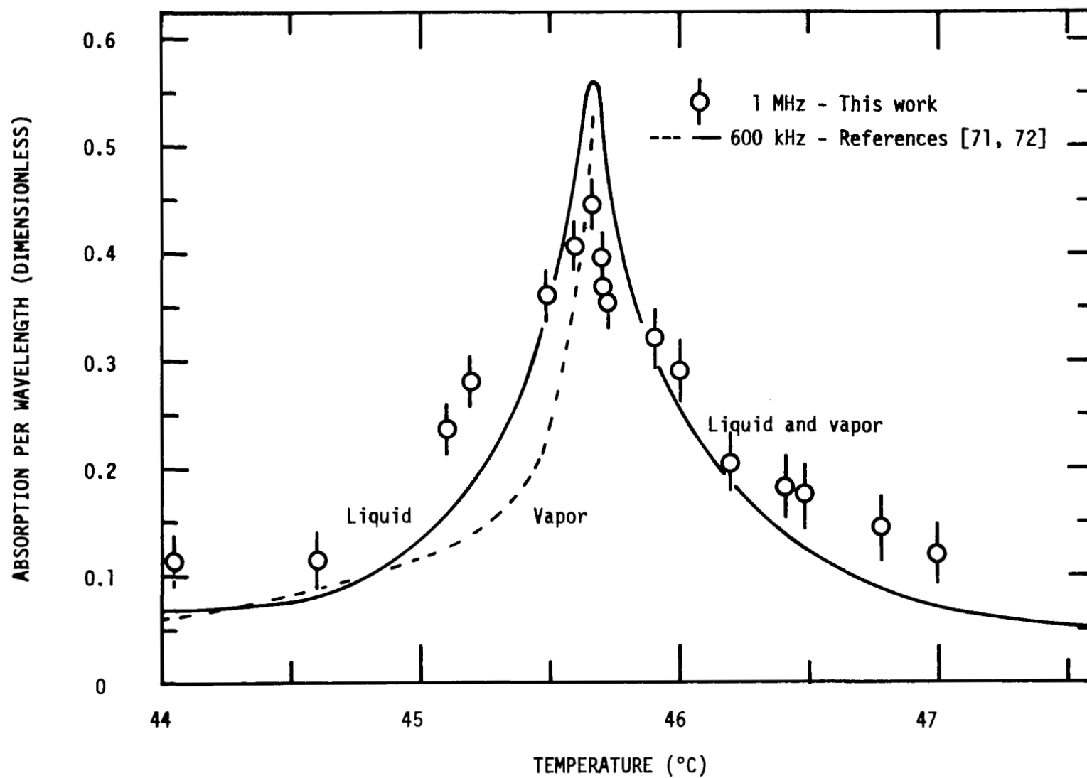
FIG. 20. SOUND ABSORPTION PER WAVELENGTH AS A FUNCTION OF TEMPERATURE IN \text{SF}_6 .
