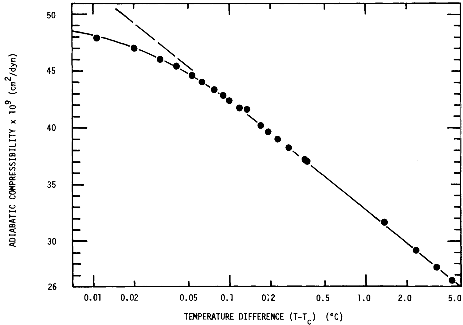
FIG. 18. ADABIATIC COMPRESSIBILITY AS A FUNCTION OF TEMPERATURE DIFFERENCE FOR \text{SF}_6 AT CRITICAL DENSITY.
