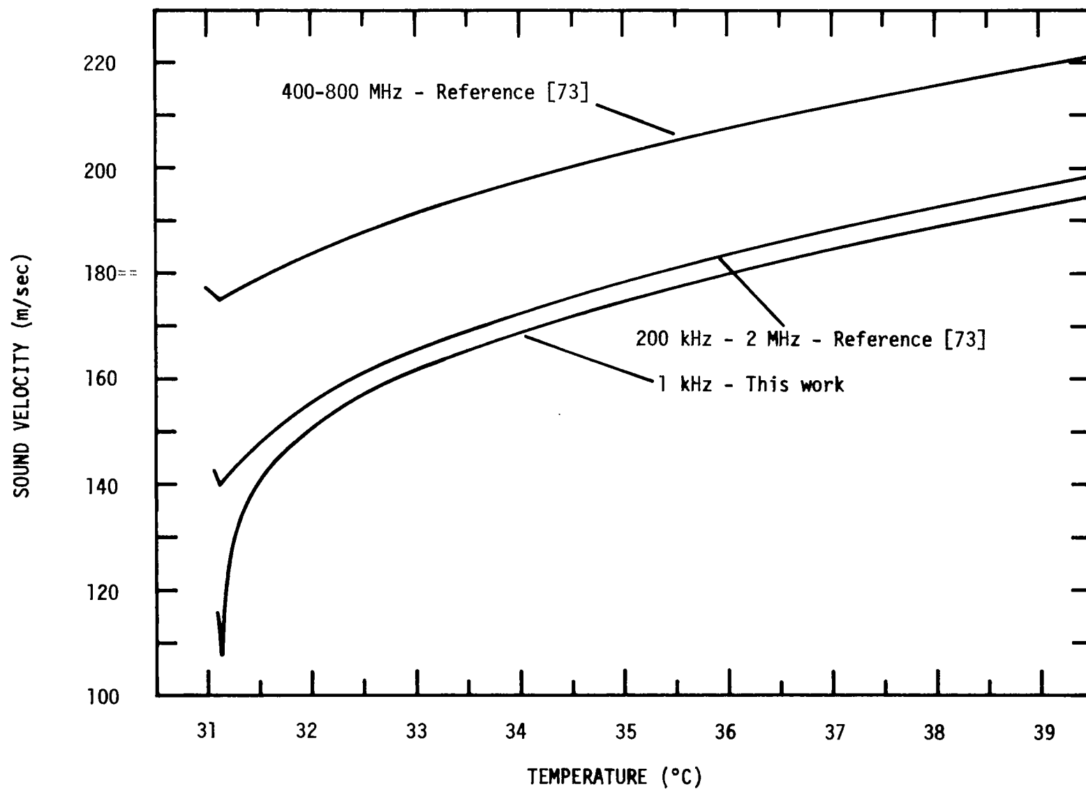
FIG. 21. SOUND VELOCITY AS A FUNCTION OF TEMPERATURE IN CO 2 AT CRITICAL DENSITY.
