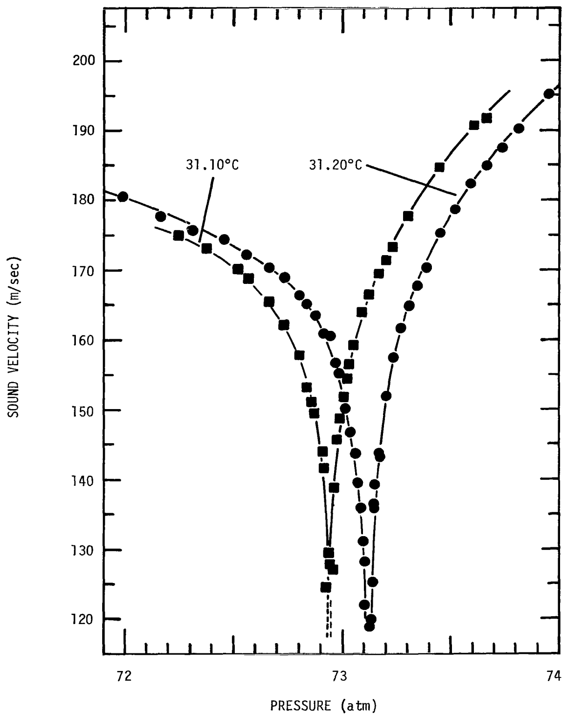
FIG. 14. SOUND VELOCITY AS A FUNCTION OF PRESSURE IN \text{CO}_2 AT 31.10^\circ\text{C} AND 31.20^\circ\text{C} .
