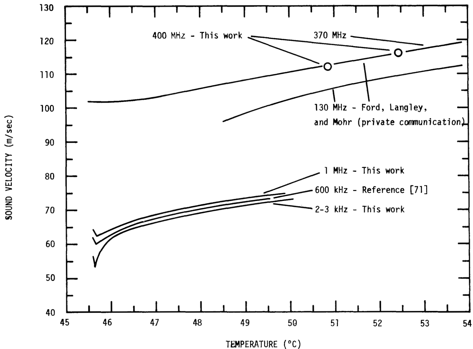
FIG. 19. SOUND VELOCITY AS A FUNCTION OF TEMPERATURE IN \text{SF}_6 AT CRITICAL DENSITY.
