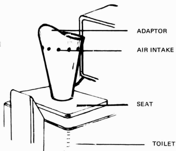
BOTH TYPES OF VOMITUS COLLECTION ADAPTORS SHOWN INSTALLED
