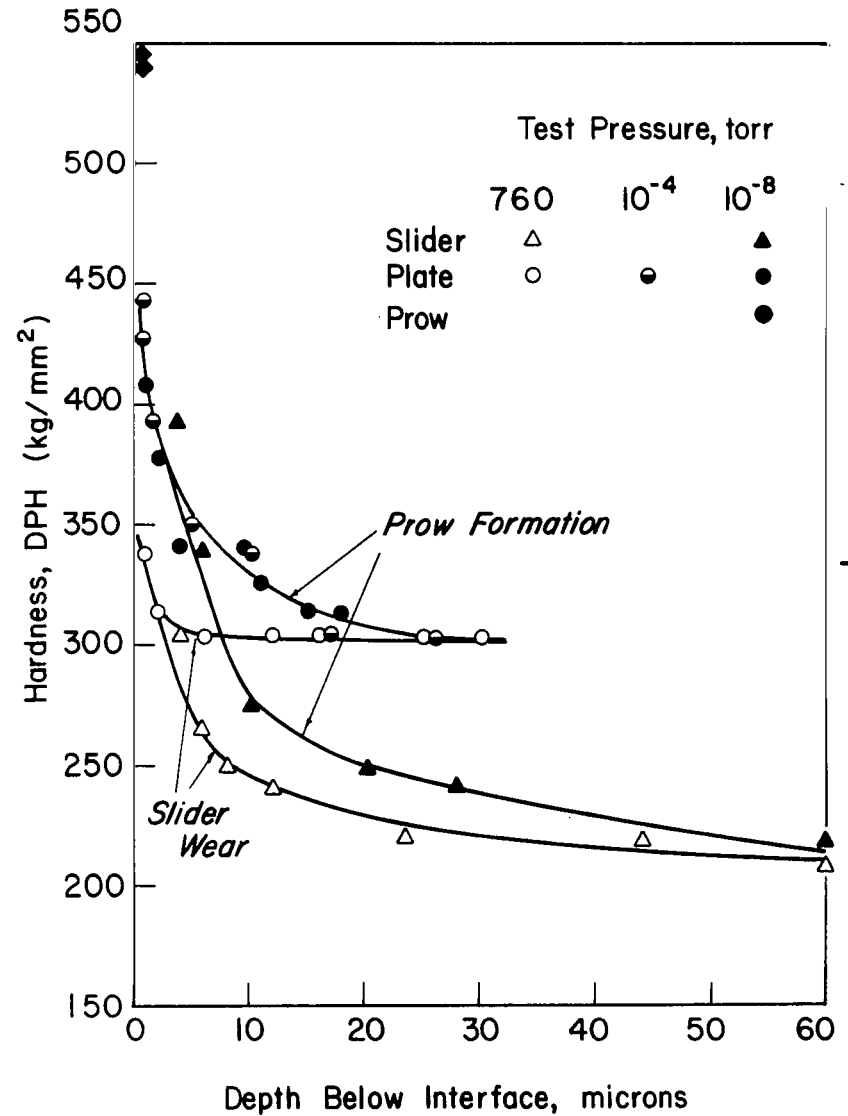
Figure 4-Microhardness traverses across wear interface for 1020 steel sliders (DPH 190) on 4340 steel plate (DPH 300).
