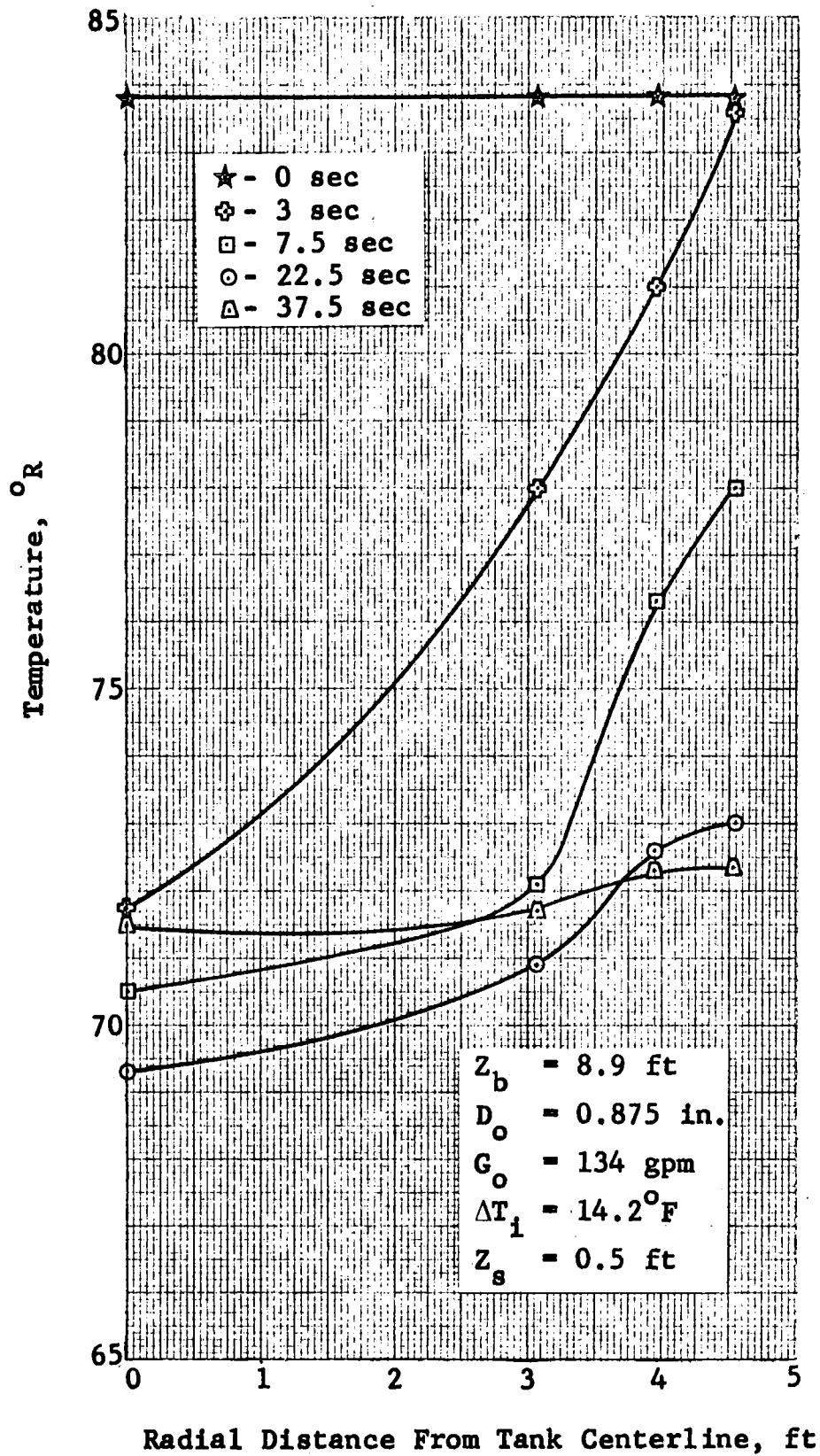
Figure 6 Large-Scale Tank Surface Temperature Variation During Mixing: Run 49
