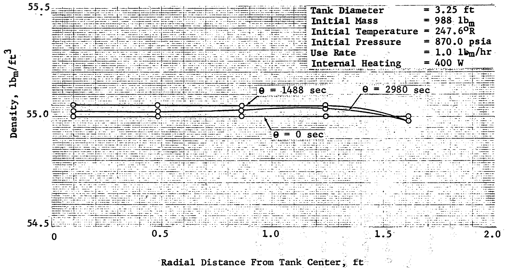
Figure 34 Density Variations in Supercritical Oxygen; Tank Diameter = 3.25 Ft
