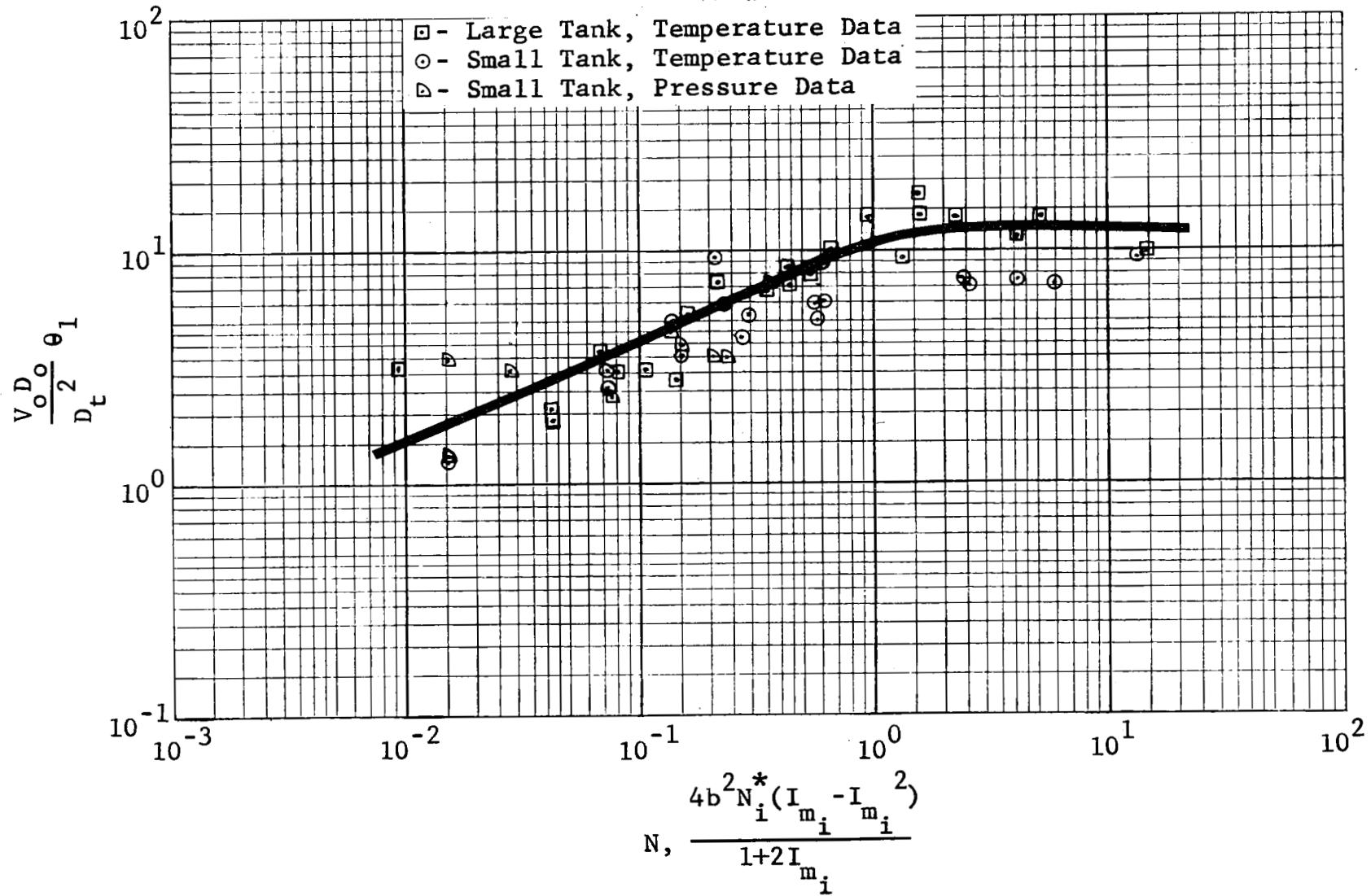
Figure 27 Correlation of the Dimensionless Time Required for Temperature Stratification or Ullage Pressure To Reach 10% of Its Initial Value Versus N: Large and Small Tank Tests
