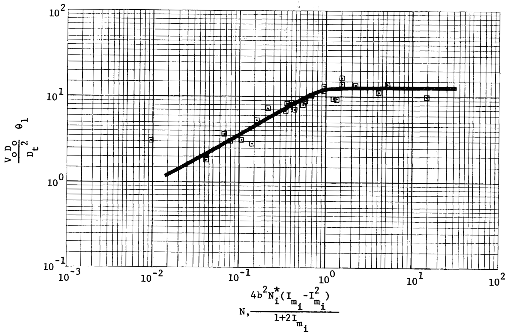
Figure 19 Correlation of Dimensionless Time Required for Temperature Stratification to Reach 10% of Its Initial Value Versus N : Large-Scale Tests
