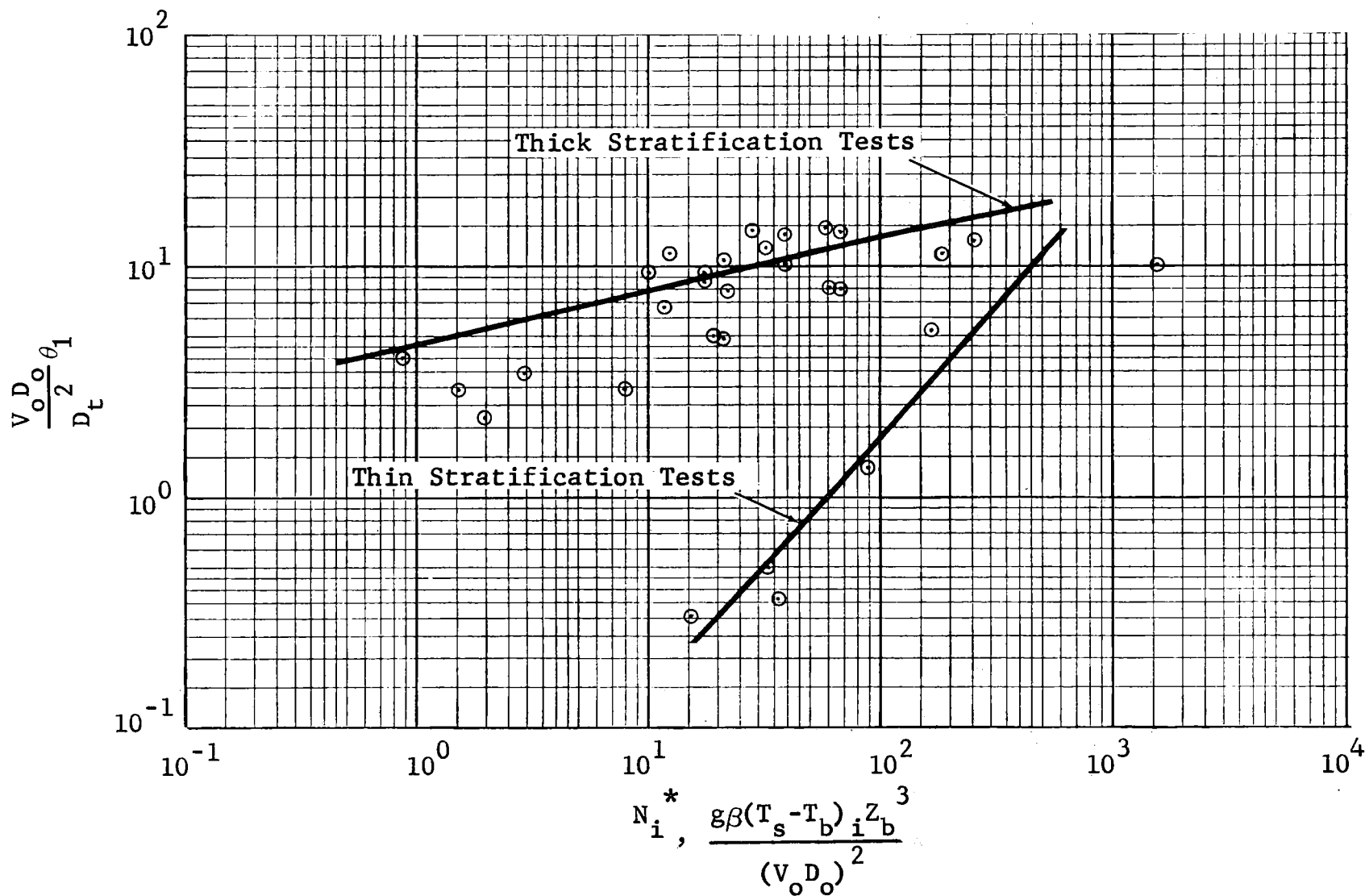
Figure 17 Correlation of Dimensionless Time Required for Temperature Stratification to Reach 5% of Its Initial Value Versus N_i^* : Large-Scale Tank Tests
