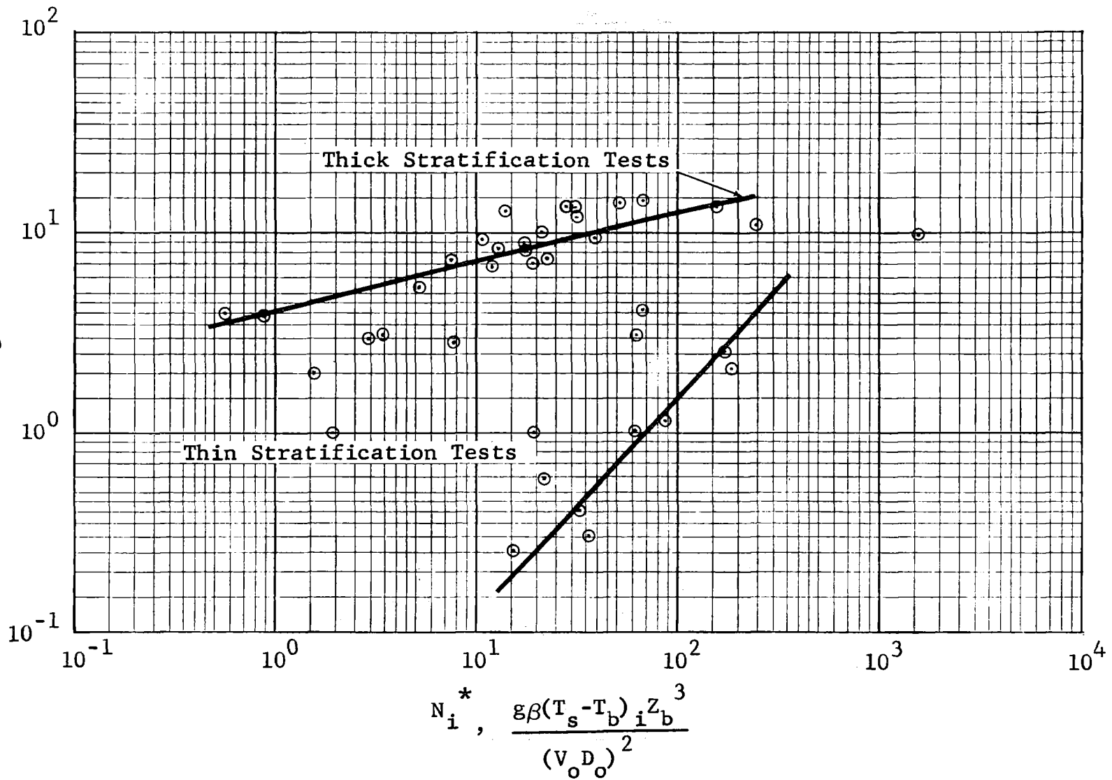
Figure 16 Correlation of Dimensionless Time Required for Temperature Stratification to Reach 10% of Its Initial Value Versus N_i^* : Large-Scale Tank Tests
