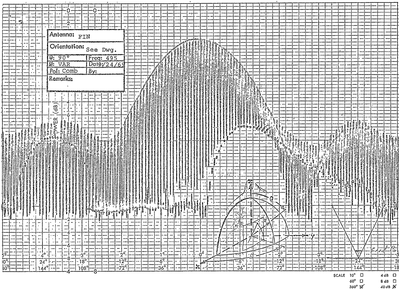
Figure 45. Pattern of Vee Fin Fed At Apex -57-
