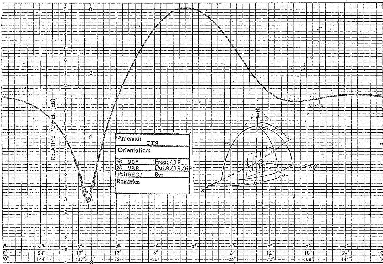
Figure 36. Pattern of Fin With Reversed Parasite \lambda/4 Distant, Circular Polarization
