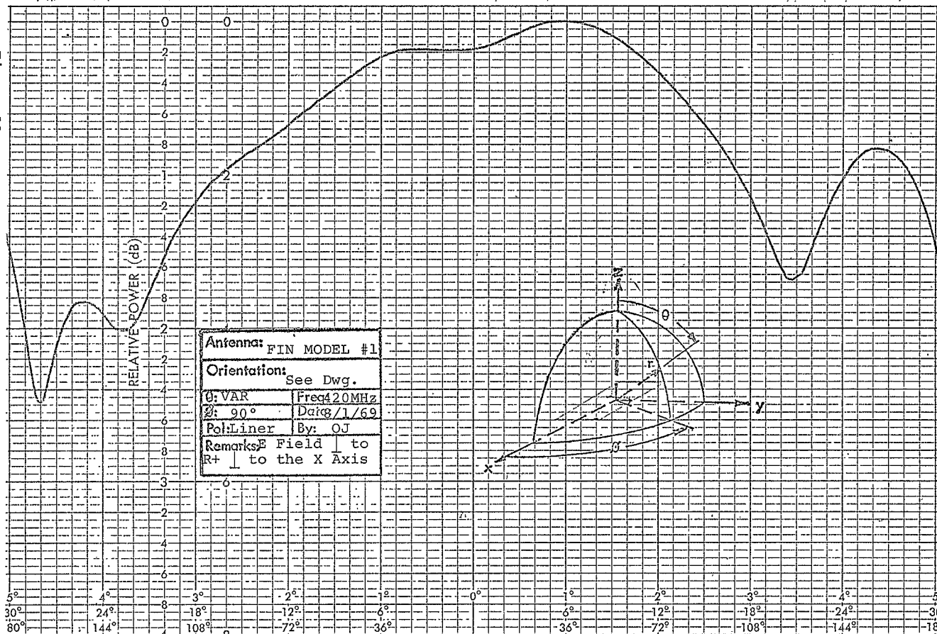
Figure 11. Pattern For Large Groundplane, \phi=90^\circ , Y-Axis Polarization
