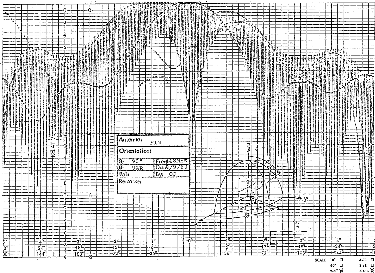
Figure 25. Pattern For Blocking Plate 3/4" From Fin
