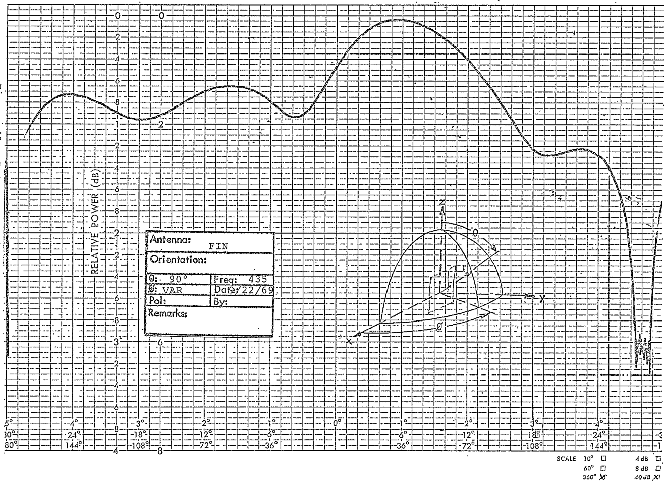
Figure 40. Pattern of Fin With Open Top, Circular Polarization
