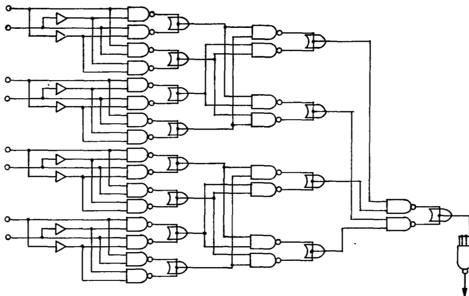
NAND GATE LOGIC FOR 8-BIT PARITY (From Parity Logic Board SPC-102 Dwg.32801)
