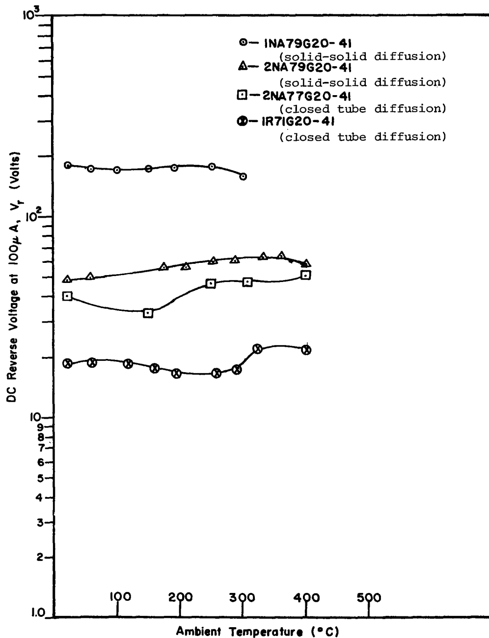
FIGURE 12(b). CYCLIC VARIATION OF D.C. REVERSE VOLTAGE (AT 100\mu a REVERSE CURRENT) WITH TEMPERATURE
