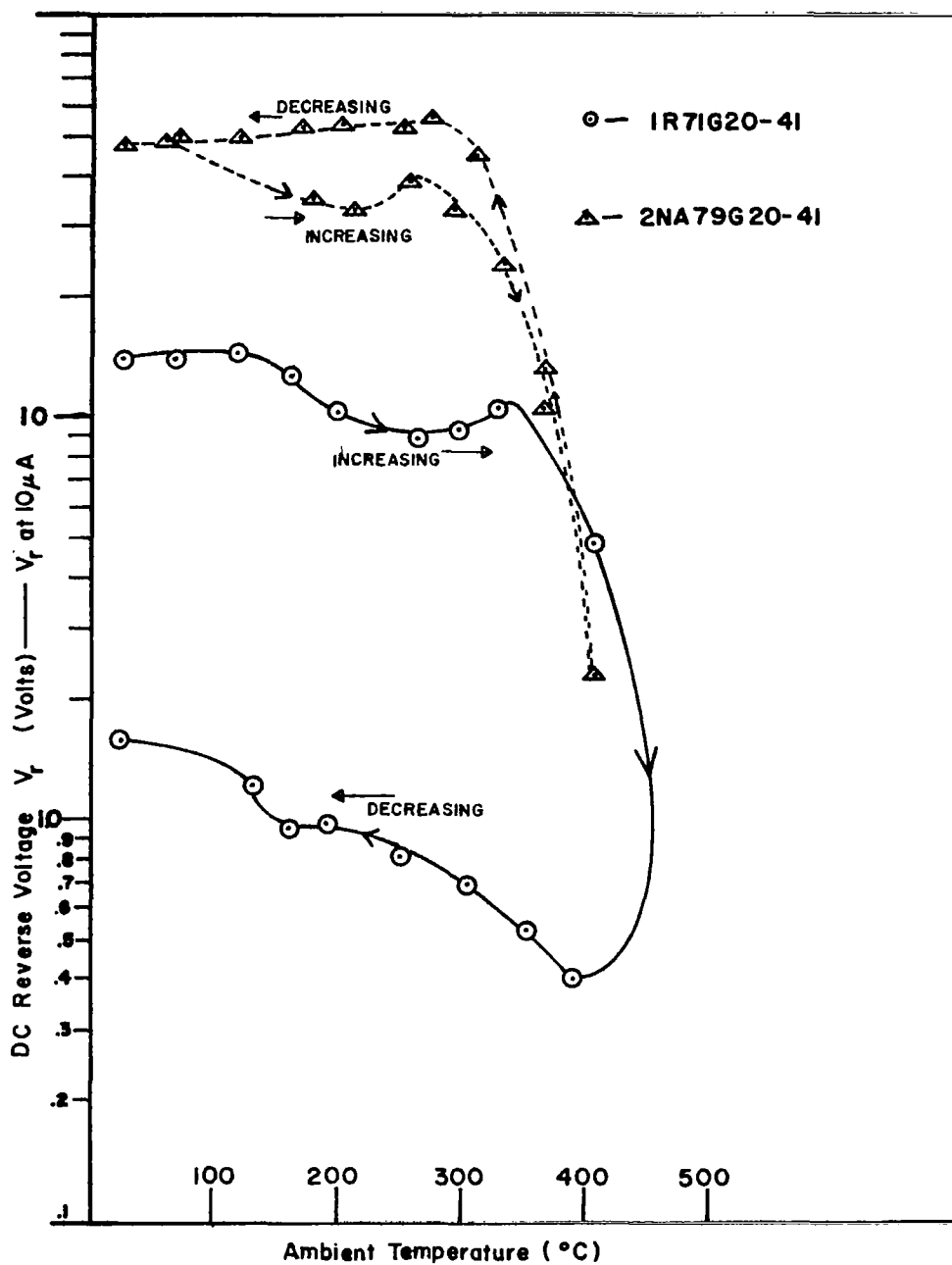
FIGURE 13. CYCLIC VARIATION OF REVERSE VOLTAGE AT 10\mu a REVERSE CURRENT WITH TEMPERATURE (Samples 1R71 G20-41 and 2 NA 79 G20-41)
