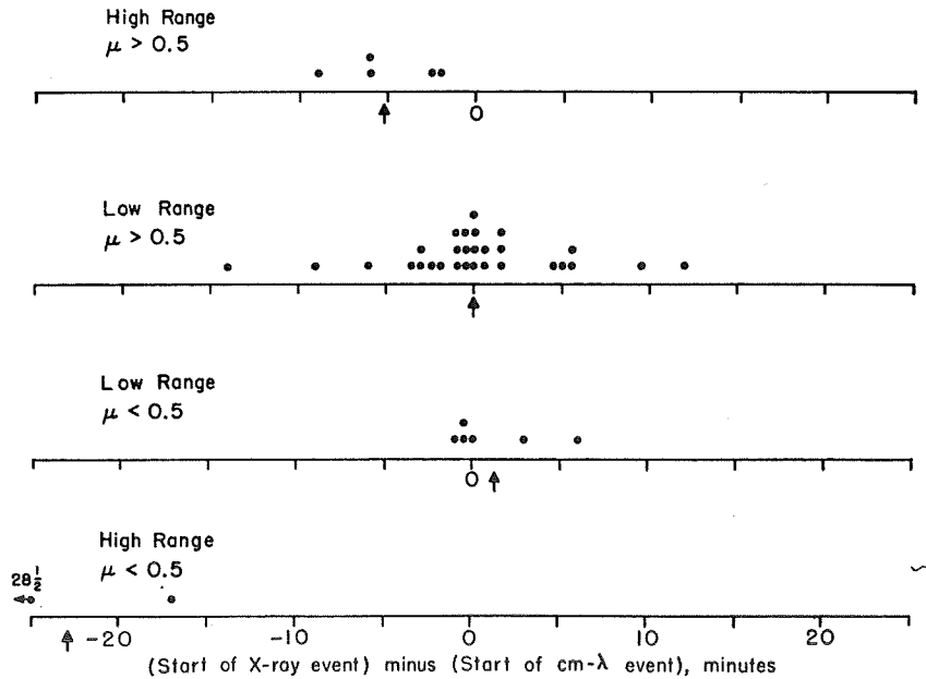
Fig. 9. Comparison of reported starting times of cm- \lambda bursts and soft X-ray enhancements. Each dot is a single event. Relative times are in the sense that negative indicates early X-rays. Arrows point to mean values.
