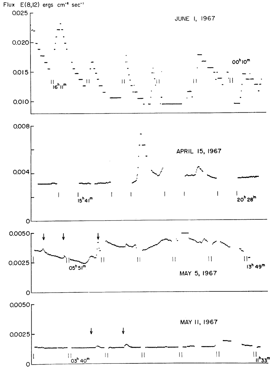
Fig. 4. Representative data for four days in 1967.
