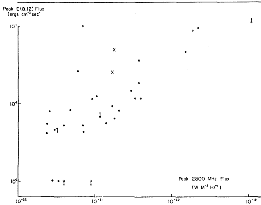
Fig. 8. Relation of peak fluxes for associated X-ray and cm- \lambda events. Filled circles: simple bursts with flares; crosses: complex bursts with flares; open circles: simple bursts without reported flares. All values are as measured at the earth, uncorrected for earth's orbital eccentricity.
