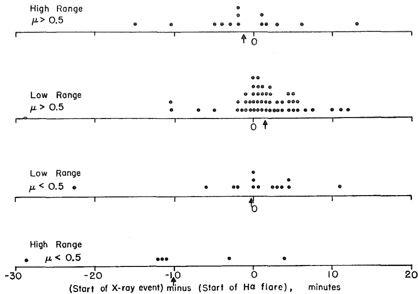
Fig. 4. Comparison of reported starting times of H \alpha flares and associated soft X-ray enhancements. Each dot is a single event. Relative times are in the sense that negative indicates early X-rays. Arrows point to mean values. Data are divided according to instrumental sensitivity range at beginning of event and according to \mu = \cos \theta .
