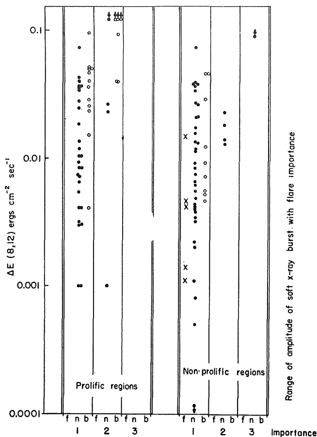
Fig. 2. Soft X-ray flux enhancements observed in flares of importance \geq 1 , divided according to flare importance and brilliance and further divided as to whether the flares occurred, in our estimation, in flare-rich or flare-poor active centers.
