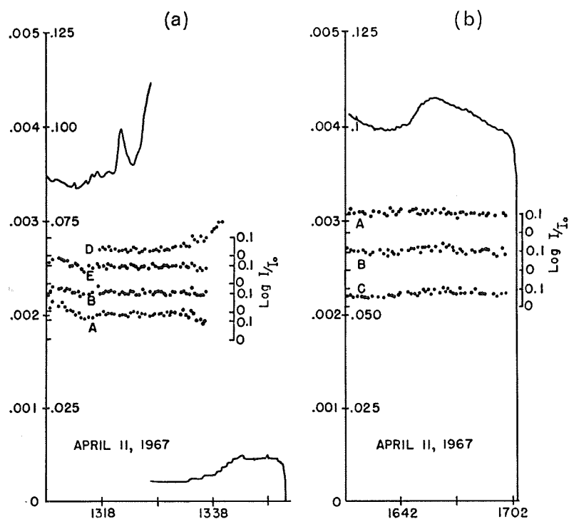
Fig. 1. - (a) Importance-1b flare (N22 W24) of April 11, 1967. Abscissa: Universal Time in hours and minutes. The solid curves are X-ray fluxes. Note change of ordinate scale at 13^{\text{h}}26^{\text{m}} . Left-most ordinate scale is for high-sensitivity operation (prior to 13^{\text{h}}26^{\text{m}} ) and the additional ordinate scale is for low-sensitivity operation. Units are E(8, 12) ergs \text{cm}^{-2} \text{sec}^{-1} , at earth, in band-pass 8-12 \text{ \AA} . Dots are intensity measures made in 4 parts of the region on \text{H}\alpha filterheliographic flare patrol films, expressed in \log_{10} I/I_0 (right ordinate scale). I_0 is the intensity of the \text{H}\alpha image at the center of the disk. Only the initial flare phases were studied photometrically. Satellite sunset occurs at 13^{\text{h}}53^{\text{m}} . - (b) Non-flare brightening in the same region (N22 W24) on April 11, 1967. X-ray detector operation in high-sensitivity range only. Parts B and C of the region brightened perceptibly beginning at about 16^{\text{h}}42^{\text{m}} . Satellite sunset at 17^{\text{h}}03^{\text{m}} .
