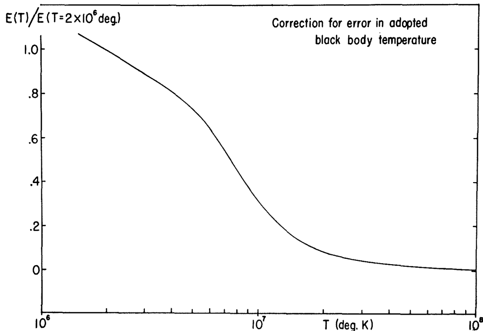
Fig. 1. If the true solar flux distribution with wavelength approximates a black-body curve for temperature T (abscissa), energy fluxes quoted in this paper must be multiplied by the value of the ordinate.
