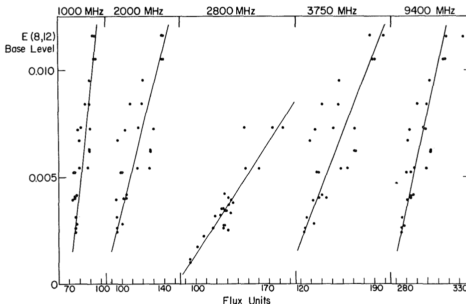
Fig. 3. Radio flux densities at 2800 MHz are those reported by Algonquin Radio Observatory (Ottawa) and at other frequencies are those reported by the Research Institute of Atmospheric at Nagoya University (Toyokawa). Radio and X-ray fluxes were observed simultaneously when no flares were occurring. The Toyokawa and Ottawa data represent samples during different months. One flux unit equals 10^{-22} \text{ W m}^{-2} \text{ Hz}^{-1} .
