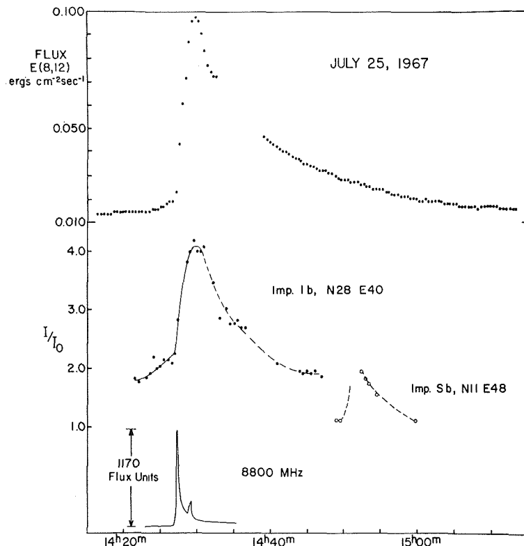
Fig. 6. The gap in the X-ray record (top) occurred during tape-recorder playback. Clouds interfered with the \text{H}\alpha flare observations (center). The 8800 MHz record was reported by Sagamore Hill (lower).
