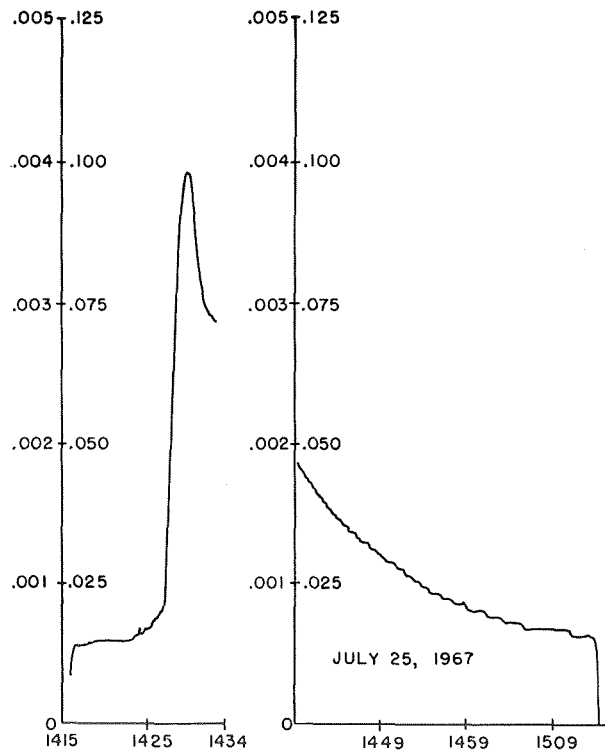
Fig. 7. A representative soft X-ray flux curve for an importance-1b flare (N28 E39) on July 25, 1967. Soft X-rays show early increase at 14 h 18 m . Low-sensitivity operation only. Sunrise and sunset at beginning and end of record.
