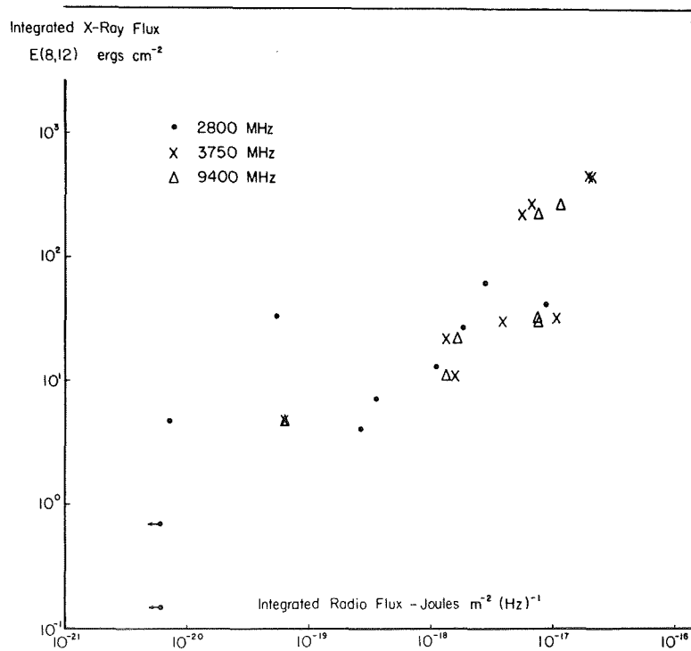
Fig. 9. Relation of time-integrals of X-ray and cm- \lambda events. The 2800 MHz point at 5.5 \times 10^{-20} Joules m -2 Hz -1 represents an event on July 11 which was not clearly flare-associated. The two 2800 MHz points towards lower left represent estimated upper limits based upon no report during observing hours. All values as measured at earth, uncorrected for earth's orbital eccentricity.
