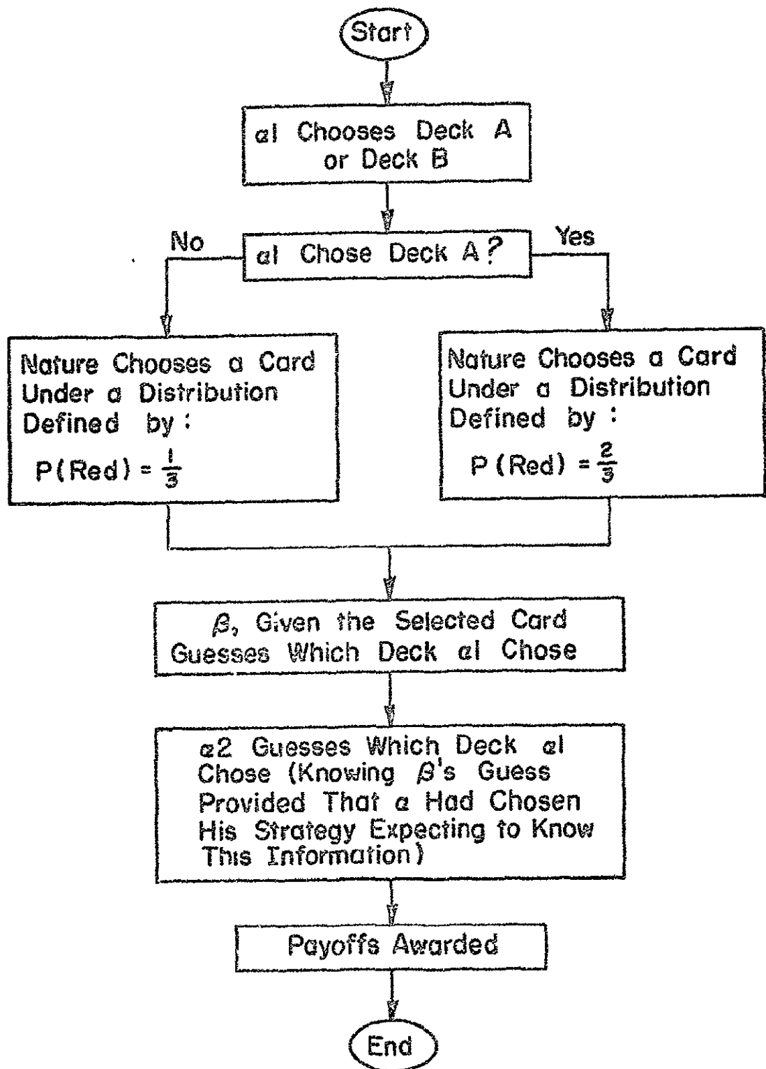
FIGURE 1. AN EXAMPLE OF A FINITE EXTENDED GAME.
