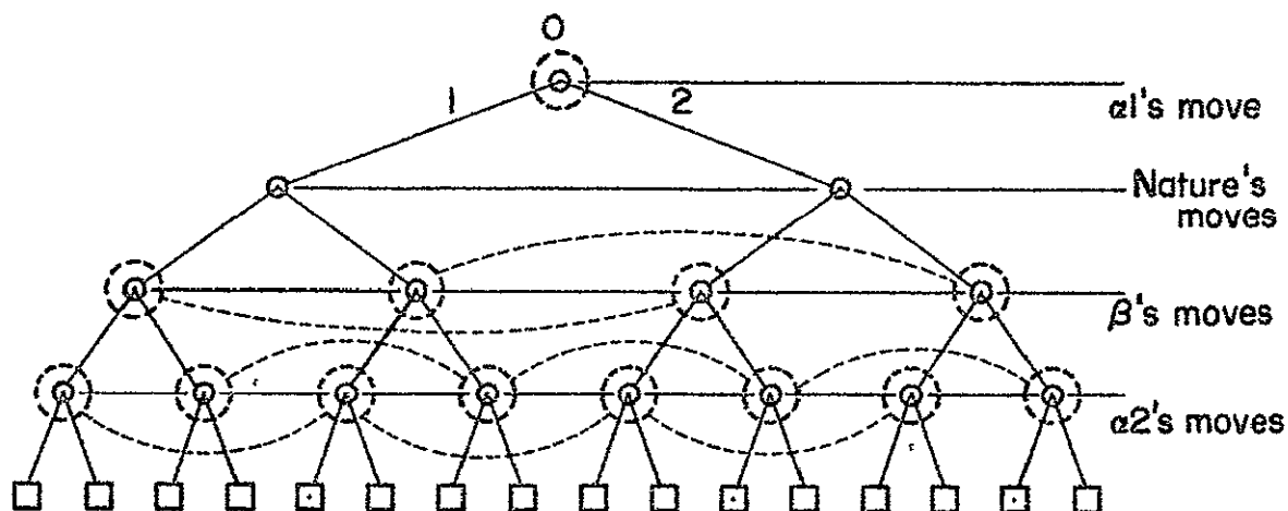
FIGURE 4(a) MOVE PARTITION DEFINING MAXIMUM GATHERABLE CHOICE INFORMATION FOR THE EXAMPLE GAME
