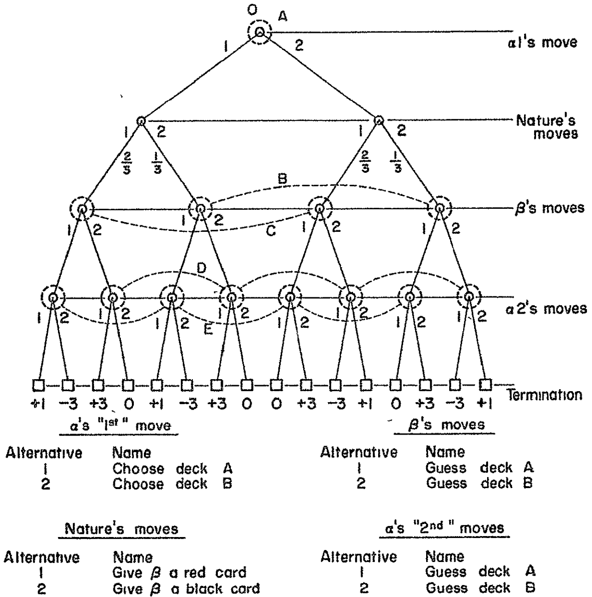
FIGURE 5. A COMPLETE DESCRIPTION OF THE EXAMPLE GAME.
