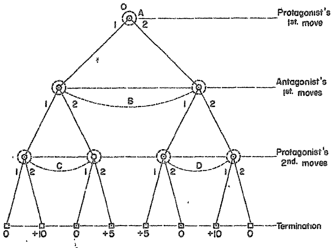
FIGURE 16. A GAME WITH AN INFORMATION COLLECTION SCHEME UPON WHICH A BEHAVIOR STRATEGY R-SOLUTION DOES NOT EXIST.
