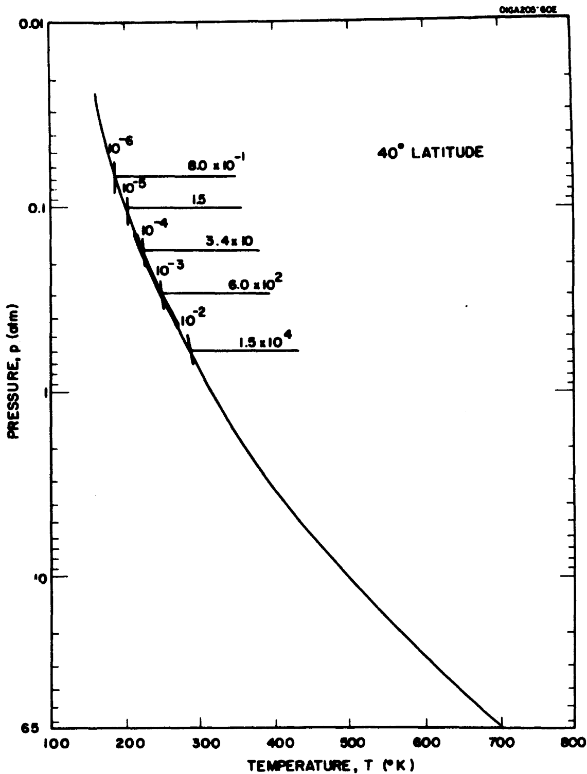
Figure 10. Thermal equilibrium temperature profile, saturation water vapor mixing ratios (labelled vertical lines), and integrated water vapor amounts above selected levels (numbers above horizontal lines with units of microns ( \mu ) of precipitable water) for 40° latitude on Venus. The 210°K to 270°K region of the temperature profile is emphasized by a thicker line.
