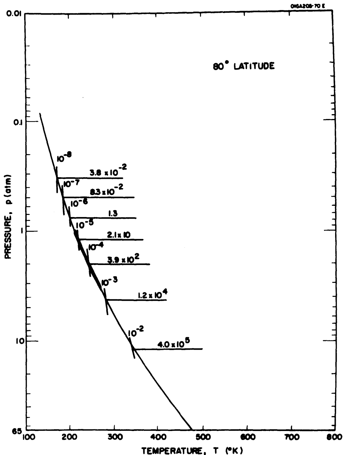
Figure 12. Thermal equilibrium temperature profile, saturation water vapor mixing ratios (labelled vertical lines), and integrated water vapor amounts above selected levels (numbers above horizontal lines with units of microns ( \mu ) of precipitable water) for 80° latitude on Venus. The 210°K to 270°K region of the temperature profile is emphasized by a thicker line.
