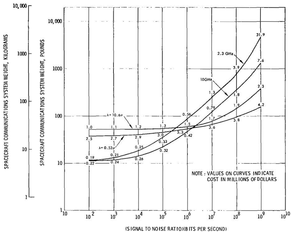
Figure B. Spaceborne Communications Systems Weight as a Function of Performance for Weight Optimized Systems Using 1980 State of the Art and a Mars Range, 10^8 Km
