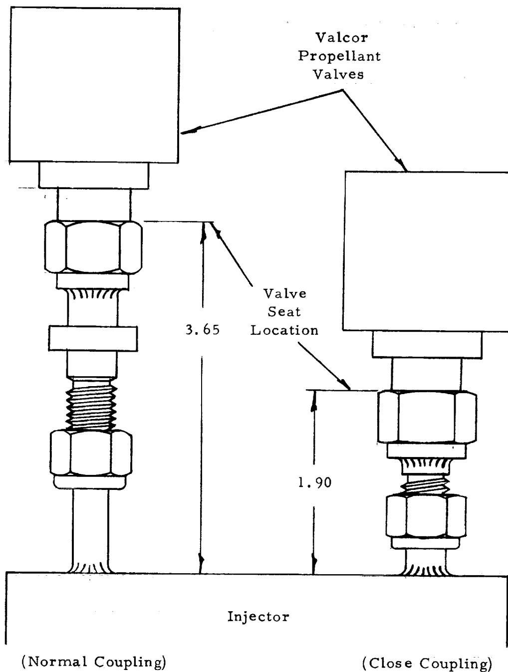
Figure 14. Sketches of Valve/Injector Coupling Configurations
