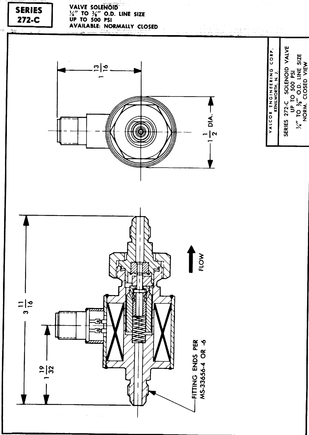
Figure 8. Drawing of Valcor Solenoid Valve Series 272-C
