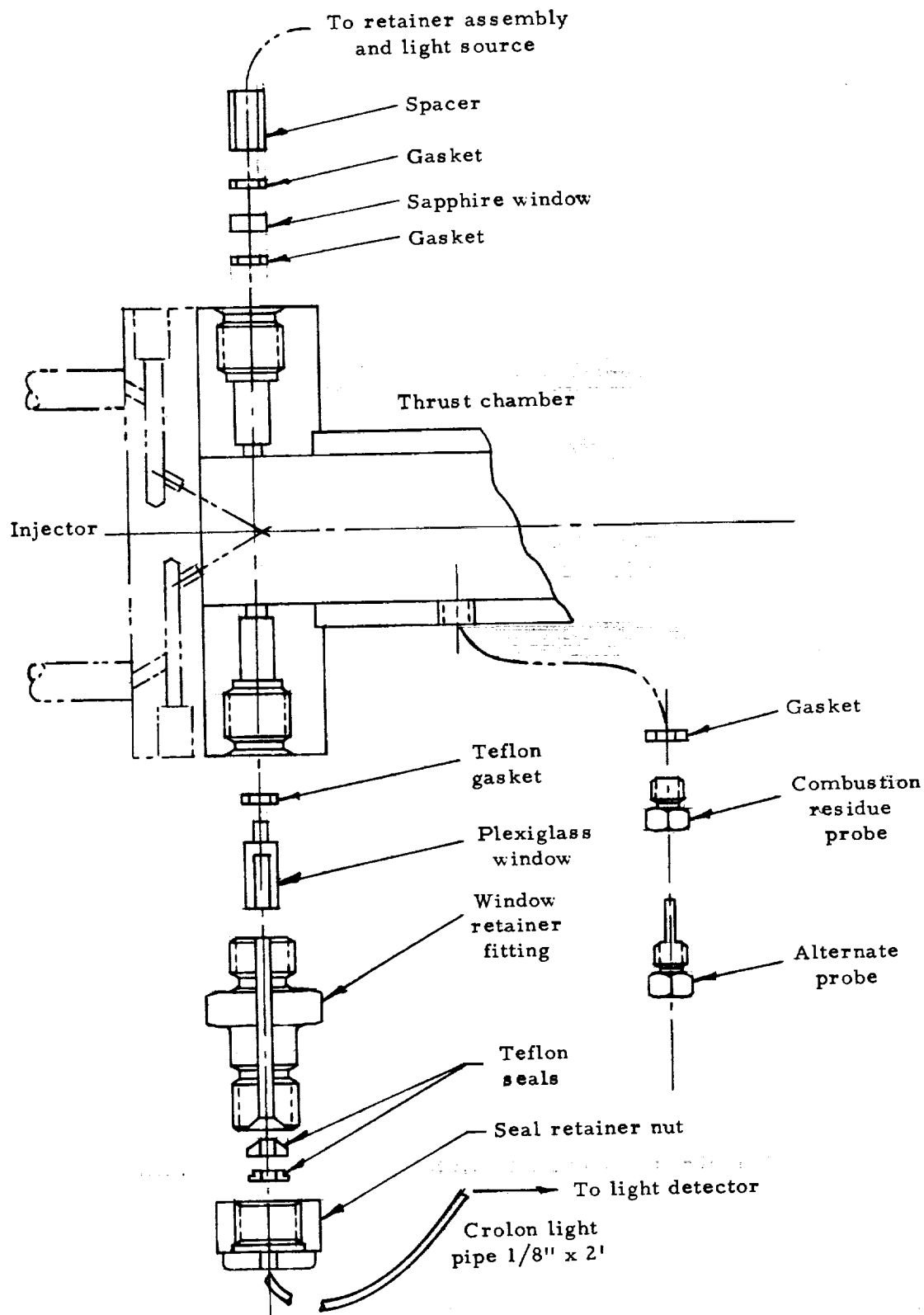
Figure 2. Sketch of Propellant Entry Detector Components and Residue Sampling Probes
