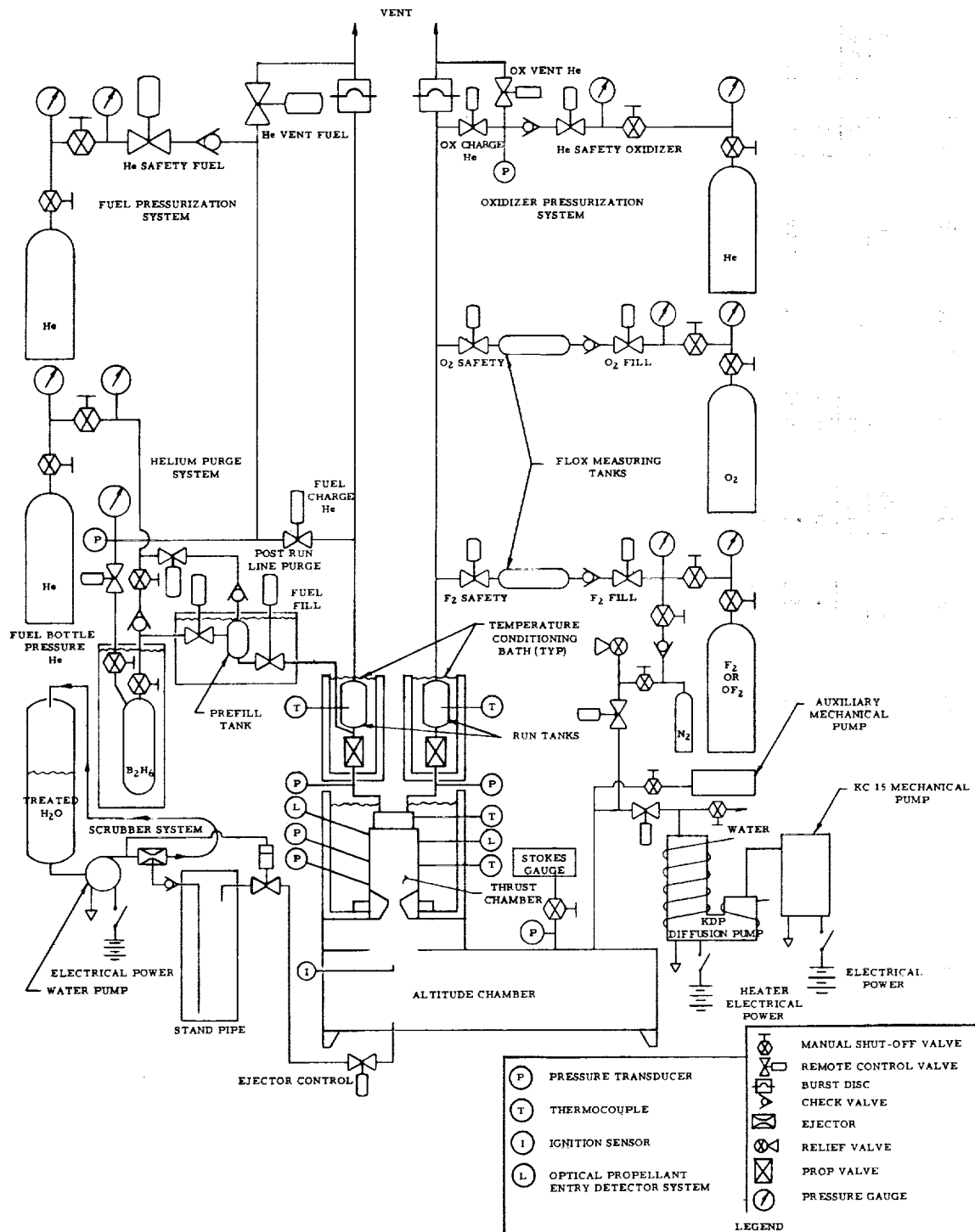
FIGURE 16. SCHEMATIC OF VACUUM IGNITION TEST SYSTEM FOR PHASE II PROGRAM
