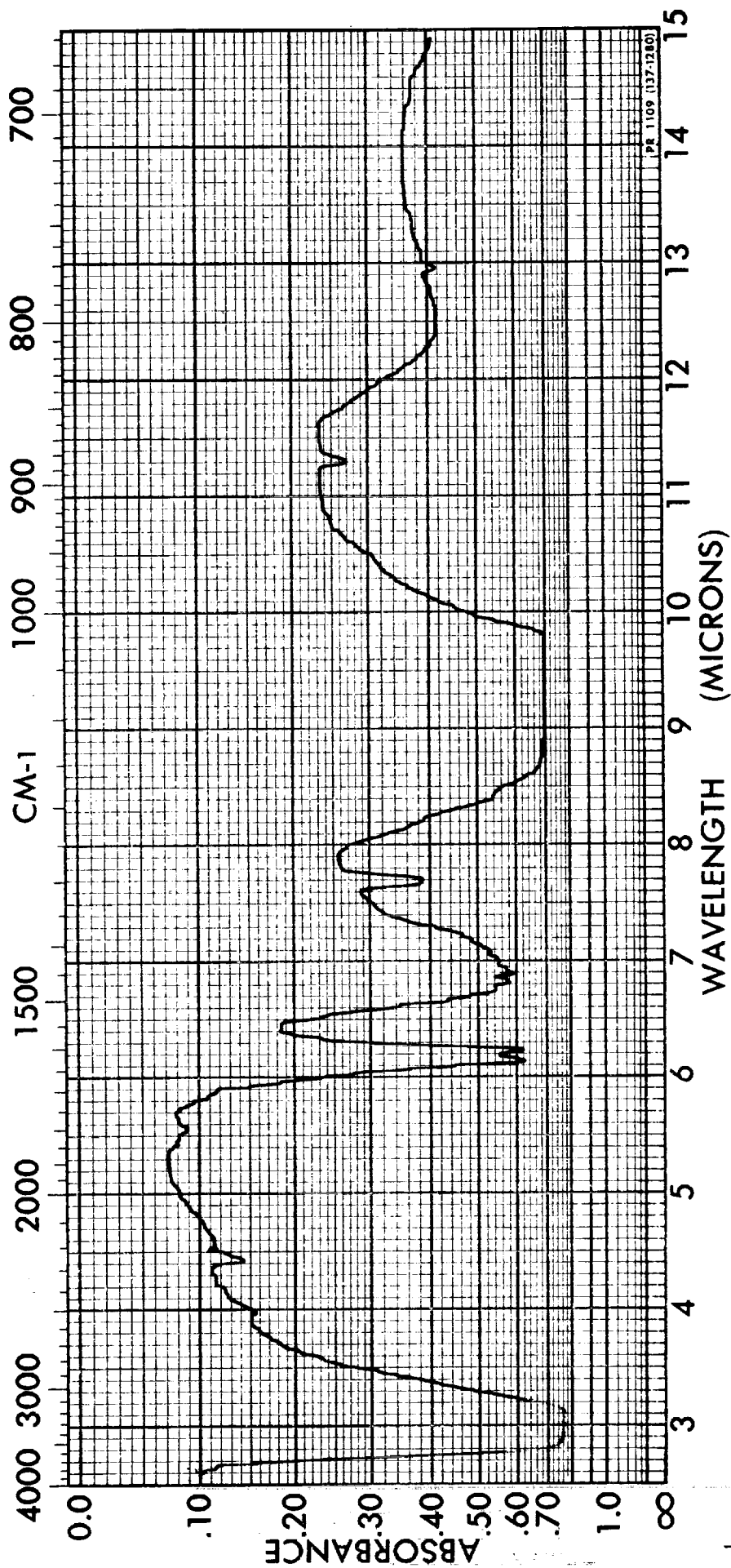
Figure 23. IR Spectrum of Black Powder Residue from OF 2 /B 2 H 6 Run 108. (High Concentration in KBr Pellet)
