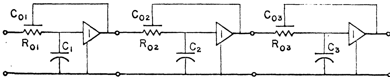
Fig. 5 Complex Optimization Example Problem
