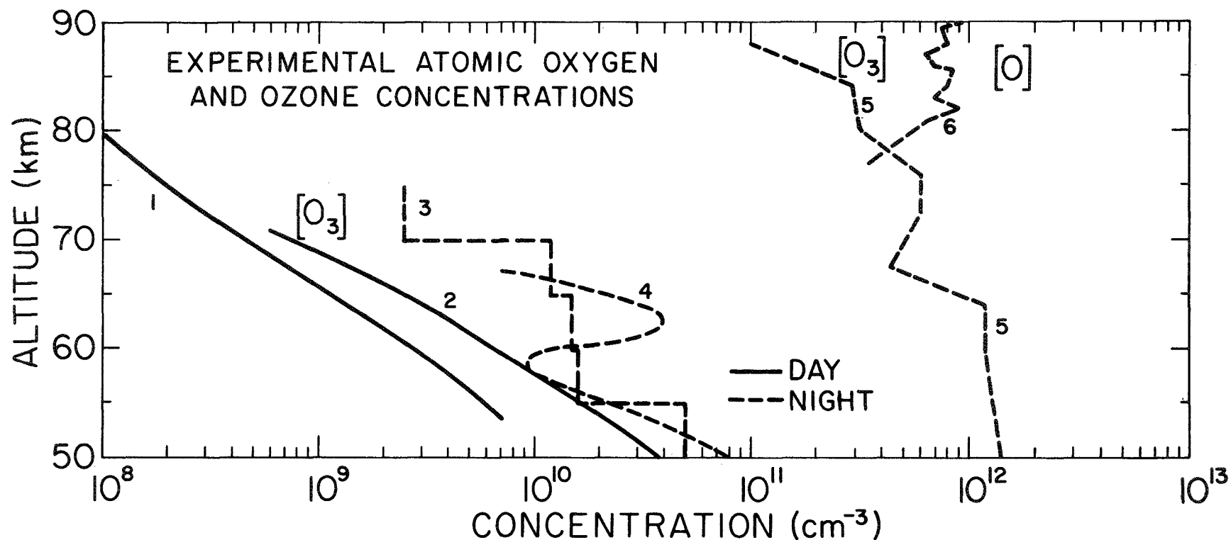
Figure 2. Experimental profiles of atomic oxygen and ozone concentrations. 1. Daytime ozone concentration by Johnson, et al. (1954); 2. Daytime ozone concentration by Rawcliffe, et al. (1963); 3. Nighttime ozone concentration by Carver, et al. (1966); 4. Nighttime ozone concentration by Reed (1968); 5. Nighttime ozone concentration by Mikirov (1965) and 6. Atomic oxygen nighttime concentration by Fedynskii, et al. (1967).
