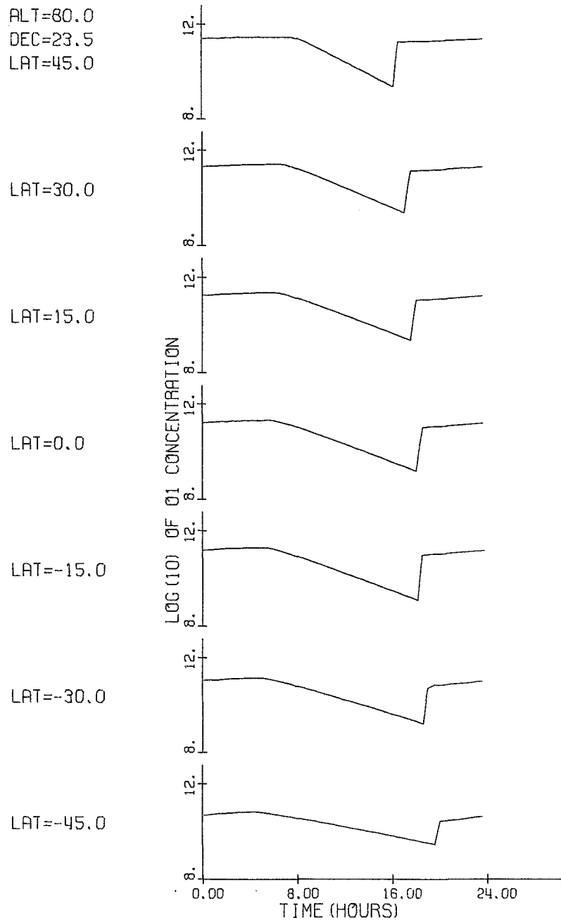
Figure 8. Theoretical values of diurnal latitudinal and seasonal variation of atomic oxygen and ozone for an oxygen alone atmosphere (80 km).
