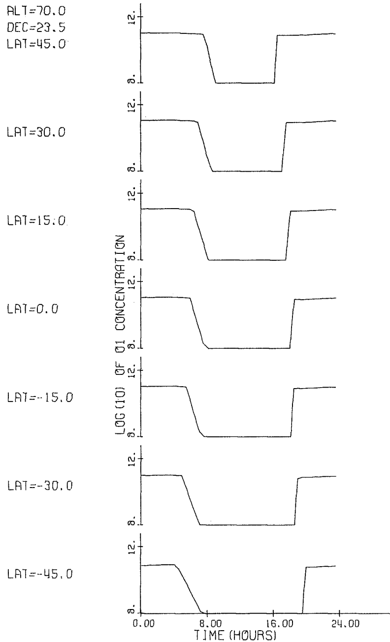
Figure 7. Theoretical values of diurnal latitudinal and seasonal variation of atomic oxygen and ozone for an oxygen alone atmosphere (70 km).
