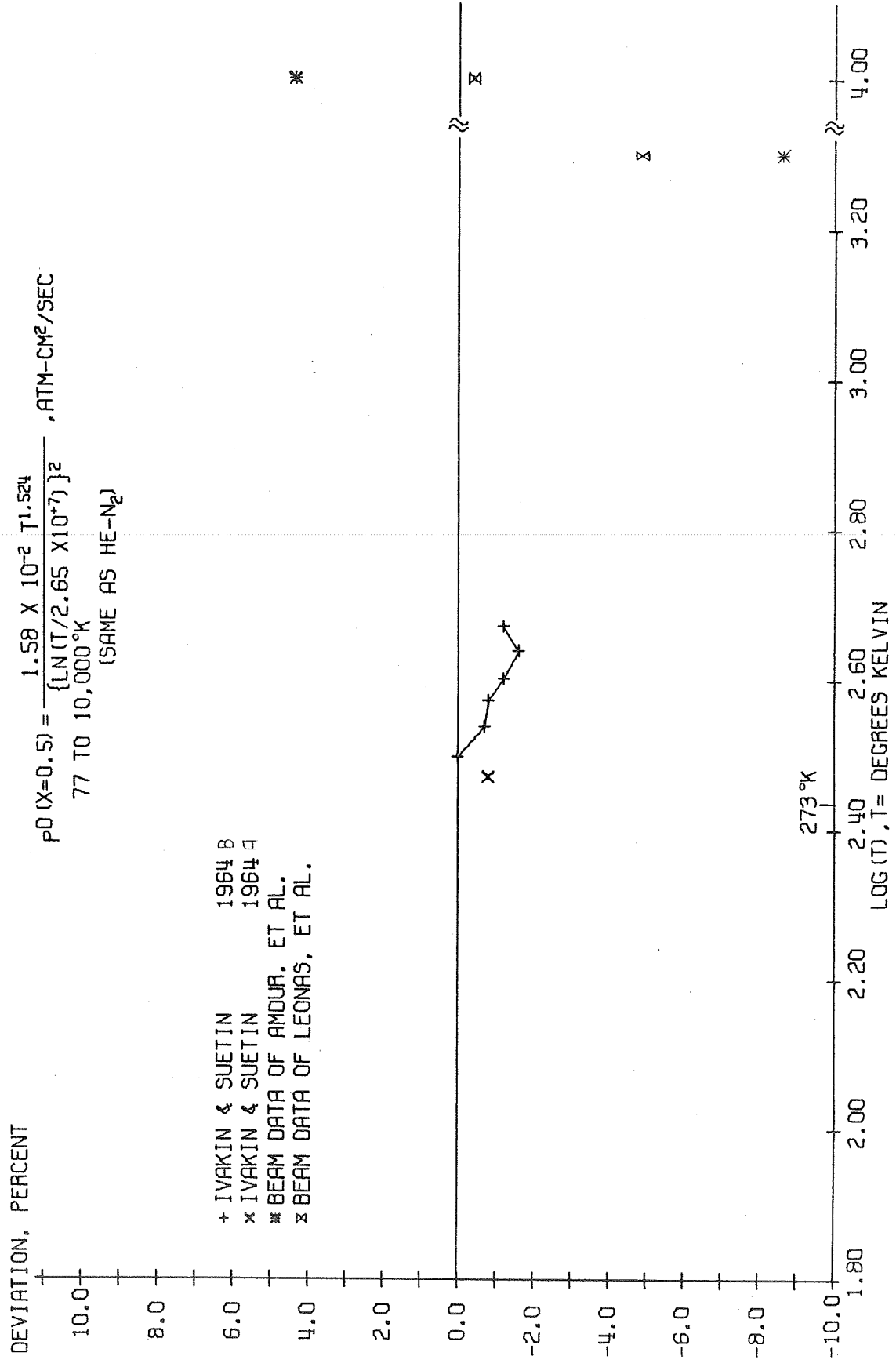
FIG. 25. DEVIATIONS OF DIFFUSION COEFFICIENTS FROM REFERENCE EQUATION, HELIUM - CARBON MONOXIDE
