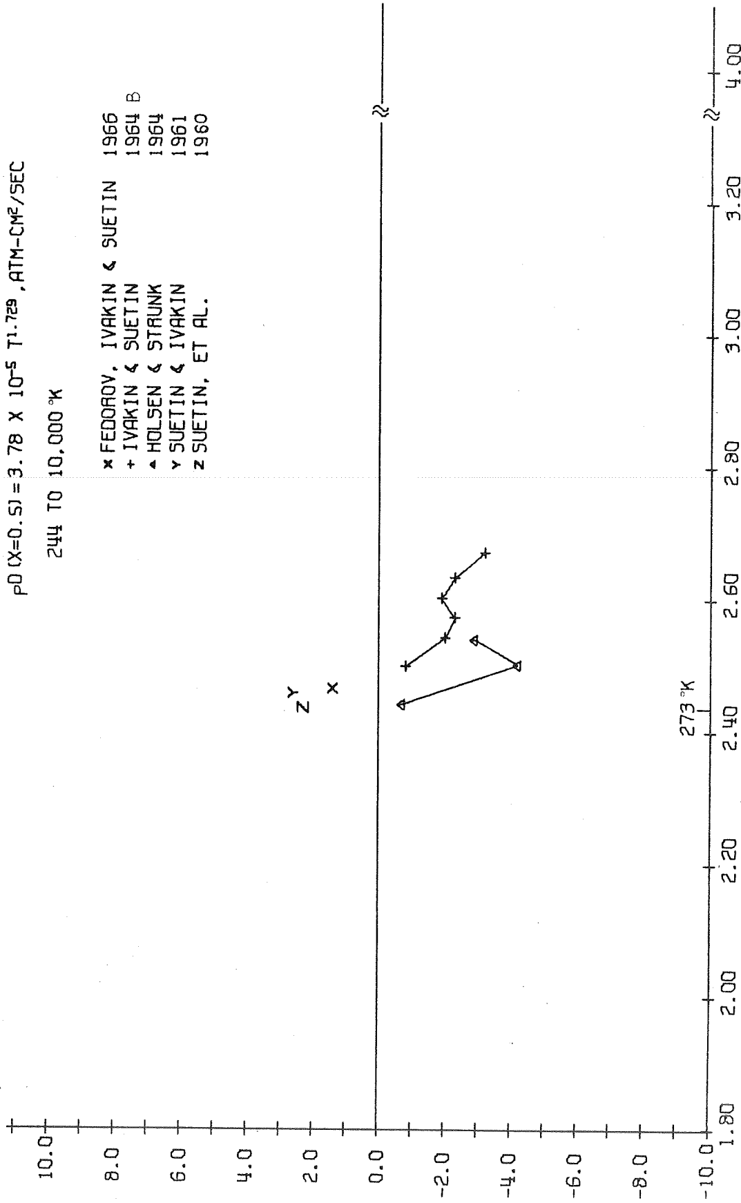
FIG. 27. DEVIATIONS OF DIFFUSION COEFFICIENTS FROM REFERENCE EQUATION, HELIUM - AIR
