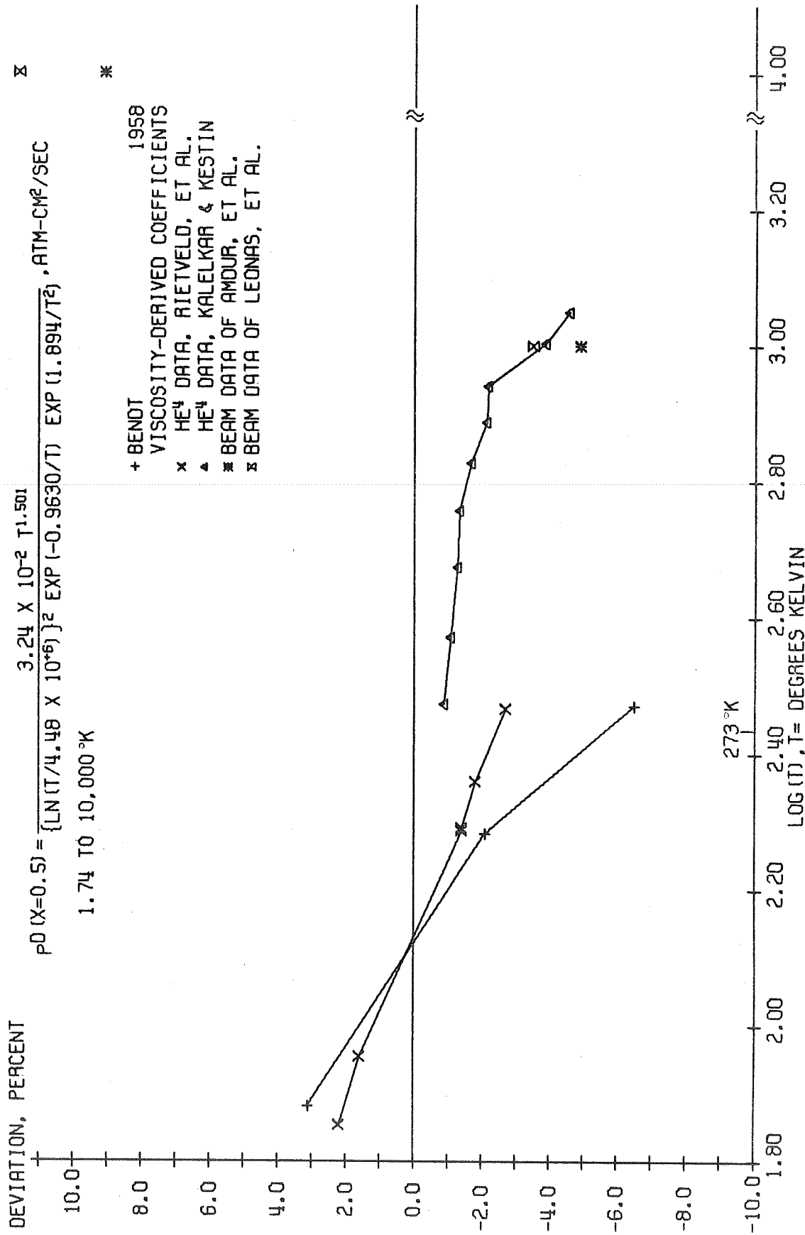
FIG. 22. DEVIATIONS OF DIFFUSION COEFFICIENTS FROM REFERENCE EQUATION, HELIUM-3 - HELIUM-4
