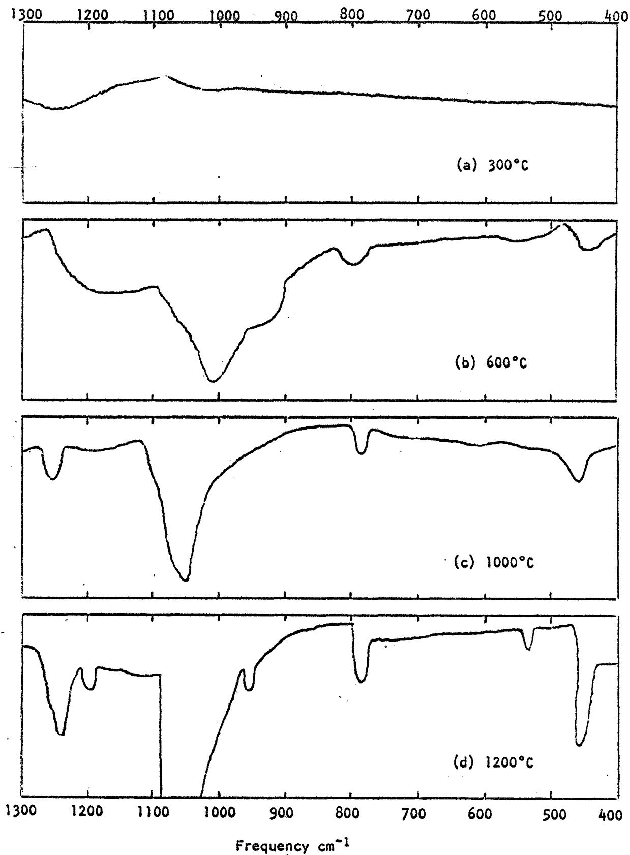
Figure 1Q. Infrared Spectra of Oxide Grown on \text{TiSi}_2 at 300-1200°C
