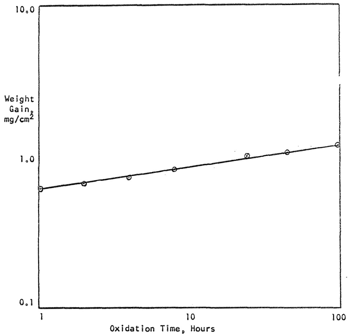
Figure 17 Oxidation Weight Gain Data for \text{Ti}_5\text{Si}_3
