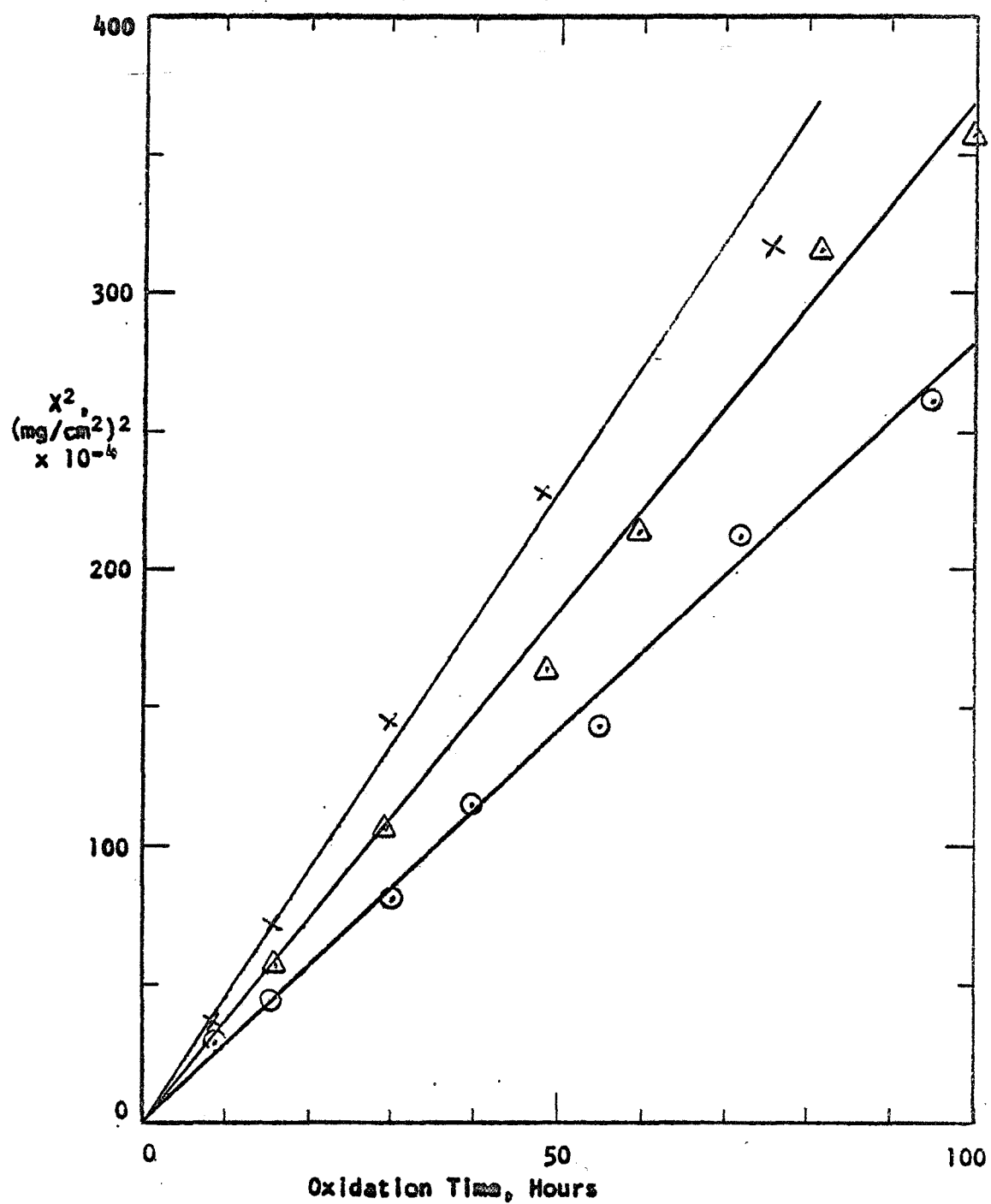
Figure 13. X^2 versus t for \text{TiSi}_2 Oxidized at 1000^\circ\text{C}
