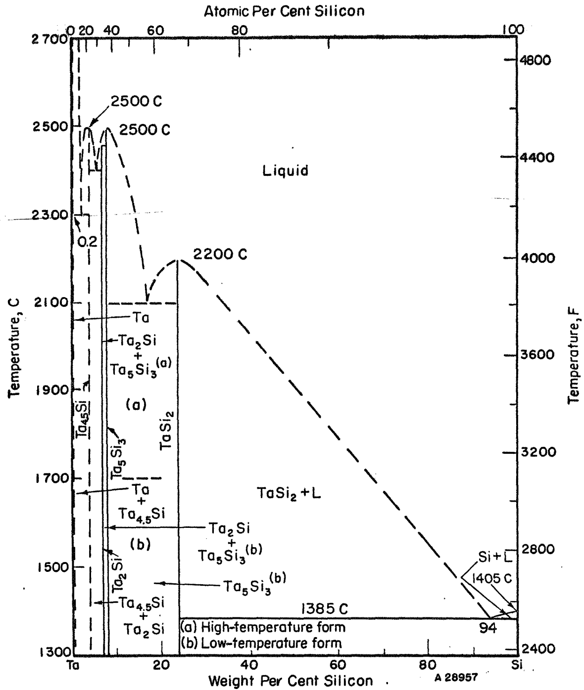
FIGURE 2 Ta-Si PHASE DIAGRAM (30)
