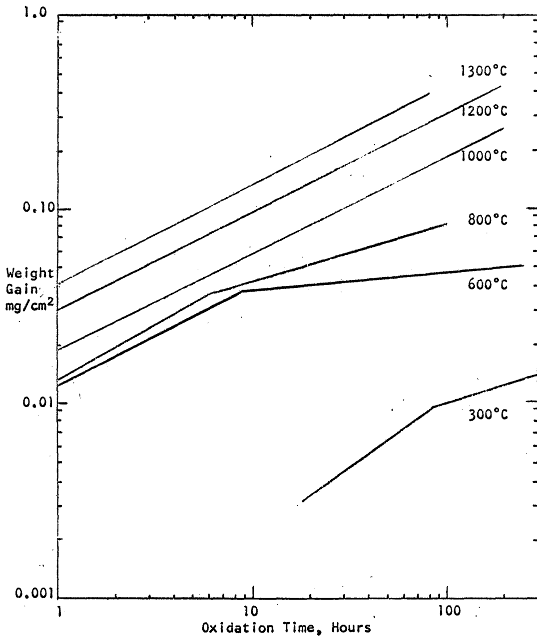
Figure 14. Summary of \text{TiSi}_2 Oxidation Rate Data: 300-1300°C
