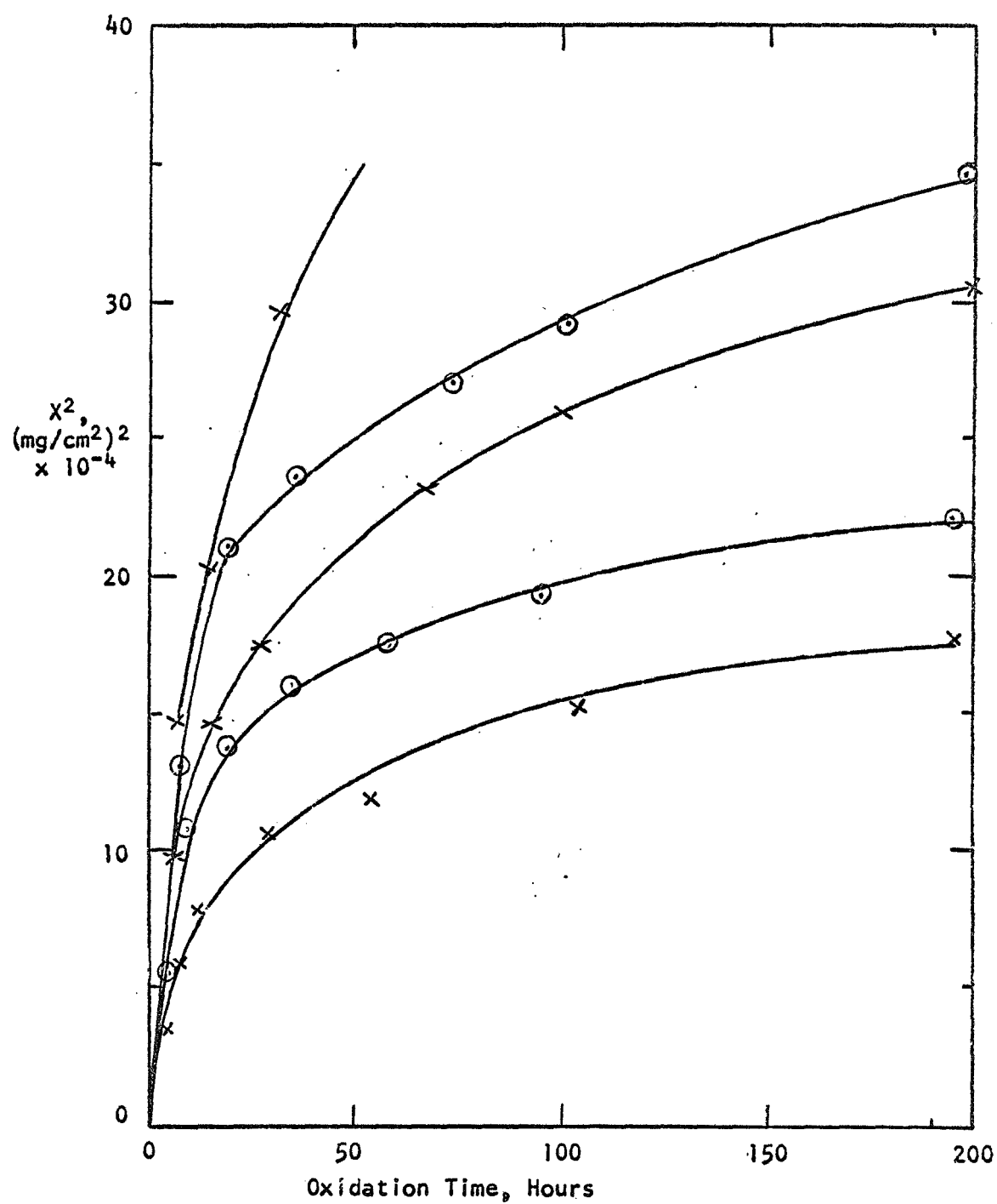
Figure 12. X^2 versus t for \text{TiSi}_2 Oxidized at 600^\circ\text{C}
