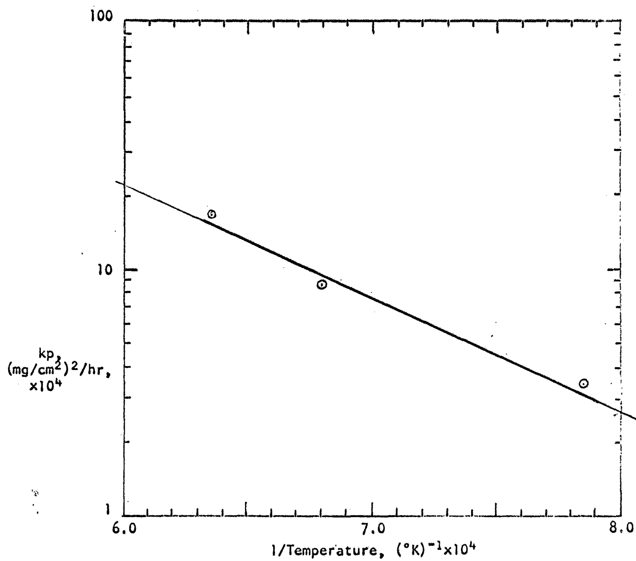
Figure 15. Arrhenius Plot of \text{TiSi}_2 Oxidation Data
