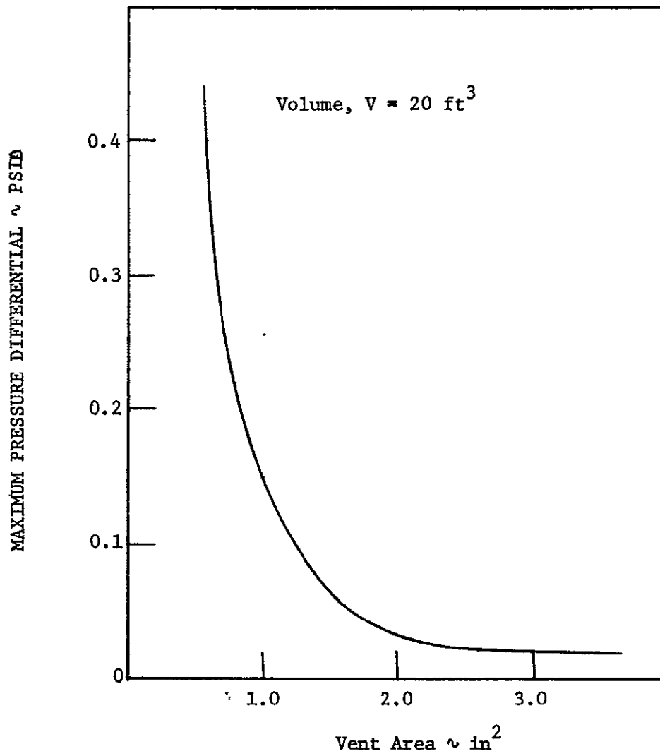
FIGURE B-2 MAXIMUM DIFFERENTIAL PRESSURE VERSUS VENT AREA, V = 20 \text{ FT}^3
