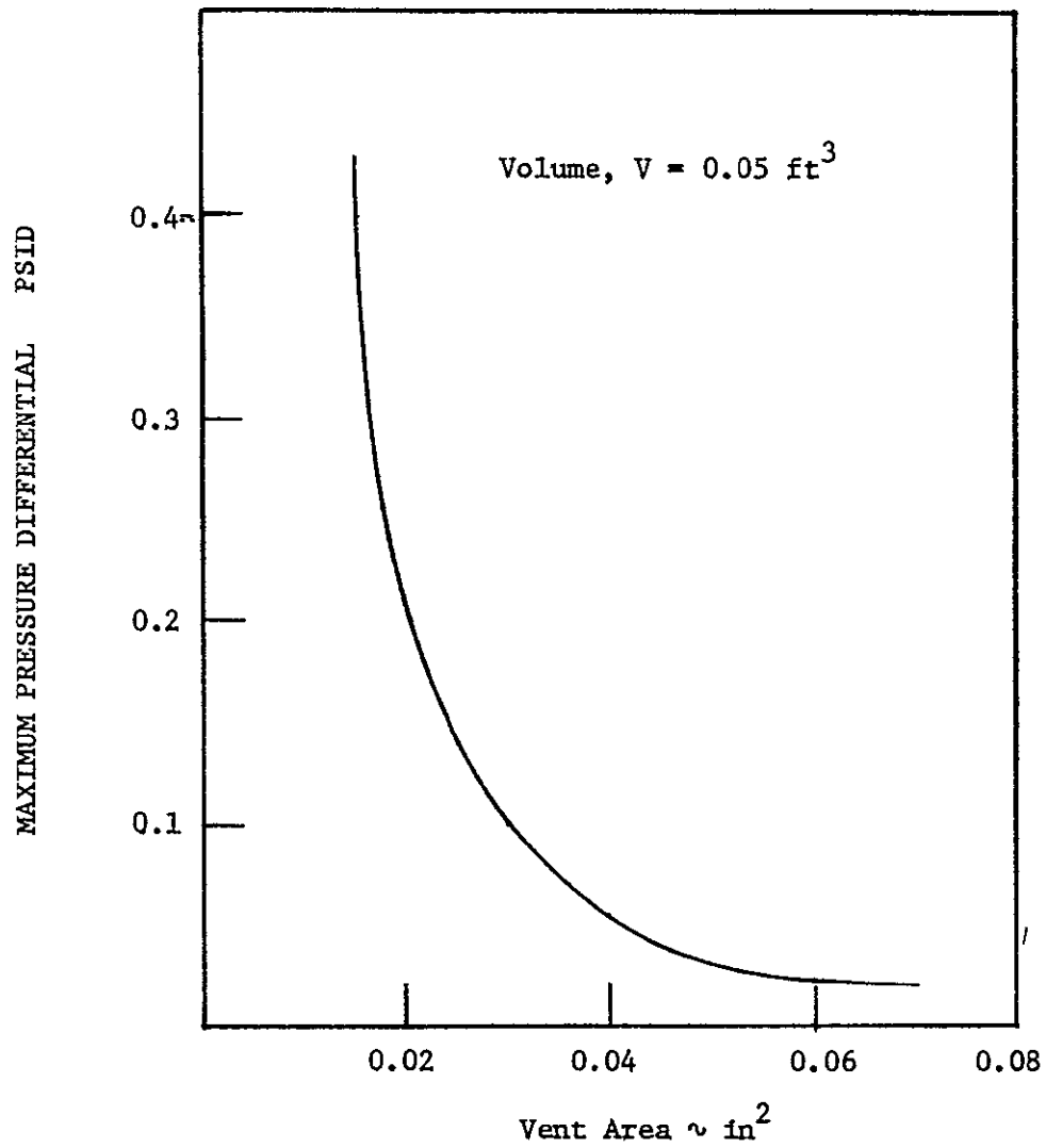
FIGURE B-3 MAXIMUM DIFFERENTIAL PRESSURE VERSUS VENT AREA, V = 0.05 FT³
