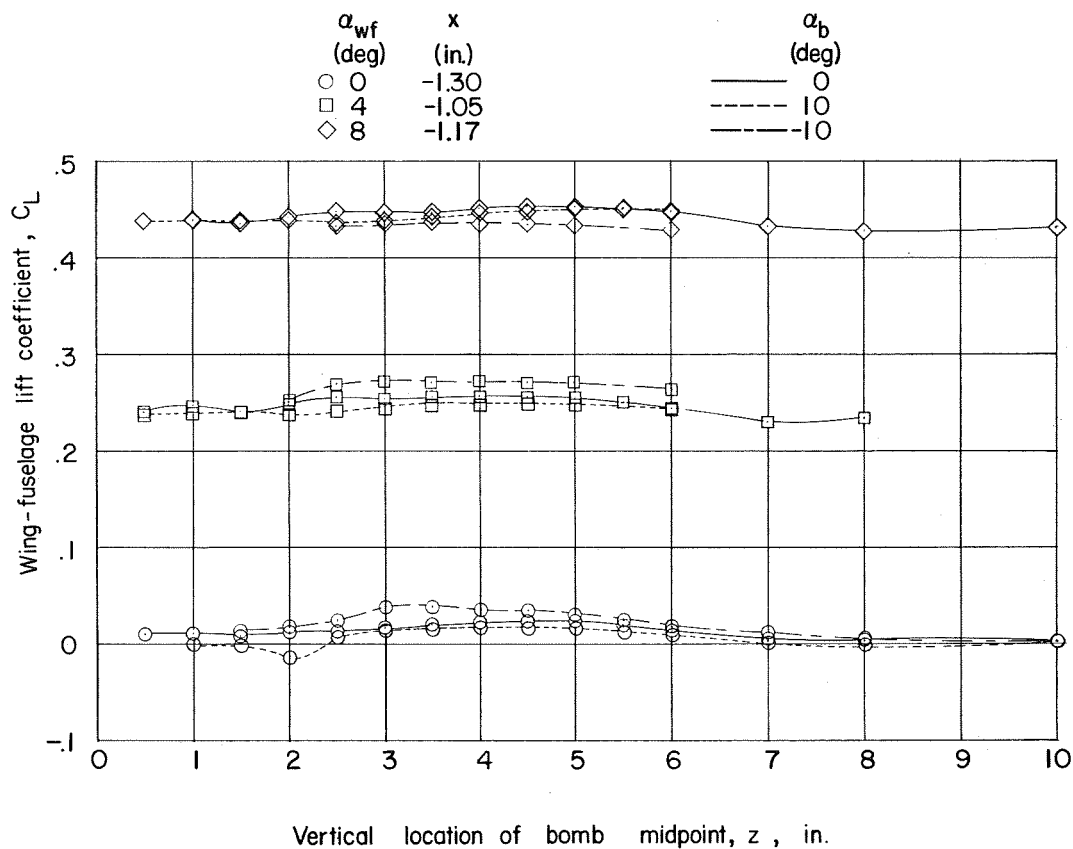
(a) Lift.
