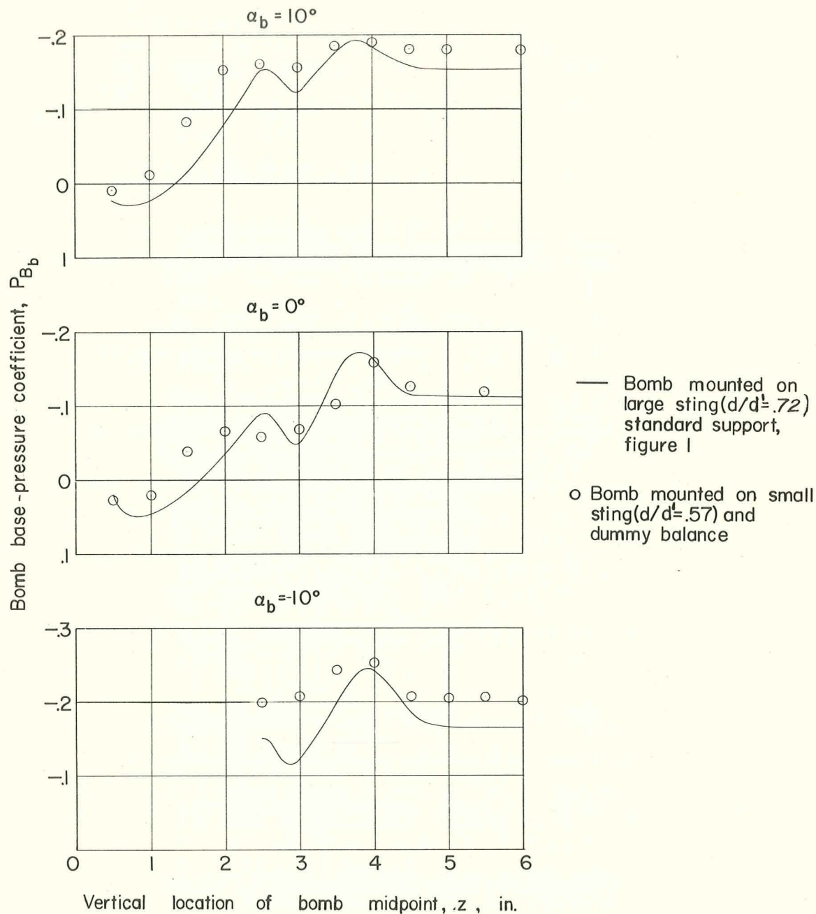
Figure 5.- Comparison of bomb base pressures measured with support stings of large and small diameters. x = -2.55 inches; \alpha_{wf} = 4^\circ ; bomb 2.
