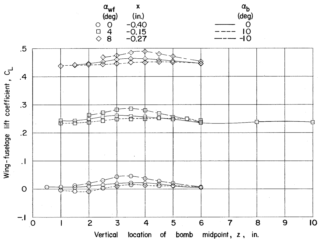
(a) Lift.
