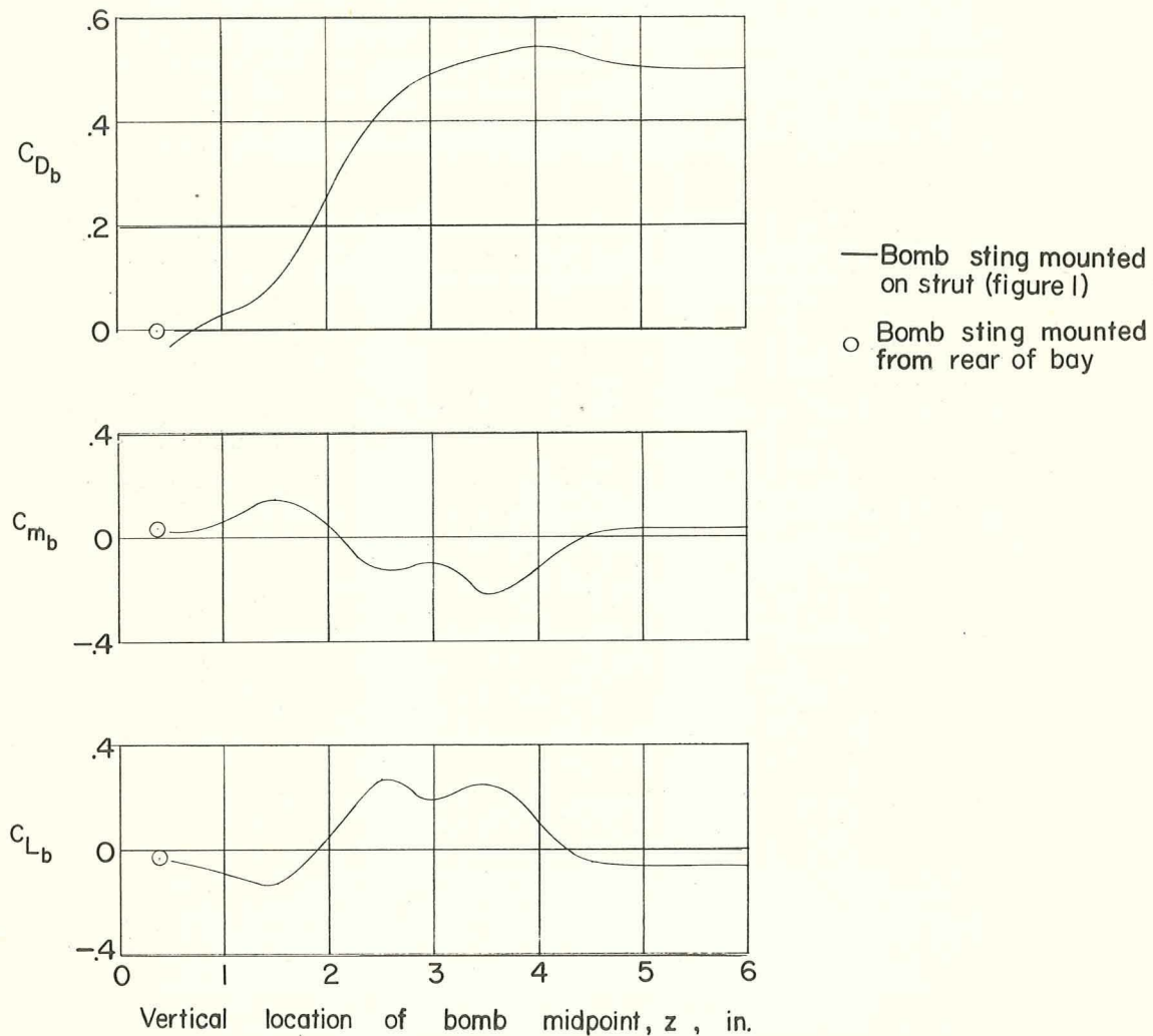
Figure 4.- Comparison of forces measured on bomb with and without bomb-support strut. Bomb 2; large fins; x = 0.95 inch; \alpha_{wf} = 0^\circ ; \alpha_b = 0^\circ .
