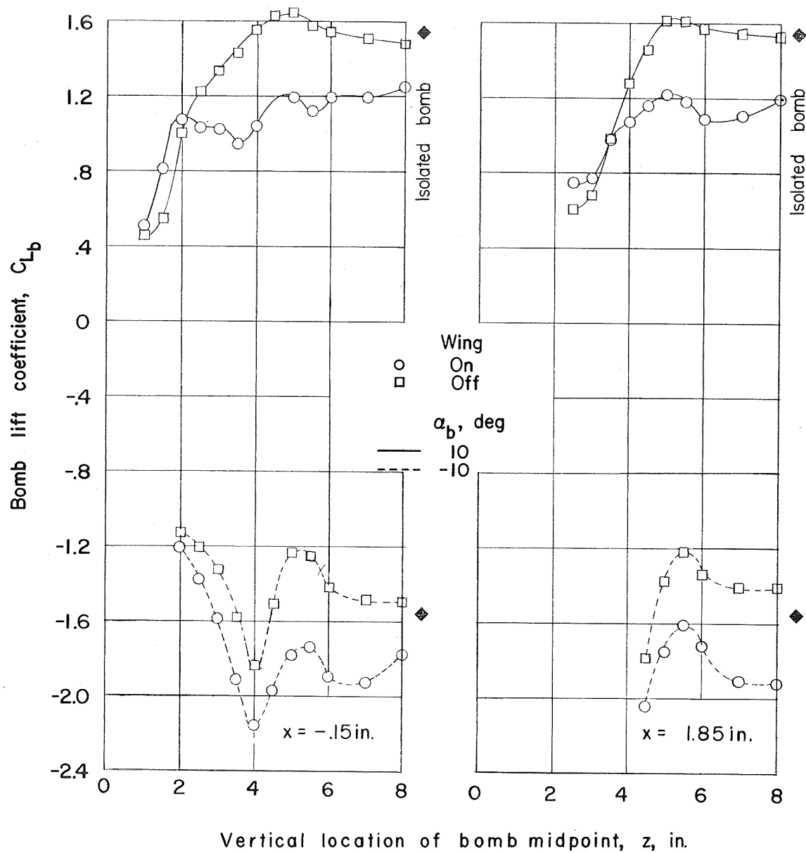
(a) Lift.
