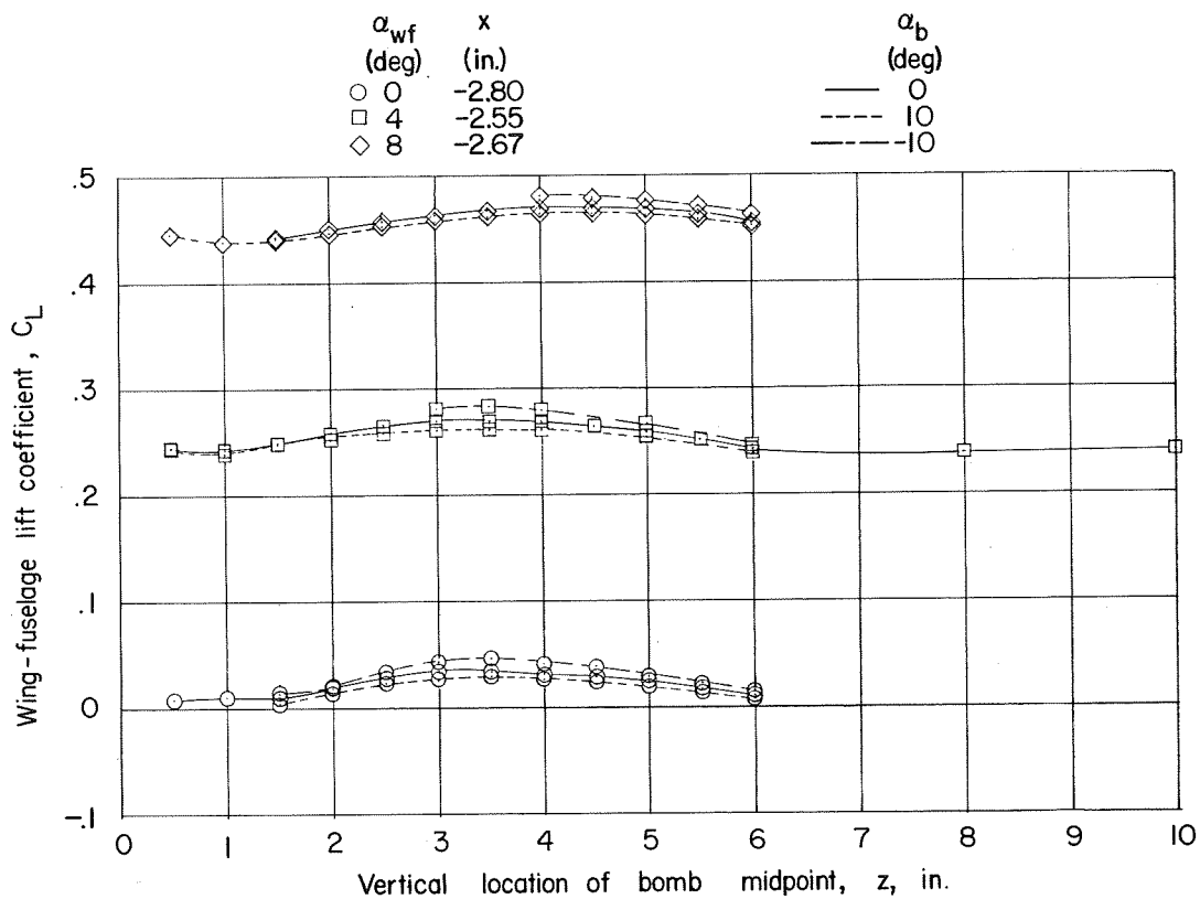
(a) Lift.
