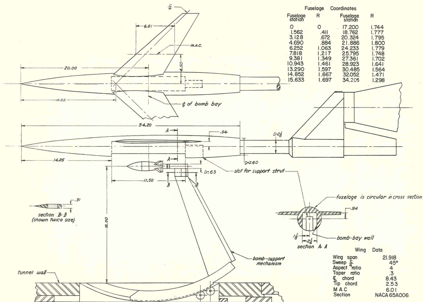
(a) Dimensions of components. All dimensions are in inches.
