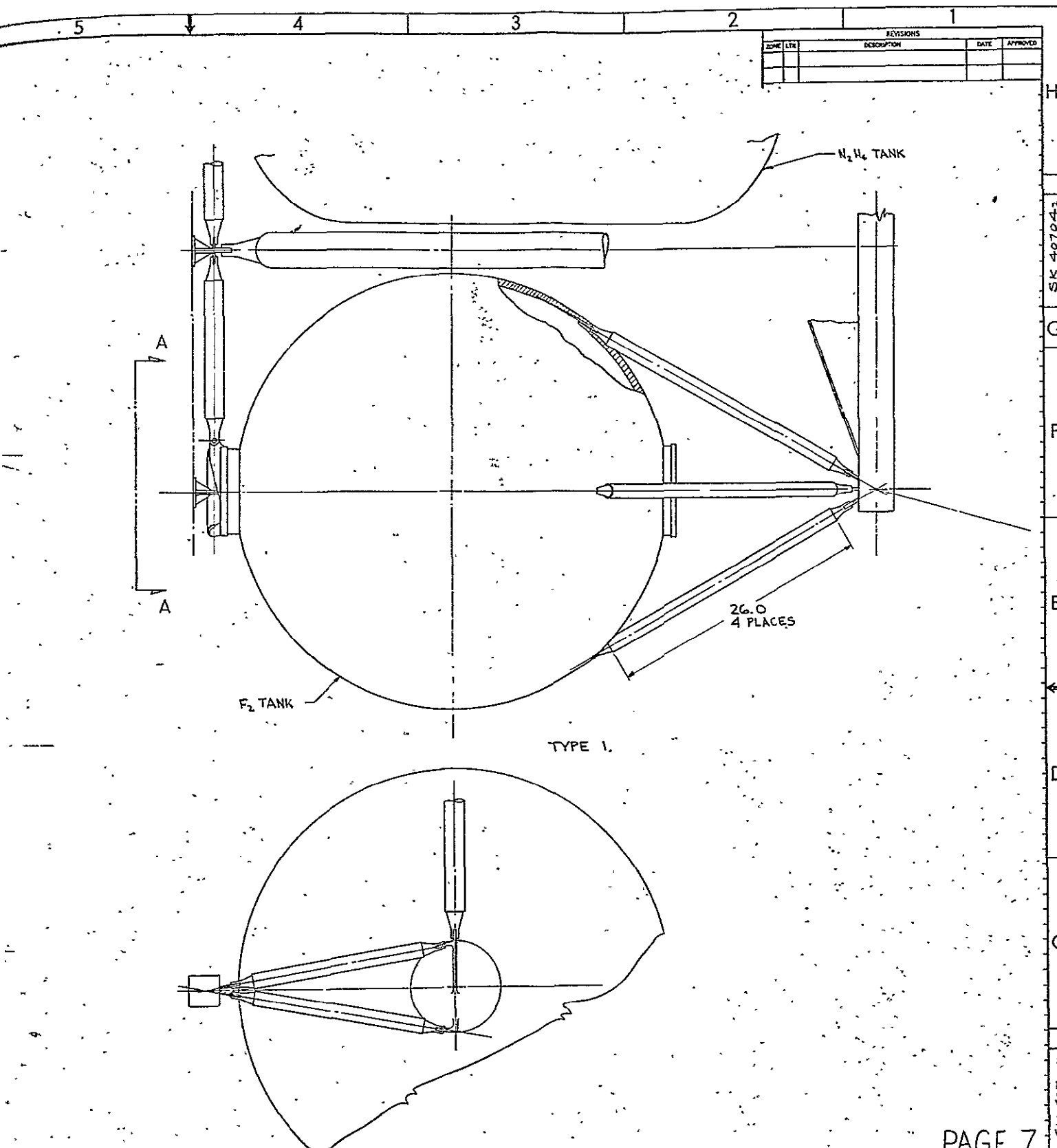
VIEW A-A TORSION TUBE LAYOUT (TYP)
