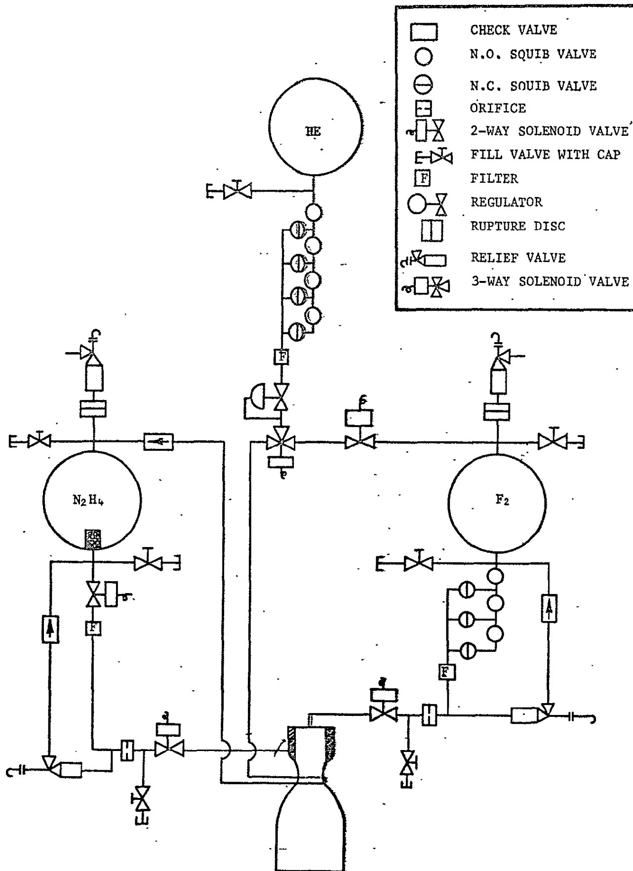
FIGURE 3-1. SCHEMATIC DIAGRAM OF F_2/N_2H_4 SPACECRAFT PROPULSION SYSTEM
