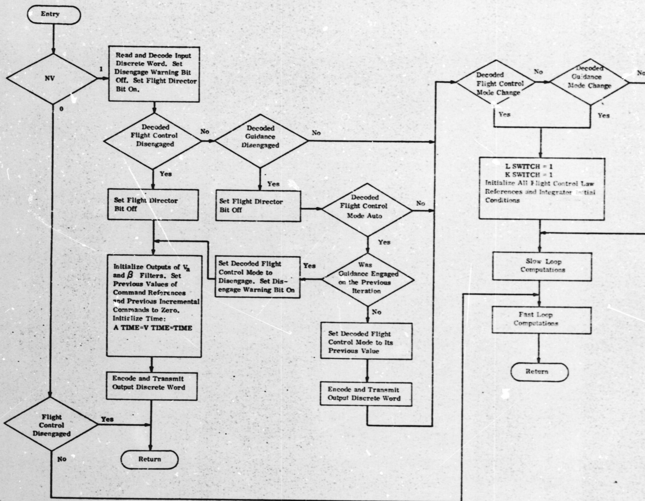
Figure 3. Flight Control Subroutine
