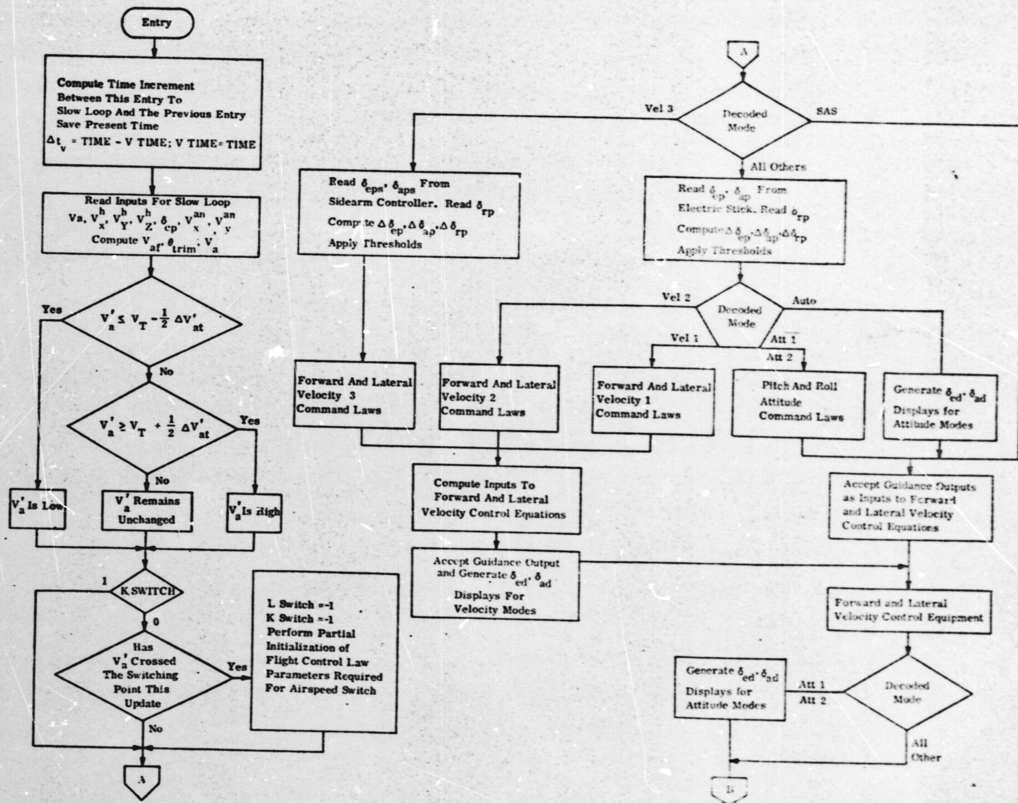
Figure 4. Slow Loop (Sheet 1 of 2)
