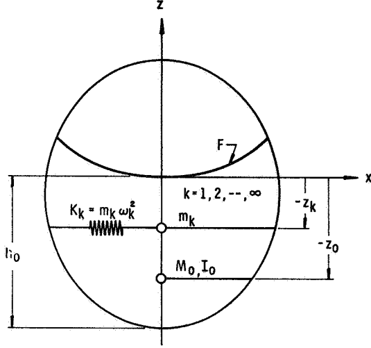
Fig. 2 Equivalent mechanical model
