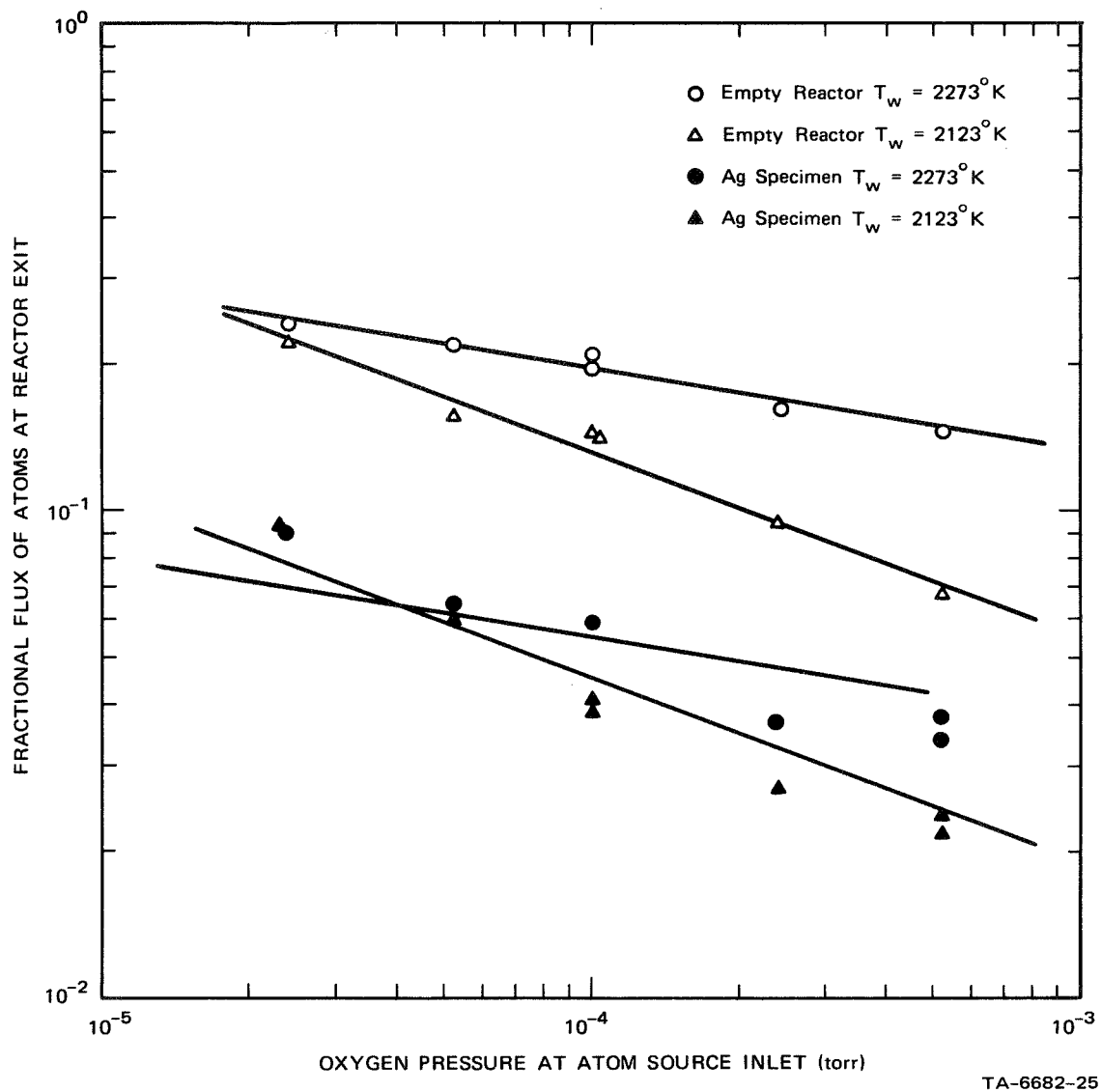
FIGURE 13 FRACTIONAL OXYGEN ATOM FLUX AT REACTOR EXIT AS A FUNCTION OF ATOM SOURCE TEMPERATURE, T_w , AND PRESSURE.
