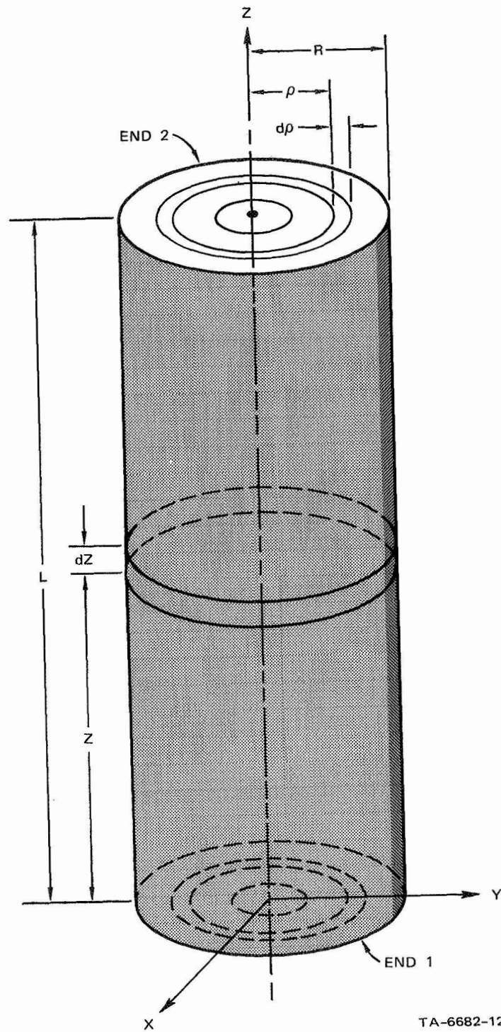
FIGURE 2 REACTOR MODEL
