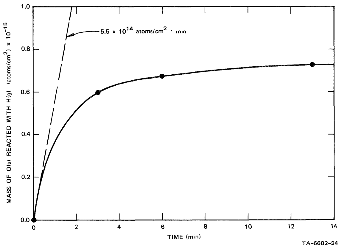
FIGURE 21 RATE OF REACTION OF GASEOUS ATOMIC HYDROGEN WITH OXYGEN ADATOMS ON GOLD AT 300°K. P_H \cong 3 \times 10^{-9} torr. At time = 0, gold surface coverage with oxygen \theta_N = 1.07 \times 10^{15} atoms/cm 2 .
