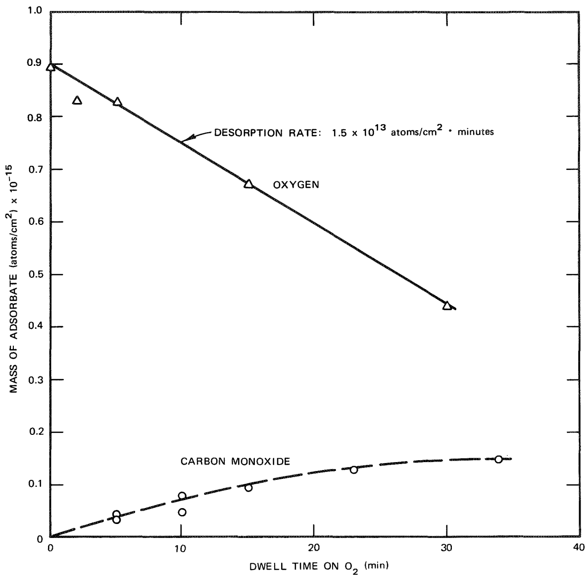
FIGURE 10 SPONTANEOUS DESORPTION OF OXYGEN FROM GOLD AT 300°K. At time = 0, gold surface was covered with approximately 1 \times 10^{15} adatoms/cm 2 . P_{O_2} \cong 5 \times 10^{-5} torr. Rate of adsorption of CO is shown by dashed curve. P_{CO} \cong 5 \times 10^{-6} torr.
