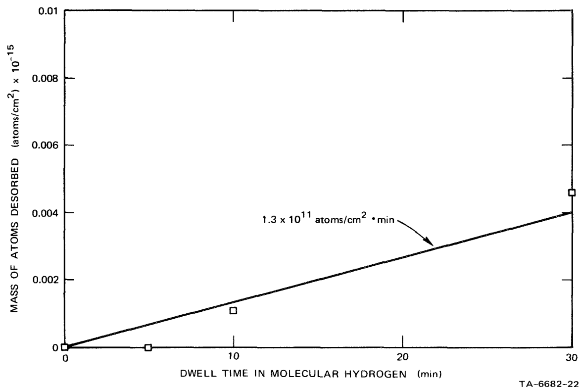
FIGURE 19 SPONTANEOUS DESORPTION OF HYDROGEN ADATOMS FROM GOLD AT 300°K. Initial coverage at time 0 = 0.016 \times 10^{15} atoms/cm 2 .
