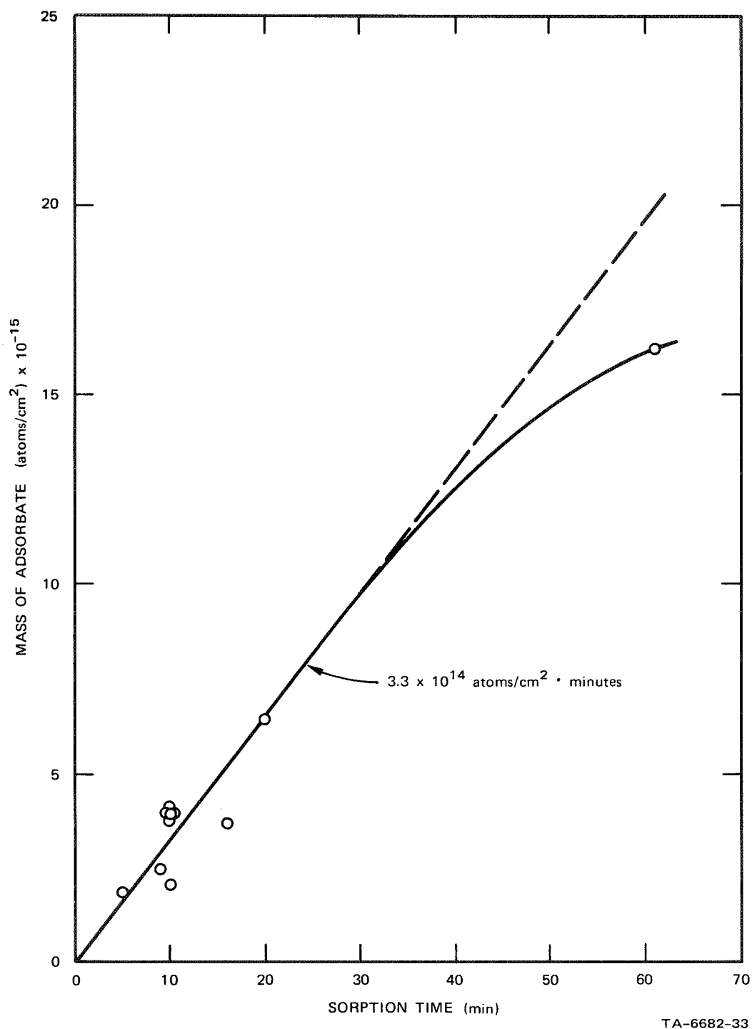
FIGURE 11 ADSORPTION/OCCLUSION OF OXYGEN ATOMS BY SILVER AT 300°K. P_{\text{O}} \cong 1.4 \times 10^{-7} torr.
