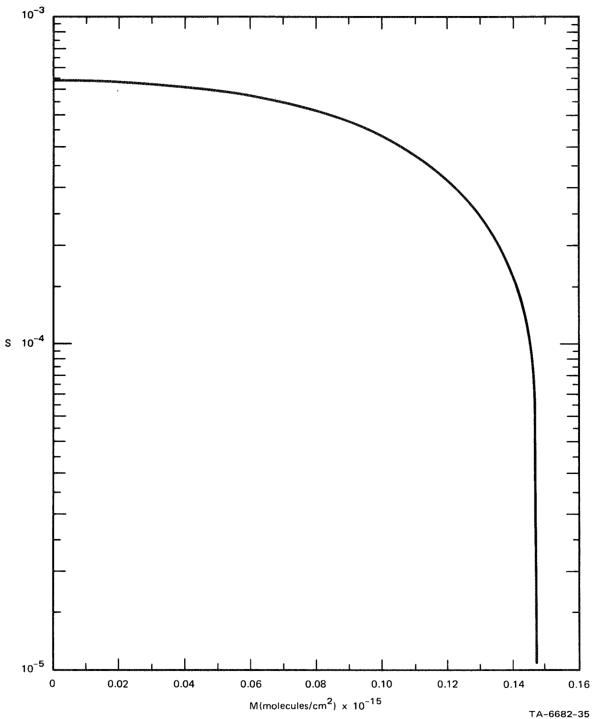
FIGURE 22 STICKING COEFFICIENT OF CO ON GOLD AT 300°K. P_{\text{CO}} \cong 5 \times 10^{-6} torr.
