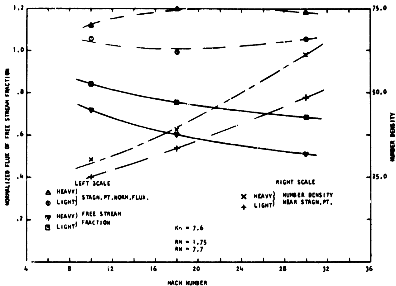
Figure 22. Variation of Stagnation Point Conditions with Mach Number of the Flow, Data is from Run No. M2, M8, and M9
