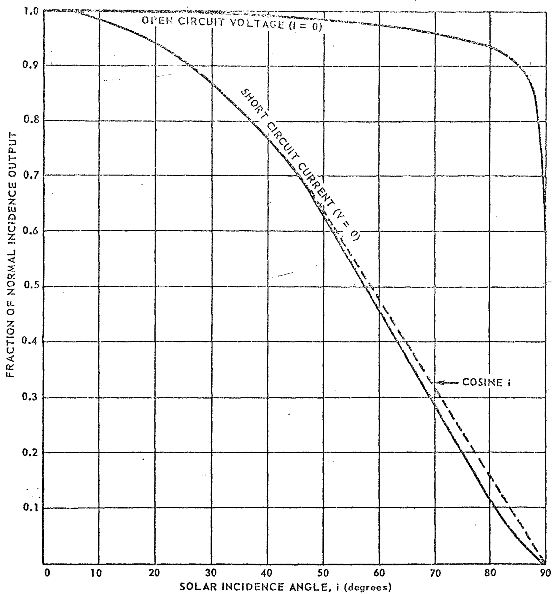
Fig. 3 NORMALIZED SOLAR CELL ELECTRICAL OUTPUT AS A FUNCTION OF SOLAR INCIDENCE ANGLE (Corning 0211 Microsheet - 0.006 Inch OCL Blue Filter and Antireflective Coating)
