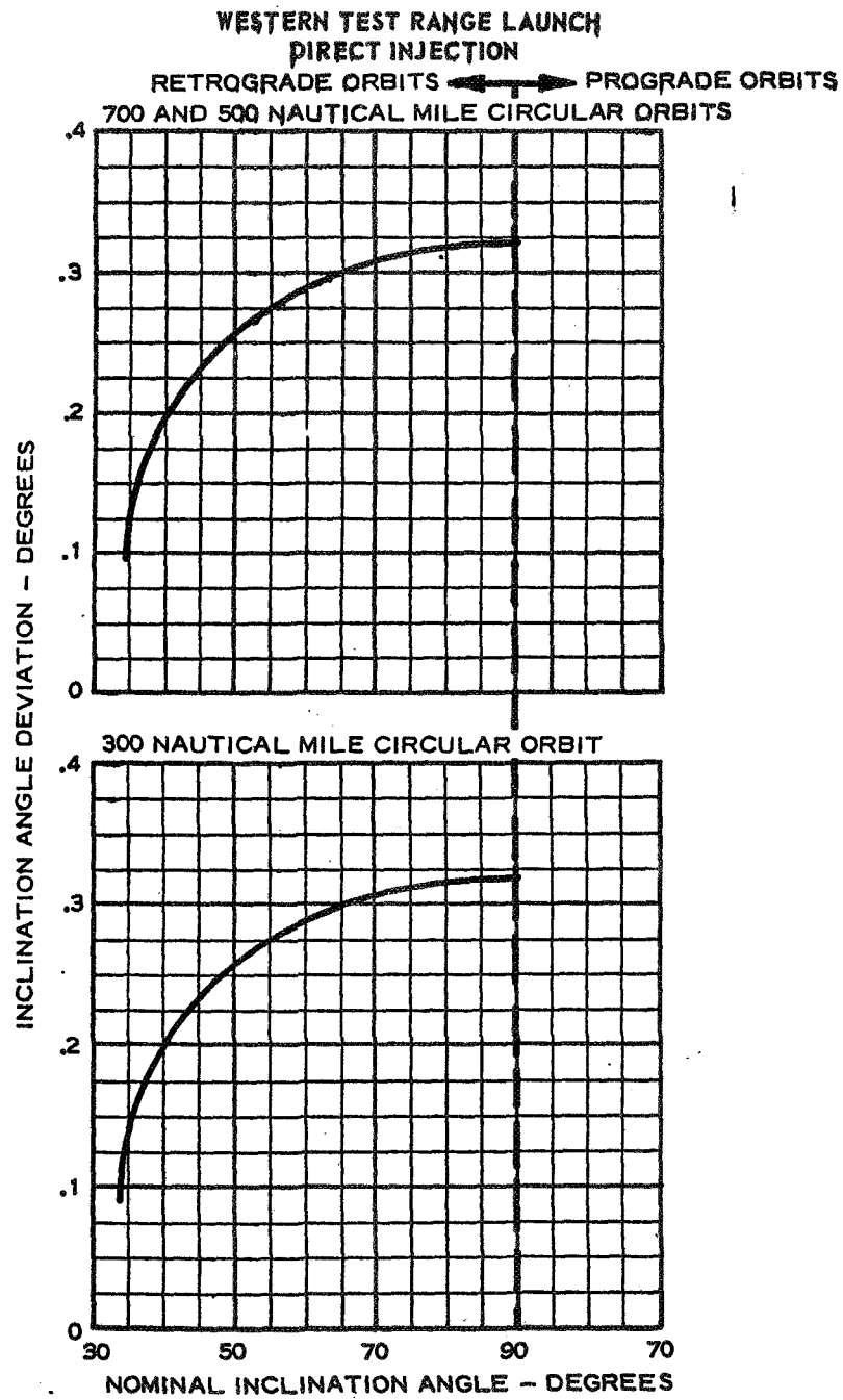
FIGURE 5-20. ONE-STANDARD DEVIATION IN INCLINATION ACCURACY - WTR
