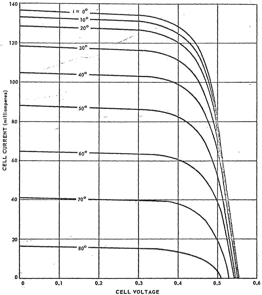
Fig. 2 TYPICAL SOLAR CELL CHARACTERISTICS AS A FUNCTION OF INCIDENCE ANGLE, CELL TEMPERATURE 25^\circ\text{C}
