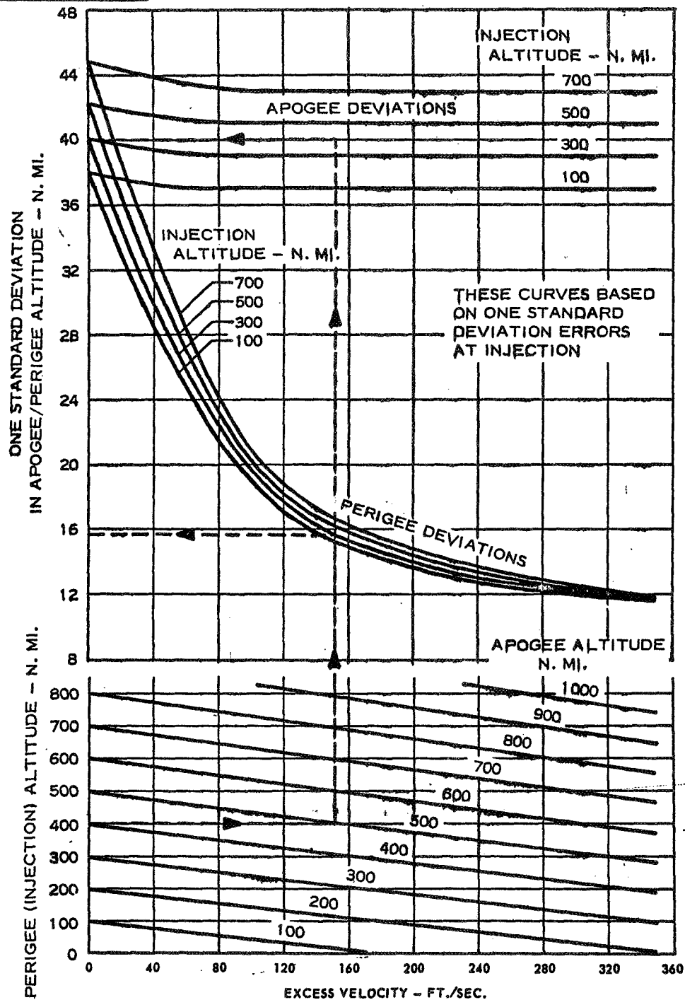
FIGURE 5-21. ORBIT ACCURACY (SHEET 1)
