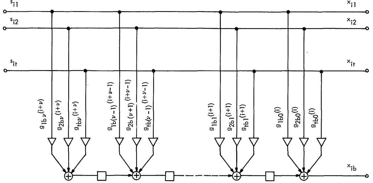
Fig. 11. High-rate systematic convolutional code encoder.
